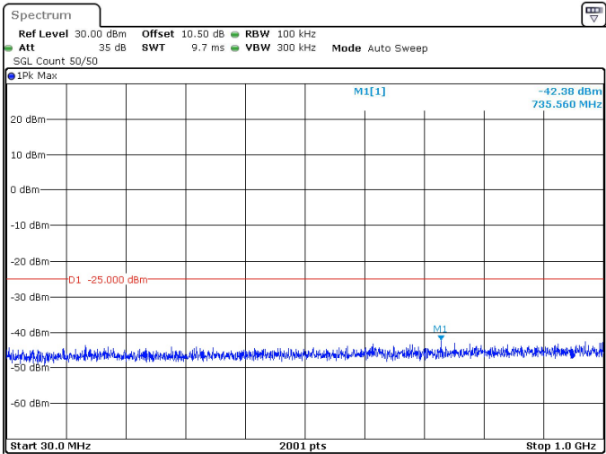
15MHz_30kHz_2612.5MHz_DFT-s-OFDM QPSK_RB1@0 -42.38 dBm
