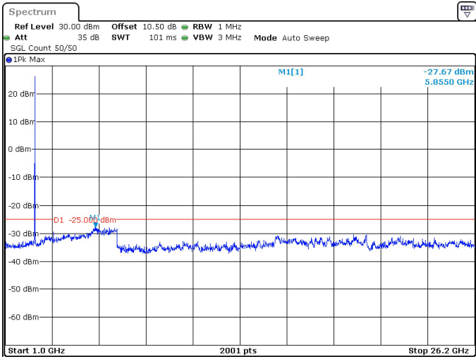
15MHz_30kHz_2595MHz_DFT-s-OFDM QPSK_RB1@0 -27.67 dBm
