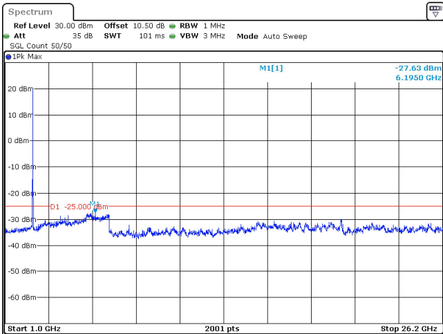
15MHz_30kHz_2595MHz_DFT-s-OFDM QPSK_RB36@0 -27.63 dBm
