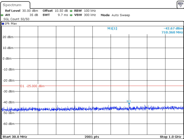
15MHz_30kHz_2577.5MHz_DFT-s-OFDM QPSK_RB36@0 -42.67 dBm
