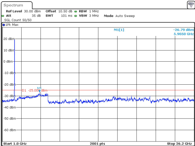
15MHz_30kHz_2612.5MHz_DFT-s-OFDM QPSK_RB36@0 -26.79 dBm
