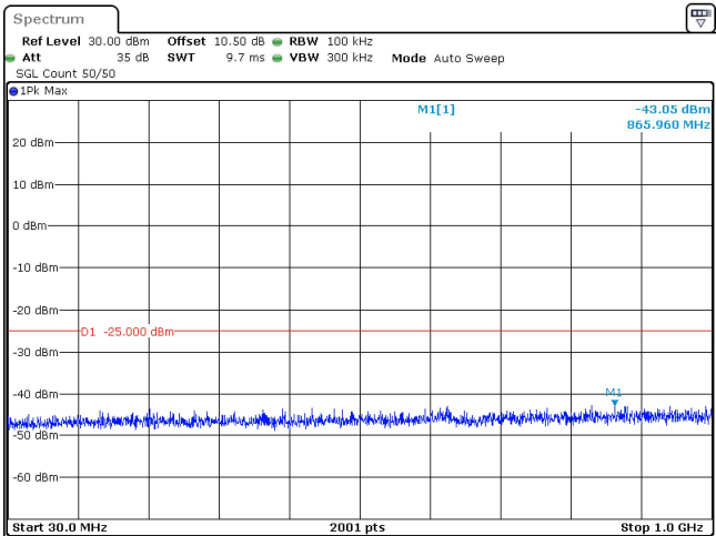
15MHz_30kHz_2612.5MHz_DFT-s-OFDM QPSK_RB36@0 -43.05 dBm
