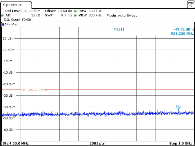
15MHz_30kHz_2577.5MHz_DFT-s-OFDM QPSK_RB1@37 -43.01 dBm
