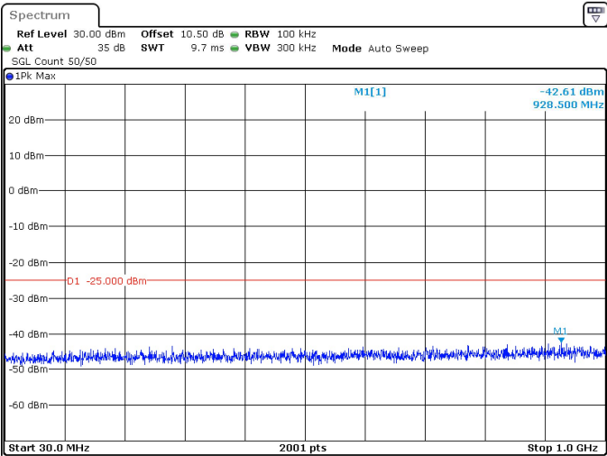
15MHz_30kHz_2577.5MHz_DFT-s-OFDM QPSK_RB1@0 -42.61 dBm
