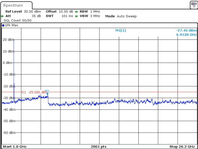
15MHz_30kHz_2577.5MHz_DFT-s-OFDM QPSK_RB36@0 -27.45 dBm
