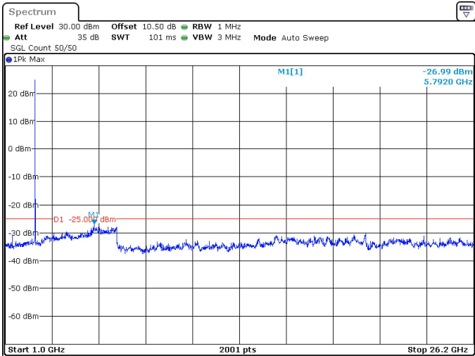
15MHz_30kHz_2612.5MHz_DFT-s-OFDM QPSK_RB1@0 -26.99 dBm
