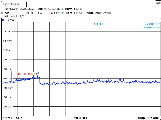
15MHz_30kHz_2595MHz_DFT-s-OFDM QPSK_RB1@37 -27.83 dBm
