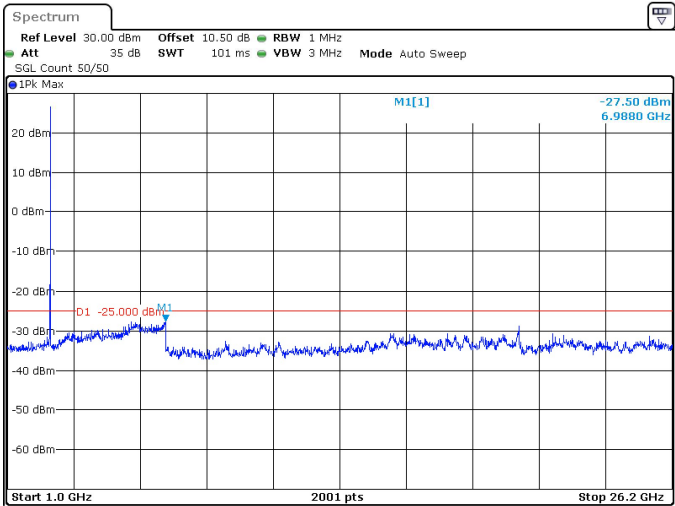
15MHz_30kHz_2612.5MHz_DFT-s-OFDM QPSK_RB1@37 -27.50 dBm
