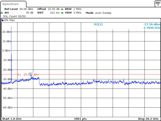
15MHz_30kHz_2577.5MHz_DFT-s-OFDM QPSK_RB1@37 -27.26 dBm
