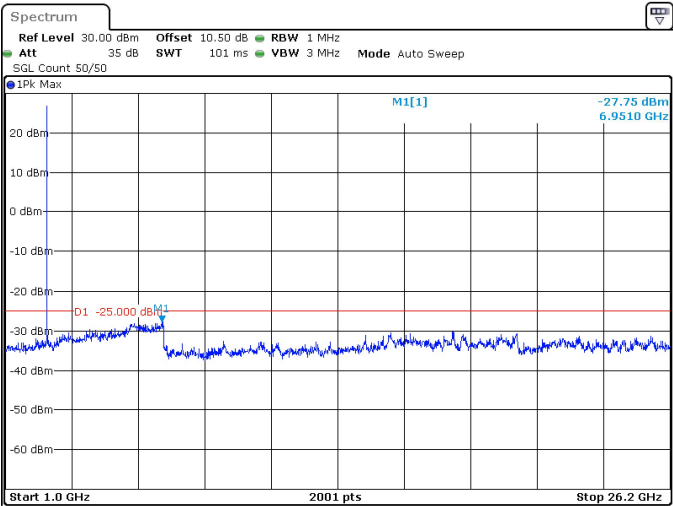
15MHz_30kHz_2577.5MHz_DFT-s-OFDM QPSK_RB1@0 -27.75 dBm
