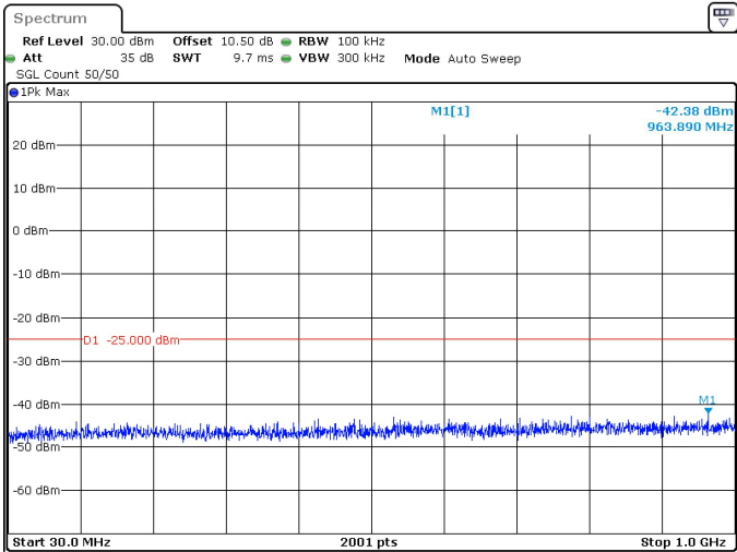
15MHz_30kHz_2612.5MHz_DFT-s-OFDM QPSK_RB1@37 -42.38 dBm
