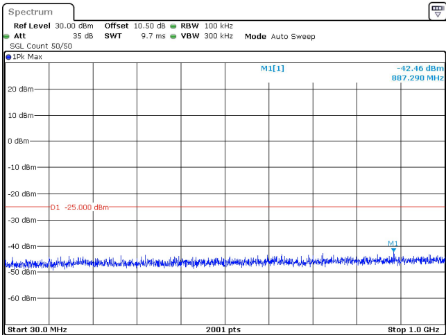
15MHz_30kHz_2595MHz_DFT-s-OFDM QPSK_RB36@0 -42.46 dBm
