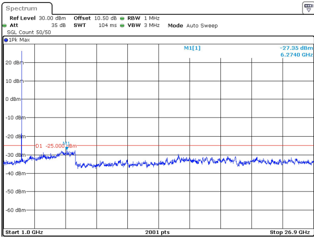
10MHz_30kHz_2501.01MHz_DFT-s-OFDM QPSK_RB1@23 -27.35 dBm
