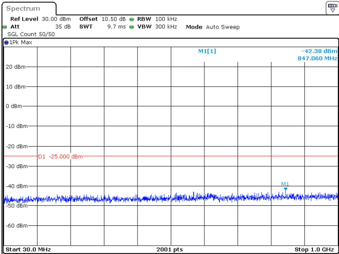
15MHz_30kHz_2503.5MHz_DFT-s-OFDM QPSK_RB1@37 -42.38 dBm
