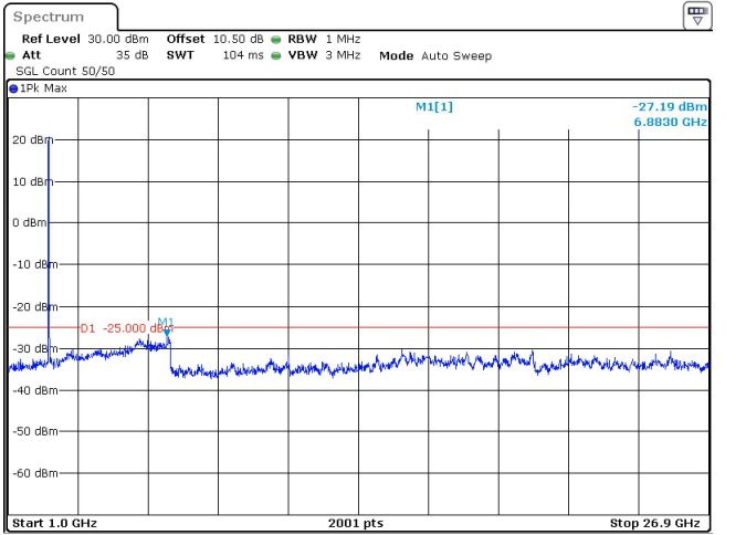
15MHz_30kHz_2503.5MHz_DFT-s-OFDM QPSK_RB36@0 -27.19 dBm
