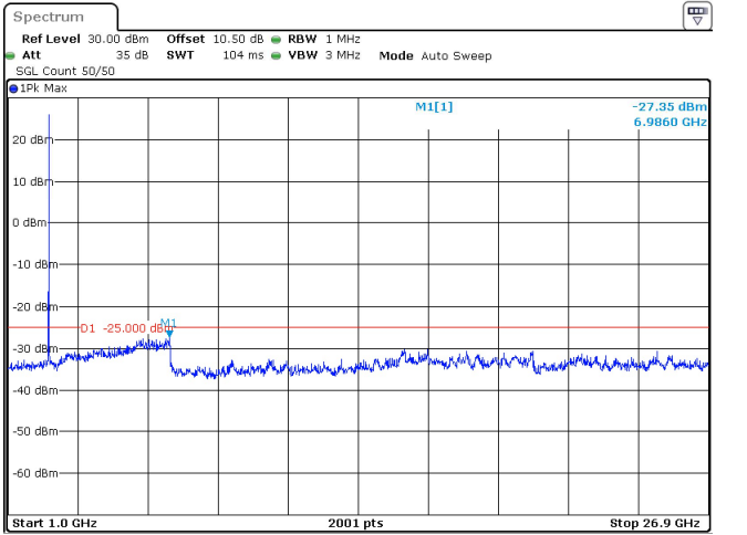
15MHz_30kHz_2503.5MHz_DFT-s-OFDM QPSK_RB1@37 -27.35 dBm
