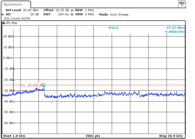
10MHz_30kHz_2592.99MHz_DFT-s-OFDM QPSK_RB1@23 -27.37 dBm
