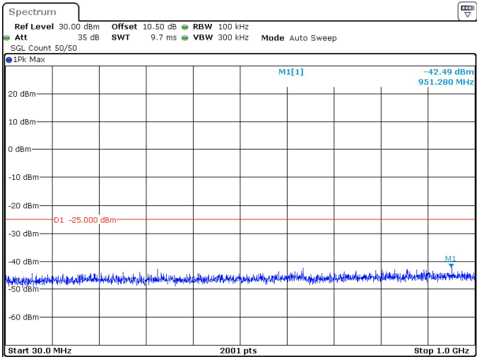
15MHz_30kHz_2503.5MHz_DFT-s-OFDM QPSK_RB1@0 -42.49 dBm
