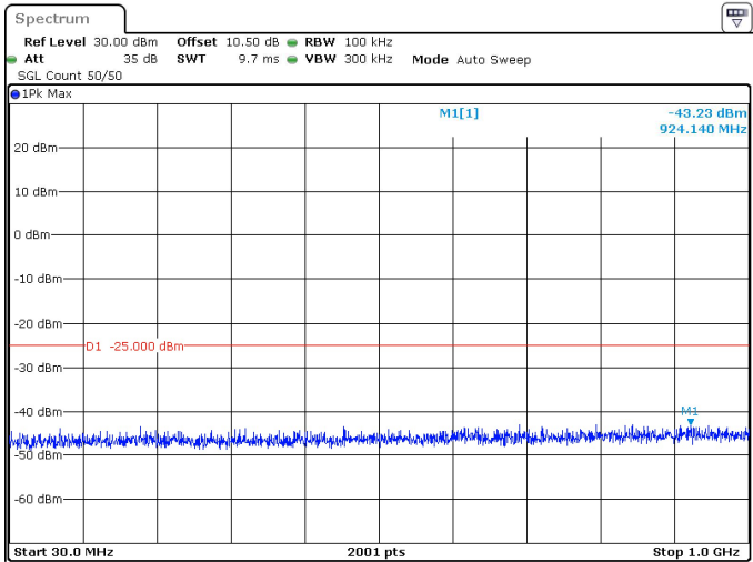
10MHz_30kHz_2592.99MHz_DFT-s-OFDM QPSK_RB1@23 -43.23 dBm
