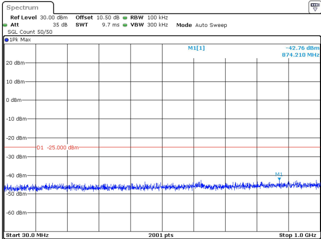
15MHz_30kHz_2682.48MHz_DFT-s-OFDM QPSK_RB36@0 -42.76 dBm
