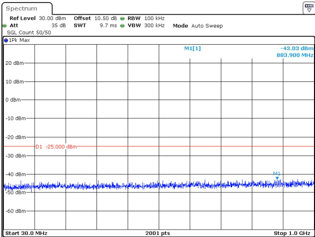
15MHz_30kHz_2592.99MHz_DFT-s-OFDM QPSK_RB36@0 -43.03 dBm
