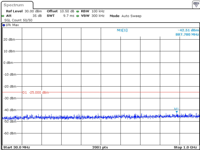
15MHz_30kHz_2592.99MHz_DFT-s-OFDM QPSK_RB1@37 -42.51 dBm
