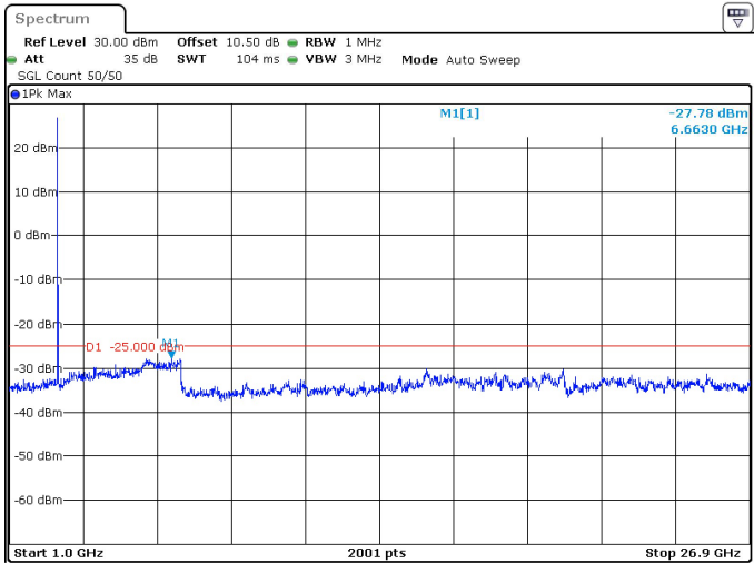
15MHz_30kHz_2682.48MHz_DFT-s-OFDM QPSK_RB1@37 -27.78 dBm
