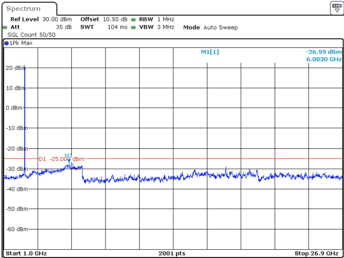
15MHz_30kHz_2592.99MHz_DFT-s-OFDM QPSK_RB36@0 -26.99 dBm
