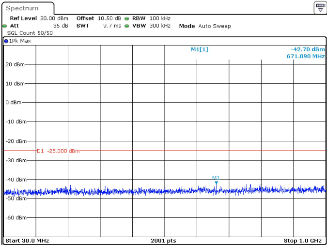
15MHz_30kHz_2592.99MHz_DFT-s-OFDM QPSK_RB1@0 -42.70 dBm
