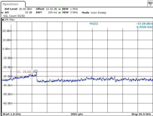
15MHz_30kHz_2592.99MHz_DFT-s-OFDM QPSK_RB1@37 -27.28 dBm
