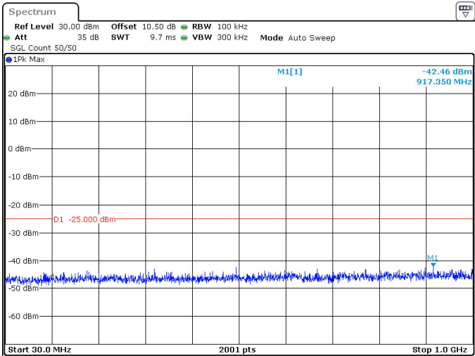
15MHz_30kHz_2503.5MHz_DFT-s-OFDM QPSK_RB36@0 -42.46 dBm
