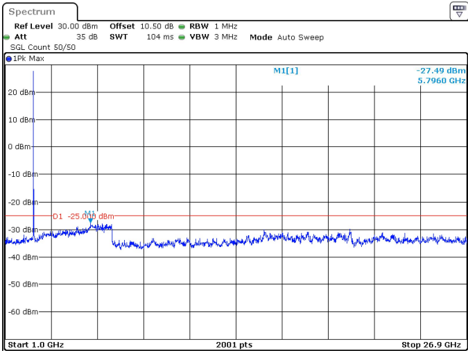
15MHz_30kHz_2592.99MHz_DFT-s-OFDM QPSK_RB1@0 -27.49 dBm
