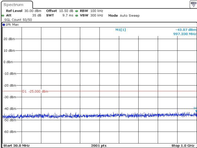
15MHz_30kHz_2682.48MHz_DFT-s-OFDM QPSK_RB1@37 -43.07 dBm
