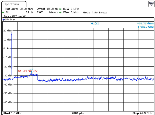
40MHz_30kHz_2516.01MHz_DFT-s-OFDM QPSK_RB100@0 -26.73 dBm
