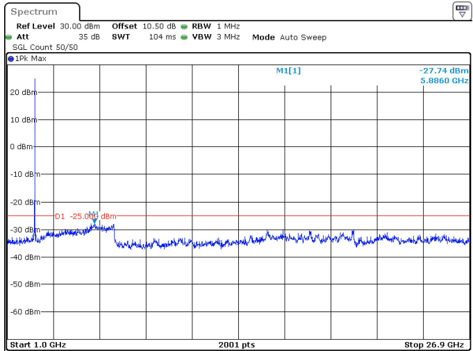
40MHz_30kHz_2516.01MHz_DFT-s-OFDM QPSK_RB1@105 -27.74 dBm
