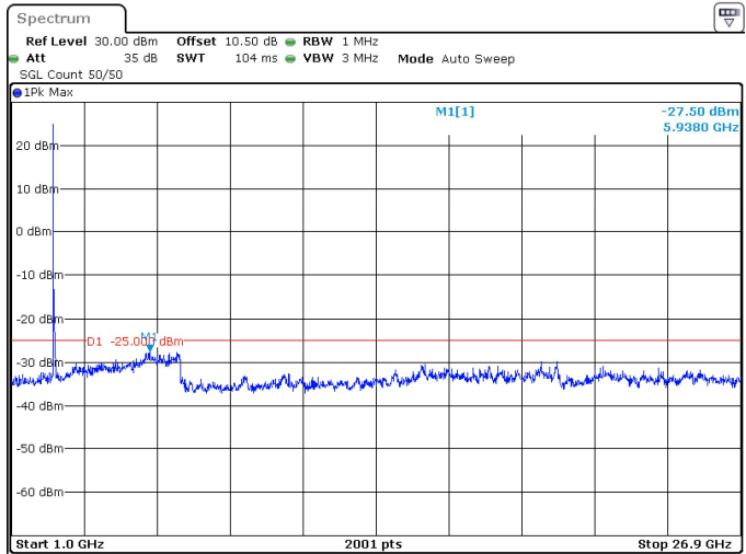
40MHz_30kHz_2516.01MHz_DFT-s-OFDM QPSK_RB1@0 -27.50 dBm
