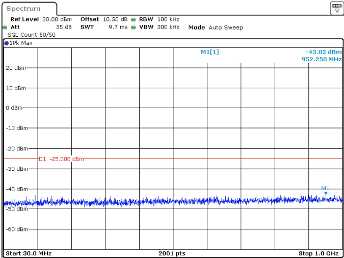
40MHz_30kHz_2516.01MHz_DFT-s-OFDM QPSK_RB1@0 -43.02 dBm
