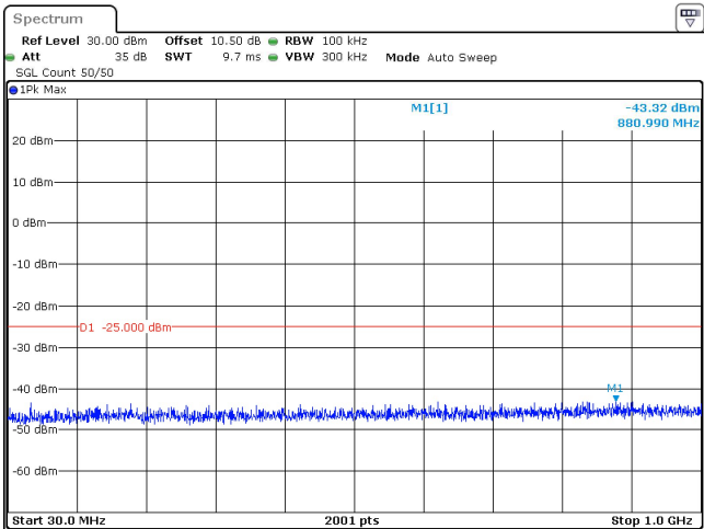
40MHz_30kHz_2516.01MHz_DFT-s-OFDM QPSK_RB1@105 -43.32 dBm
