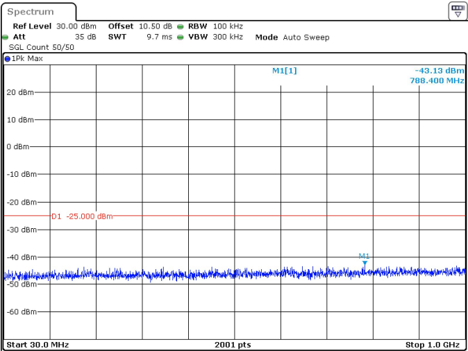
50MHz_30kHz_2592.99MHz_DFT-s-OFDM QPSK_RB1@0 -43.13 dBm
