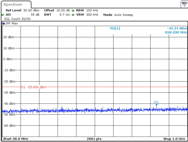
50MHz_30kHz_2592.99MHz_DFT-s-OFDM QPSK_RB128@0 -42.21 dBm
