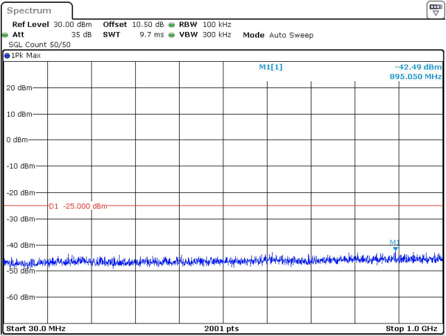
50MHz_30kHz_2592.99MHz_DFT-s-OFDM QPSK_RB1@132 -42.49 dBm
