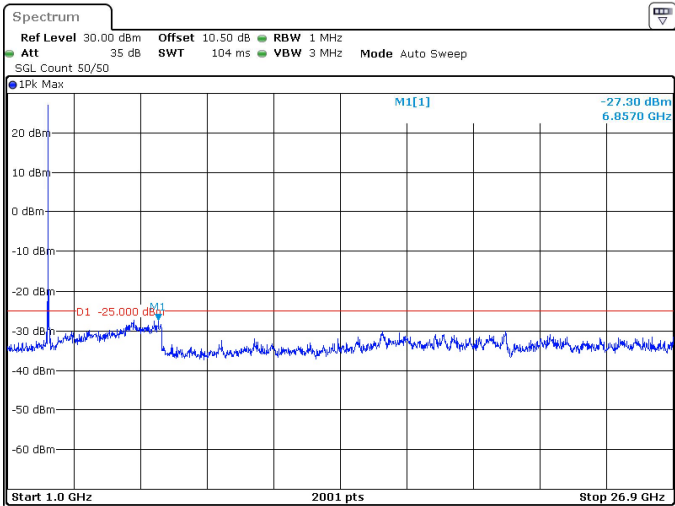
50MHz_30kHz_2592.99MHz_DFT-s-OFDM QPSK_RB1@0 -27.30 dBm
