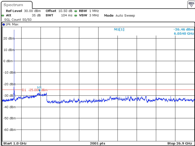
50MHz_30kHz_2592.99MHz_DFT-s-OFDM QPSK_RB1@132 -26.46 dBm
