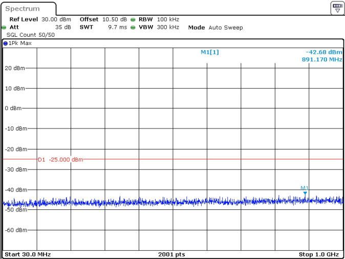
50MHz_30kHz_2521.02MHz_DFT-s-OFDM QPSK_RB128@0 -42.68 dBm
