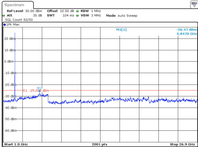
80MHz_30kHz_2536.02MHz_DFT-s-OFDM QPSK_RB1@216 -26.47 dBm
