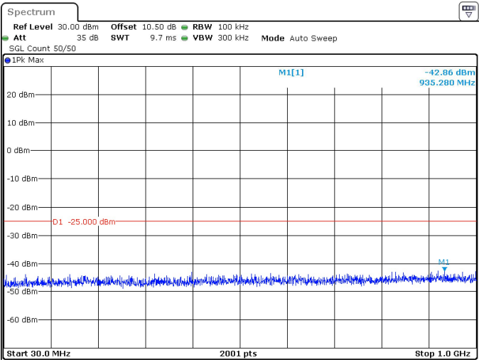
60MHz_30kHz_2592.99MHz_DFT-s-OFDM QPSK_RB162@0 -42.86 dBm
