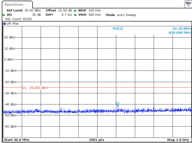
80MHz_30kHz_2536.02MHz_DFT-s-OFDM QPSK_RB216@0 -42.18 dBm
