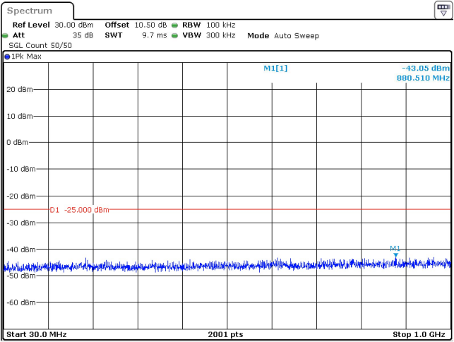
80MHz_30kHz_2536.02MHz_DFT-s-OFDM QPSK_RB1@216 -43.05 dBm
