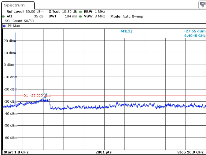
60MHz_30kHz_2592.99MHz_DFT-s-OFDM QPSK_RB1@161 -27.65 dBm
