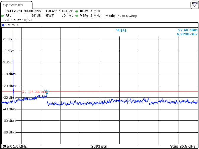
80MHz_30kHz_2536.02MHz_DFT-s-OFDM QPSK_RB1@0 -27.58 dBm
