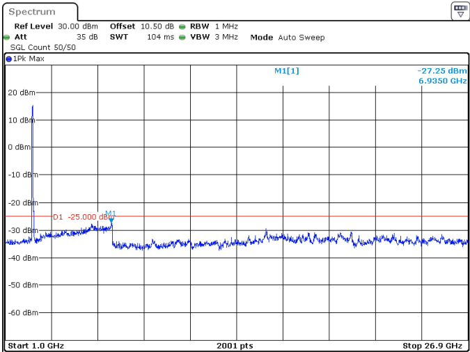
60MHz_30kHz_2526MHz_DFT-s-OFDM QPSK_RB162@0 -27.25 dBm
