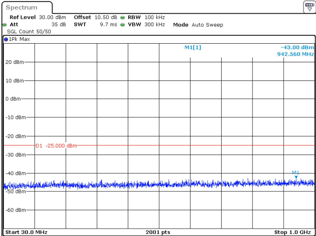
60MHz_30kHz_2592.99MHz_DFT-s-OFDM QPSK_RB1@161 -43.00 dBm
