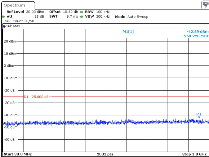
60MHz_30kHz_2592.99MHz_DFT-s-OFDM QPSK_RB1@0 -42.89 dBm
