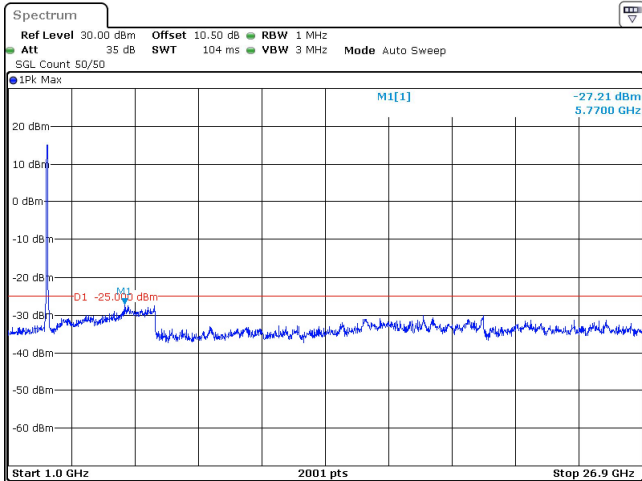
60MHz_30kHz_2592.99MHz_DFT-s-OFDM QPSK_RB162@0 -27.21 dBm
