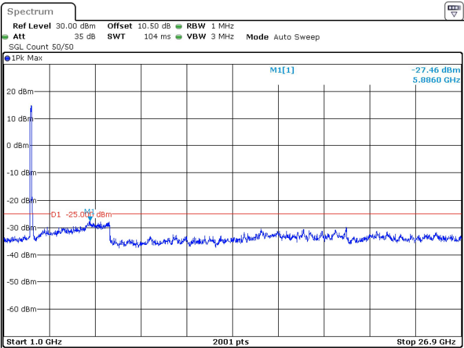
80MHz_30kHz_2536.02MHz_DFT-s-OFDM QPSK_RB216@0 -27.46 dBm
