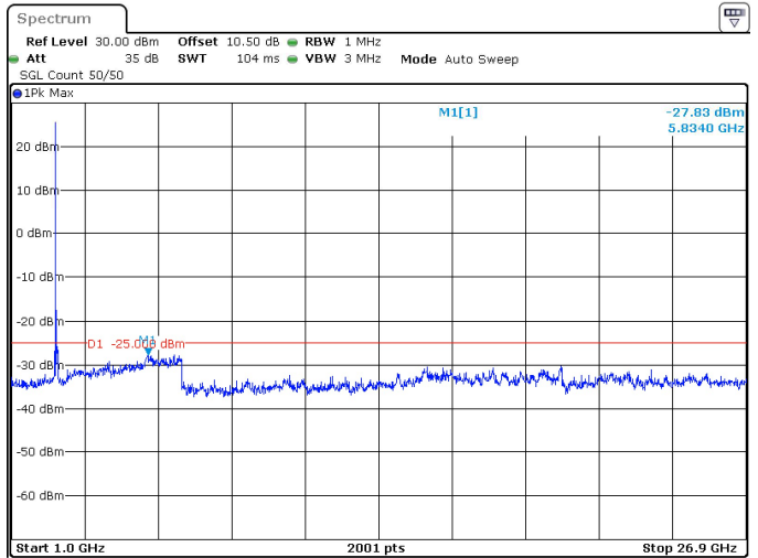
80MHz_30kHz_2592.99MHz_DFT-s-OFDM QPSK_RB1@0 -27.83 dBm
