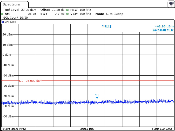
80MHz_30kHz_2592.99MHz_DFT-s-OFDM QPSK_RB216@0 -42.93 dBm
