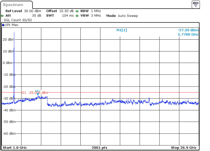
80MHz_30kHz_2592.99MHz_DFT-s-OFDM QPSK_RB1@216 -27.39 dBm
