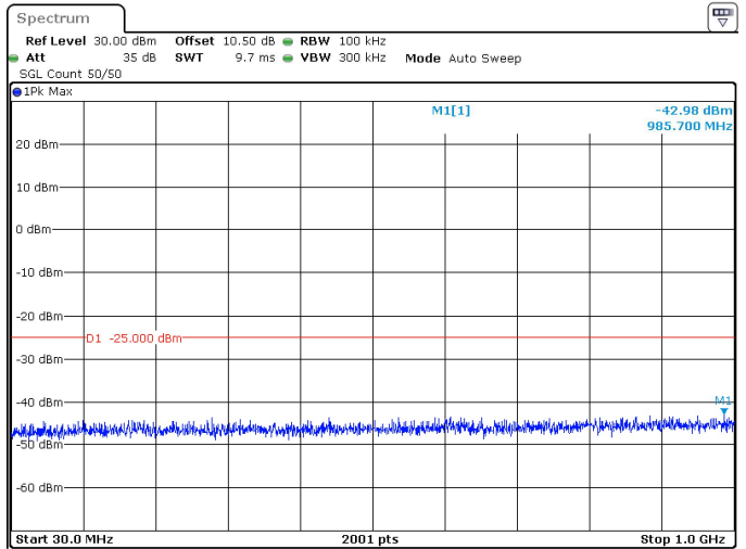
80MHz_30kHz_2592.99MHz_DFT-s-OFDM QPSK_RB1@216 -42.98 dBm
