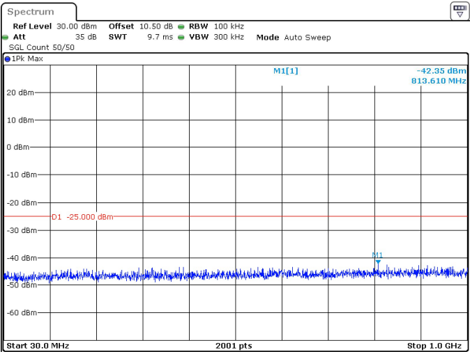
80MHz_30kHz_2592.99MHz_DFT-s-OFDM QPSK_RB1@0 -42.35 dBm
