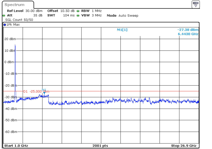
80MHz_30kHz_2592.99MHz_DFT-s-OFDM QPSK_RB216@0 -27.38 dBm
