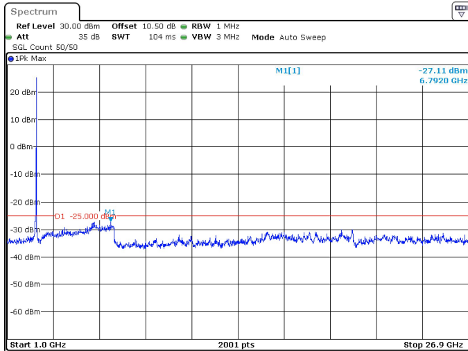
90MHz_30kHz_2592.99MHz_DFT-s-OFDM QPSK_RB1@244 -27.11 dBm
