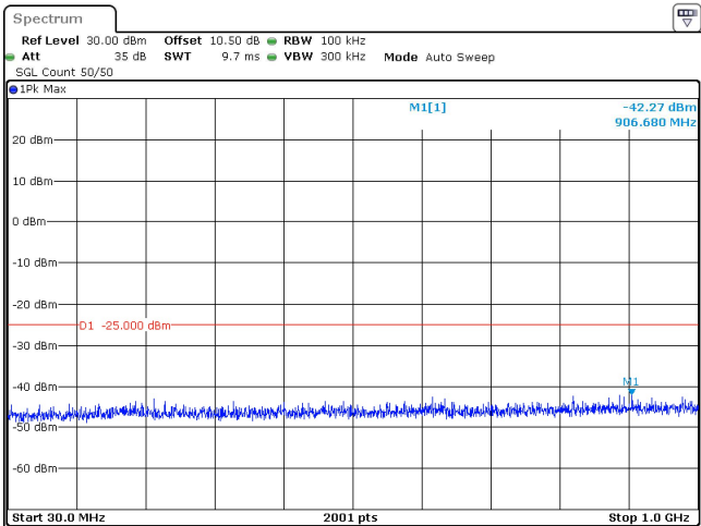
90MHz_30kHz_2592.99MHz_DFT-s-OFDM QPSK_RB1@244 -42.27 dBm
