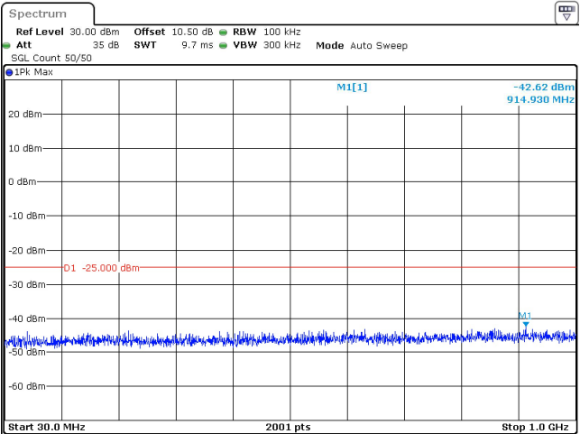
100MHz_30kHz_2546.01MHz_DFT-s-OFDM QPSK_RB1@272 -42.62 dBm
