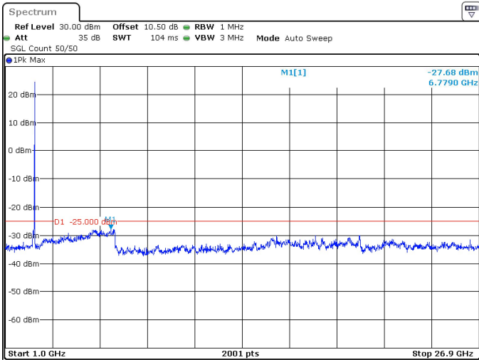
100MHz_30kHz_2546.01MHz_DFT-s-OFDM QPSK_RB1@272 -27.68 dBm
