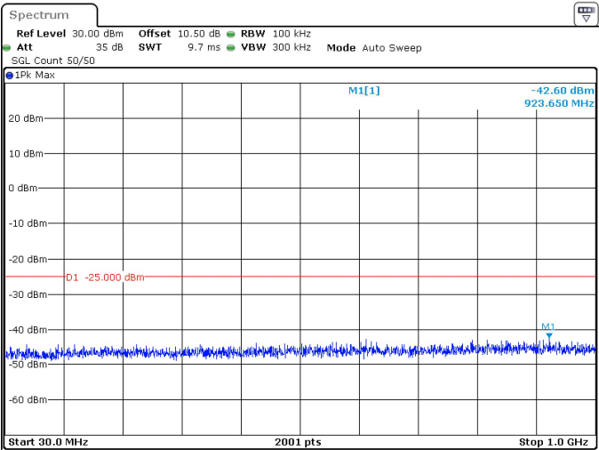
100MHz_30kHz_2546.01MHz_DFT-s-OFDM QPSK_RB1@0 -42.60 dBm
