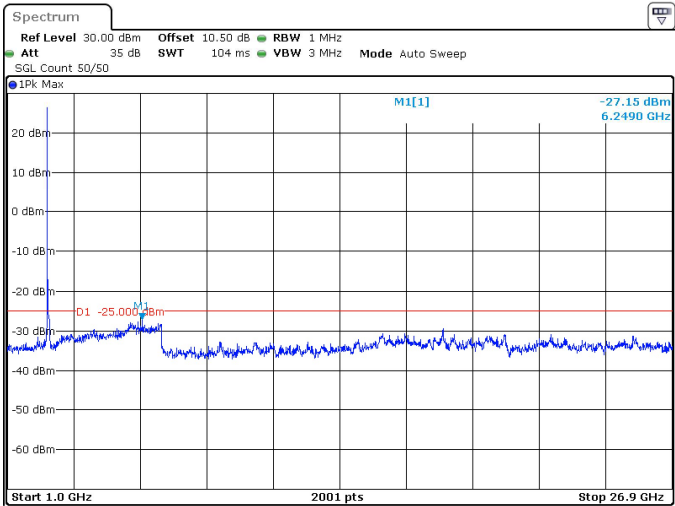
90MHz_30kHz_2592.99MHz_DFT-s-OFDM QPSK_RB1@0 -27.15 dBm
