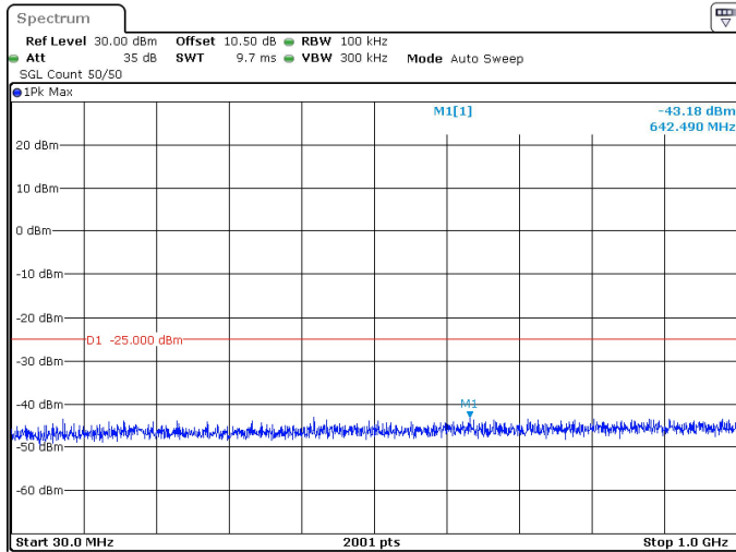
90MHz_30kHz_2592.99MHz_DFT-s-OFDM QPSK_RB1@0 -43.18 dBm
