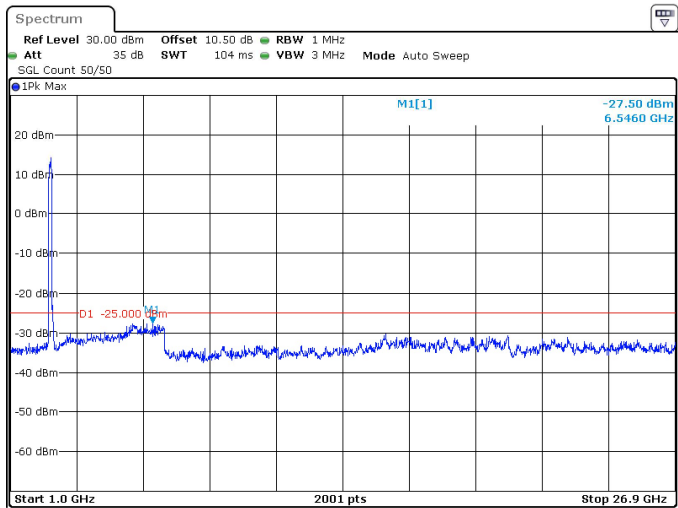
100MHz_30kHz_2546.01MHz_DFT-s-OFDM QPSK_RB270@0 -27.50 dBm
