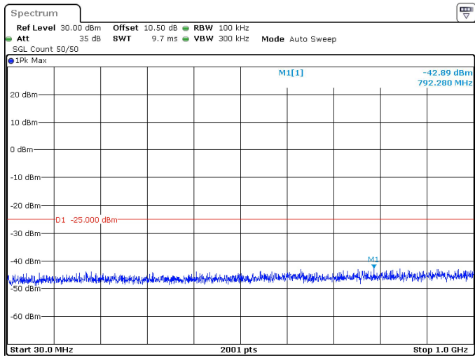
100MHz_30kHz_2592.99MHz_DFT-s-OFDM QPSK_RB1@272 -42.89 dBm
