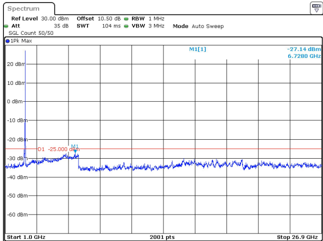
100MHz_30kHz_2592.99MHz_DFT-s-OFDM QPSK_RB1@272 -27.14 dBm
