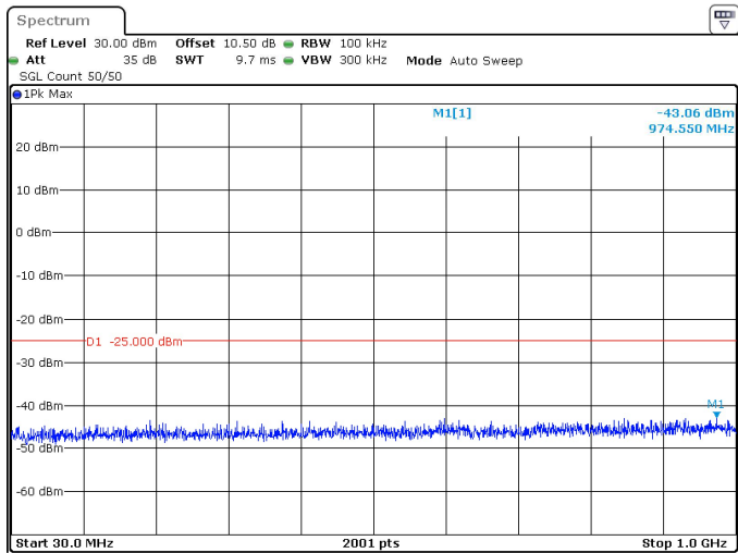
100MHz_30kHz_2592.99MHz_DFT-s-OFDM QPSK_RB1@0 -43.06 dBm
