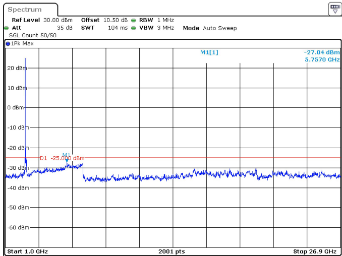
100MHz_30kHz_2592.99MHz_DFT-s-OFDM QPSK_RB1@0 -27.04 dBm
