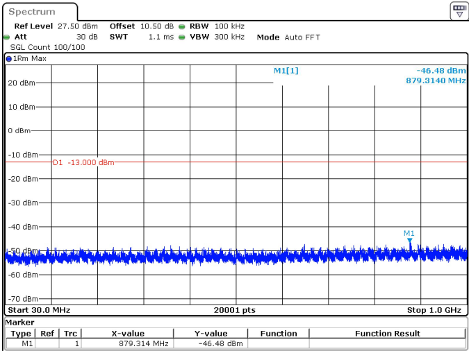
40MHz_15kHz_1730MHz_DFT-s-OFDM QPSK_RB1@0 -46.48 dBm
