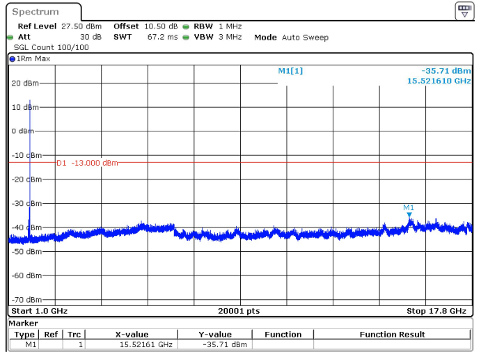
30MHz_15kHz_1745MHz_DFT-s-OFDM QPSK_RB1@159 -35.71 dBm
