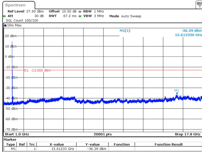
40MHz_15kHz_1730MHz_DFT-s-OFDM QPSK_RB1@0 -36.39 dBm
