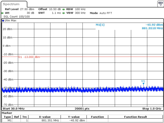
30MHz_15kHz_1765MHz_DFT-s-OFDM QPSK_RB160@0 -45.92 dBm
