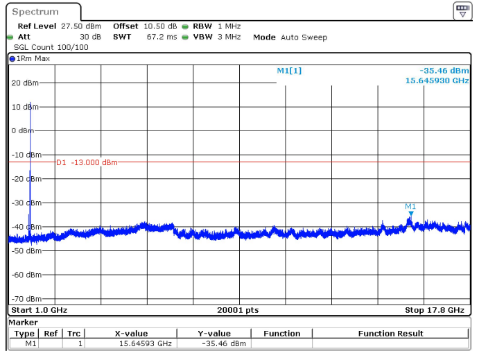
30MHz_15kHz_1765MHz_DFT-s-OFDM QPSK_RB1@159 -35.46 dBm
