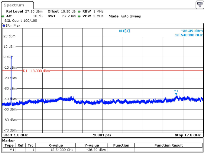
30MHz_15kHz_1745MHz_DFT-s-OFDM QPSK_RB160@0 -36.39 dBm
