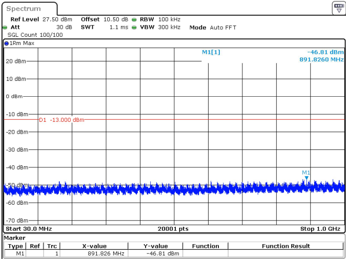
30MHz_15kHz_1745MHz_DFT-s-OFDM QPSK_RB1@0 -46.81 dBm
