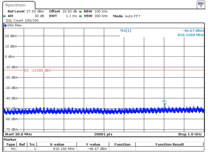
30MHz_15kHz_1765MHz_DFT-s-OFDM QPSK_RB1@0 -46.67 dBm
