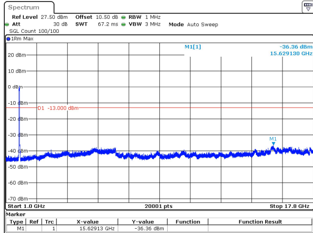
40MHz_15kHz_1730MHz_DFT-s-OFDM QPSK_RB216@0 -36.36 dBm
