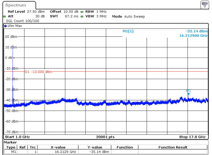
30MHz_15kHz_1745MHz_DFT-s-OFDM QPSK_RB1@0 -35.14 dBm
