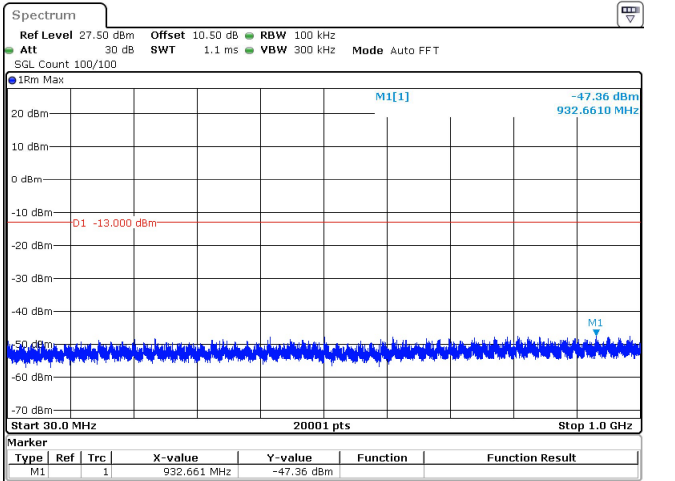
30MHz_15kHz_1765MHz_DFT-s-OFDM QPSK_RB1@159 -47.36 dBm
