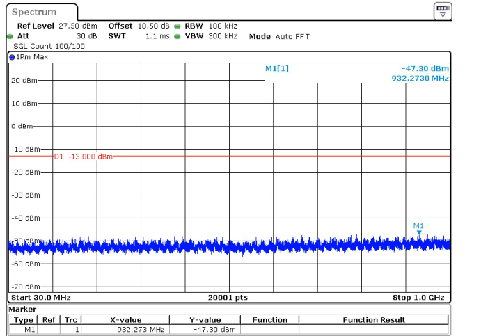
30MHz_15kHz_1745MHz_DFT-s-OFDM QPSK_RB160@0 -47.30 dBm
