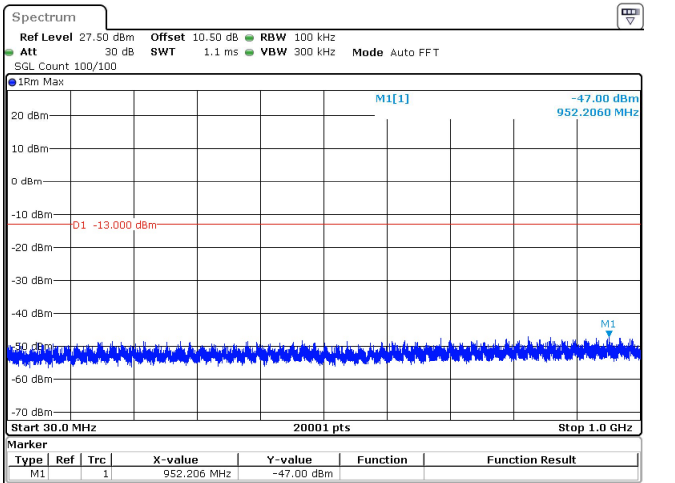
30MHz_15kHz_1745MHz_DFT-s-OFDM QPSK_RB1@159 -47.00 dBm
