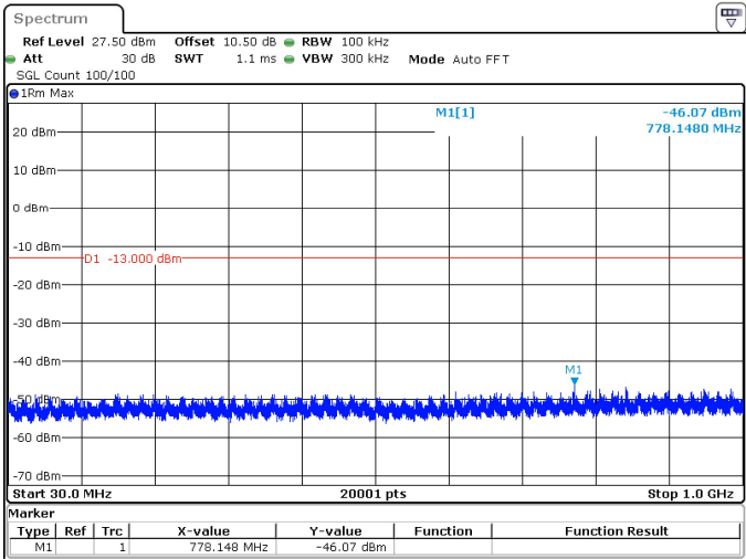
30MHz_15kHz_1725MHz_DFT-s-OFDM QPSK_RB160@0 -46.07 dBm
