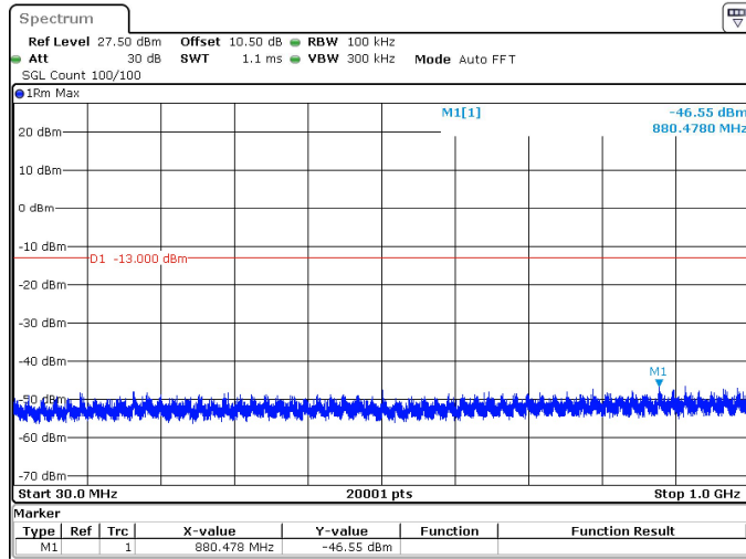
40MHz_15kHz_1730MHz_DFT-s-OFDM QPSK_RB1@215 -46.55 dBm
