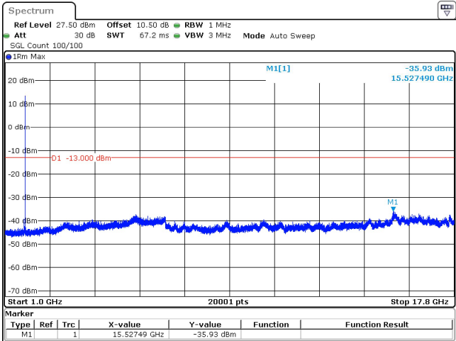
40MHz_15kHz_1730MHz_DFT-s-OFDM QPSK_RB1@215 -35.93 dBm
