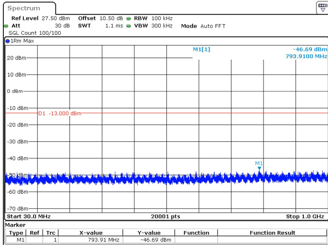
40MHz_15kHz_1760MHz_DFT-s-OFDM QPSK_RB1@0 -46.69 dBm
