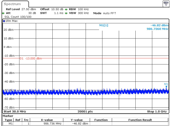
40MHz_15kHz_1760MHz_DFT-s-OFDM QPSK_RB216@0 -46.82 dBm
