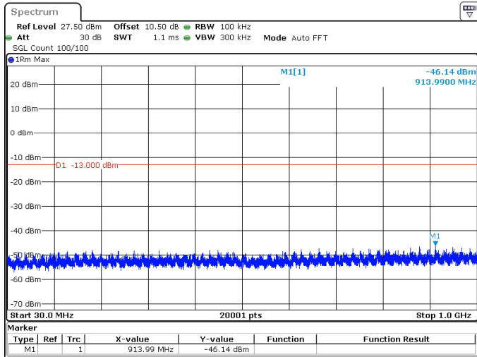
40MHz_15kHz_1760MHz_DFT-s-OFDM QPSK_RB1@215 -46.14 dBm
