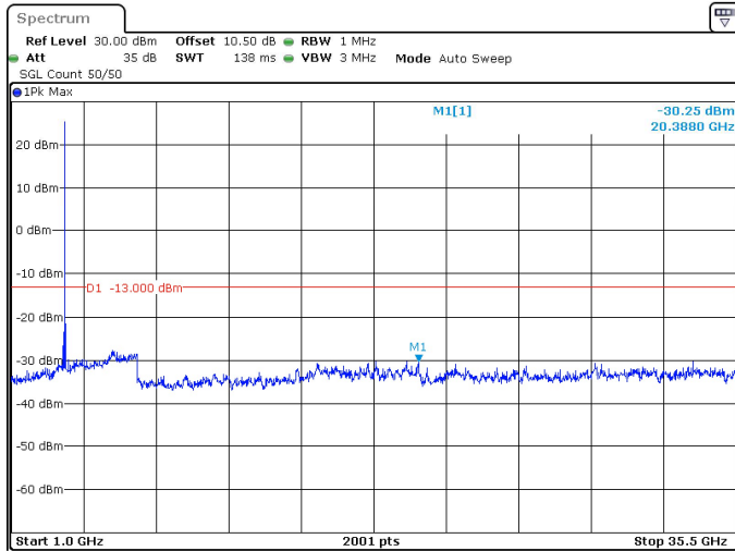
10MHz_15kHz_3545MHz_DFT-s-OFDM QPSK_RB1@0 -30.25 dBm
