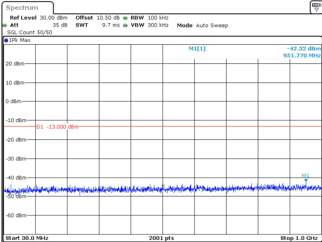
10MHz_15kHz_3500MHz_DFT-s-OFDM QPSK_RB1@51 -42.32 dBm
