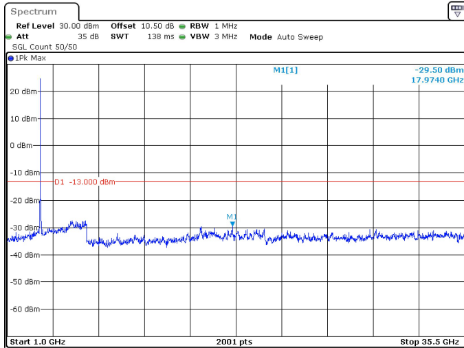
10MHz_15kHz_3500MHz_DFT-s-OFDM QPSK_RB1@51 -29.50 dBm
