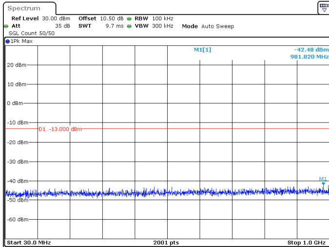
10MHz_15kHz_3545MHz_DFT-s-OFDM QPSK_RB1@51 -42.48 dBm
