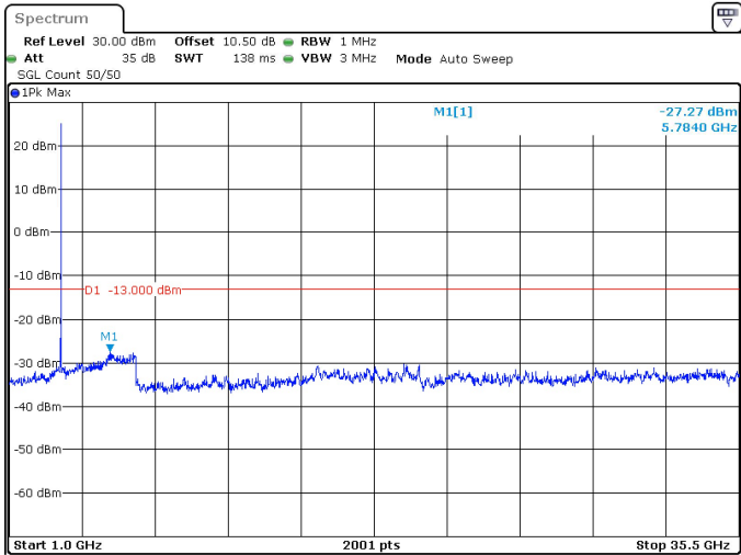
15MHz_15kHz_3457.5MHz_DFT-s-OFDM QPSK_RB1@0 -27.27 dBm
