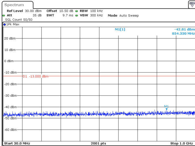
10MHz_30kHz_3545MHz_DFT-s-OFDM QPSK_RB1@0 -42.81 dBm
