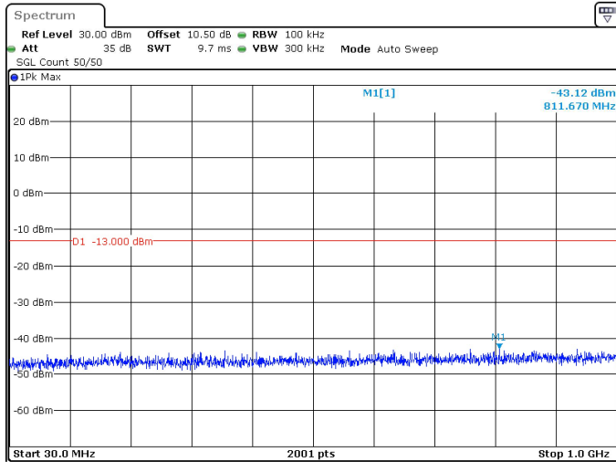
10MHz_30kHz_3545MHz_DFT-s-OFDM QPSK_RB1@23 -43.12 dBm
