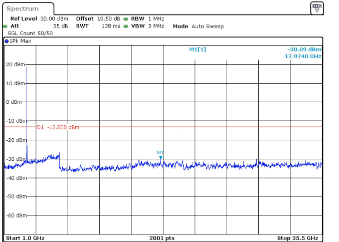
15MHz_15kHz_3457.5MHz_DFT-s-OFDM QPSK_RB75@0 -30.09 dBm
