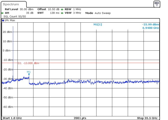
15MHz_15kHz_3457.5MHz_DFT-s-OFDM QPSK_RB1@78 -25.99 dBm
