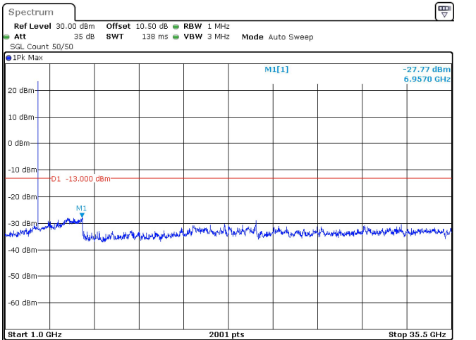
10MHz_30kHz_3545MHz_DFT-s-OFDM QPSK_RB1@23 -27.77 dBm
