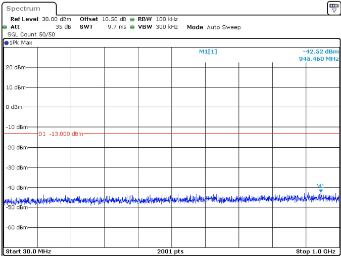
15MHz_15kHz_3457.5MHz_DFT-s-OFDM QPSK_RB1@0 -42.52 dBm
