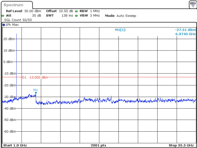
10MHz_30kHz_3545MHz_DFT-s-OFDM QPSK_RB1@0 -27.51 dBm
