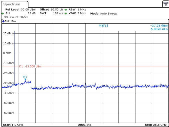
15MHz_30kHz_3542.5MHz_DFT-s-OFDM QPSK_RB1@0 -27.21 dBm
