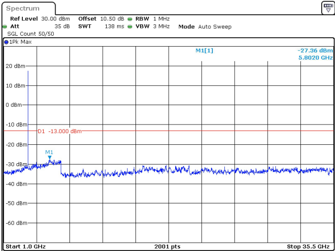
15MHz_30kHz_3542.5MHz_DFT-s-OFDM QPSK_RB36@0 -27.36 dBm
