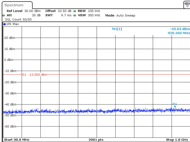
15MHz_30kHz_3500MHz_DFT-s-OFDM QPSK_RB36@0 -43.04 dBm
