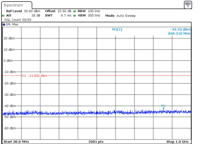
15MHz_30kHz_3542.5MHz_DFT-s-OFDM QPSK_RB36@0 -43.23 dBm
