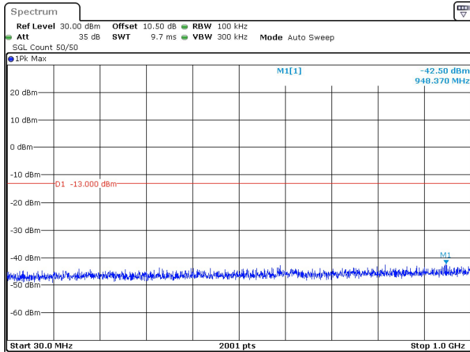
15MHz_30kHz_3500MHz_DFT-s-OFDM QPSK_RB1@0 -42.50 dBm
