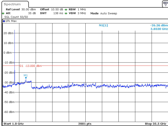
15MHz_30kHz_3500MHz_DFT-s-OFDM QPSK_RB1@37 -26.36 dBm
