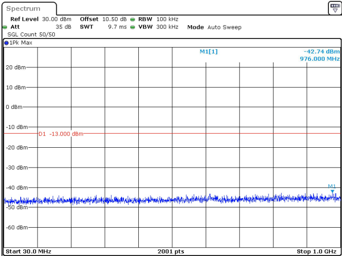
15MHz_30kHz_3542.5MHz_DFT-s-OFDM QPSK_RB1@0 -42.74 dBm
