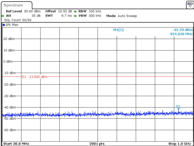
15MHz_30kHz_3500MHz_DFT-s-OFDM QPSK_RB1@37 -42.29 dBm
