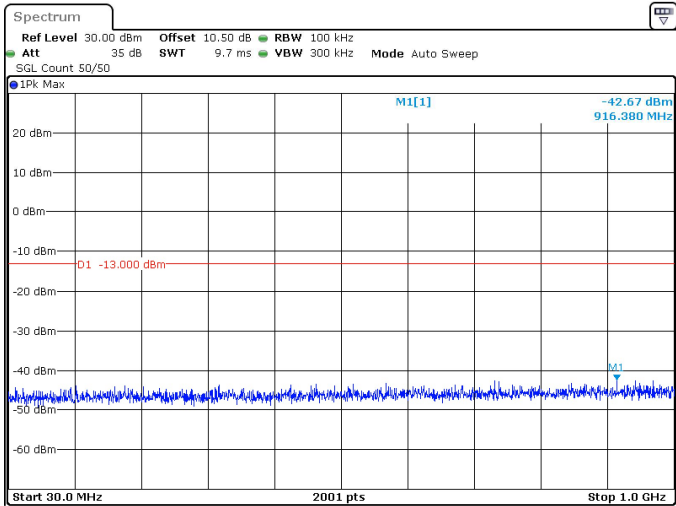
15MHz_30kHz_3542.5MHz_DFT-s-OFDM QPSK_RB1@37 -42.67 dBm
