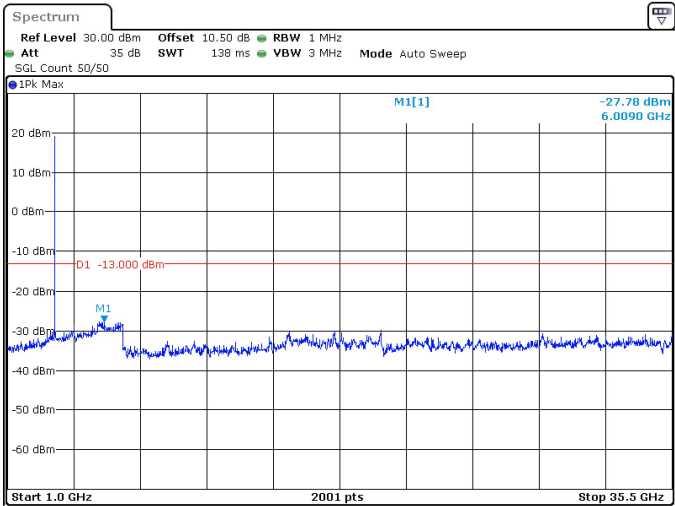
15MHz_30kHz_3457.5MHz_DFT-s-OFDM QPSK_RB36@0 -27.78 dBm
