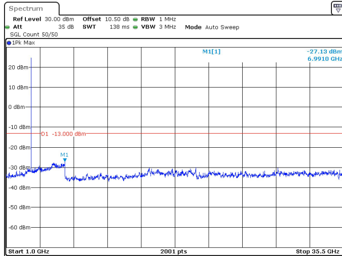
20MHz_15kHz_3540MHz_DFT-s-OFDM QPSK_RB1@105 -27.13 dBm
