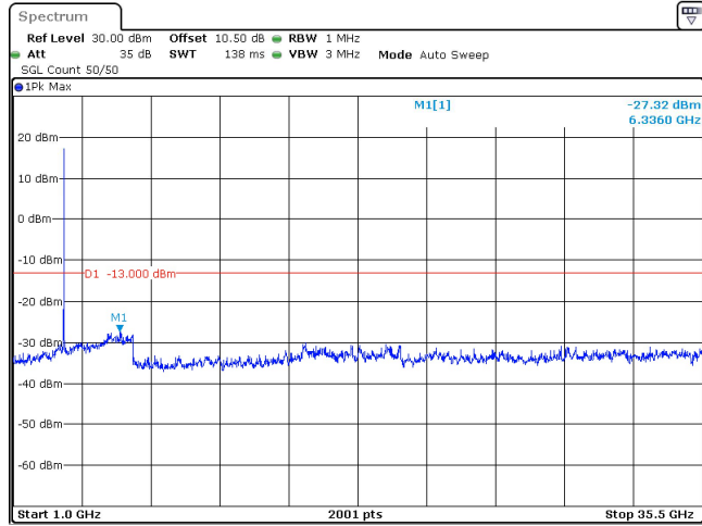
20MHz_15kHz_3540MHz_DFT-s-OFDM QPSK_RB100@0 -27.32 dBm
