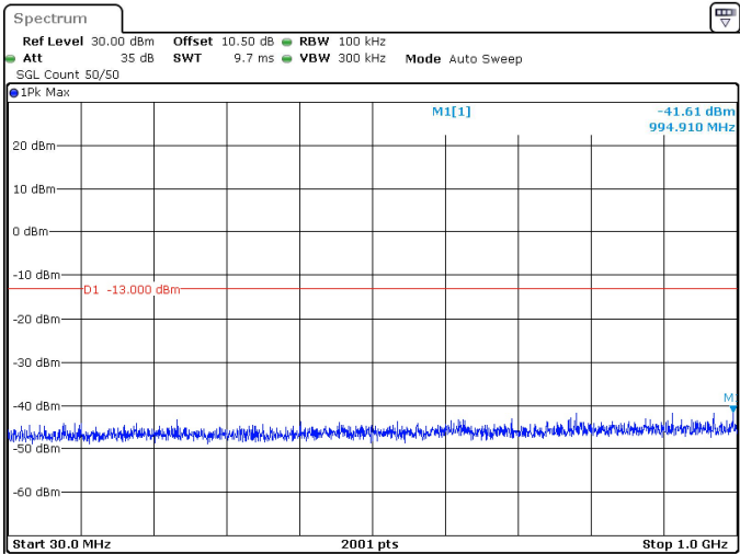
20MHz_15kHz_3540MHz_DFT-s-OFDM QPSK_RB100@0 -41.61 dBm
