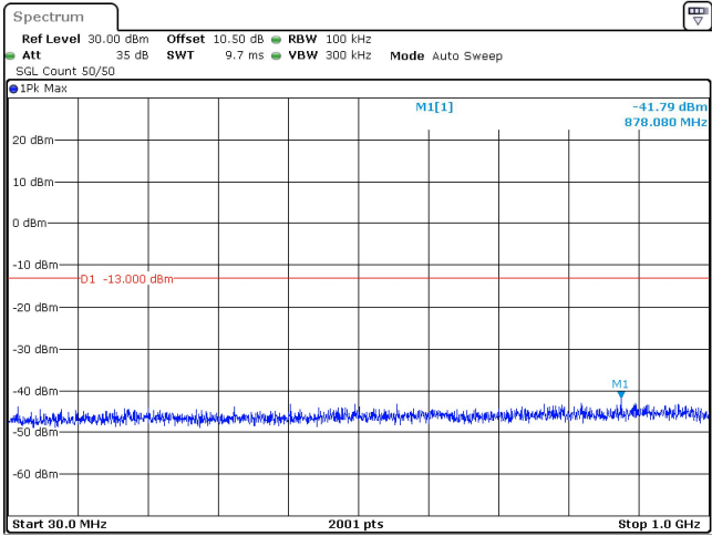
20MHz_15kHz_3540MHz_DFT-s-OFDM QPSK_RB1@105 -41.79 dBm
