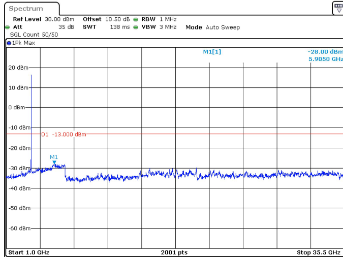
20MHz_15kHz_3540MHz_DFT-s-OFDM QPSK_RB1@0 -28.00 dBm
