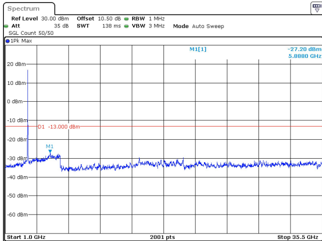
30MHz_15kHz_3465MHz_DFT-s-OFDM QPSK_RB160@0 -27.20 dBm
