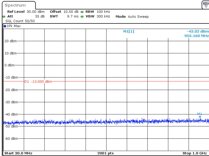
30MHz_15kHz_3465MHz_DFT-s-OFDM QPSK_RB1@159 -43.02 dBm
