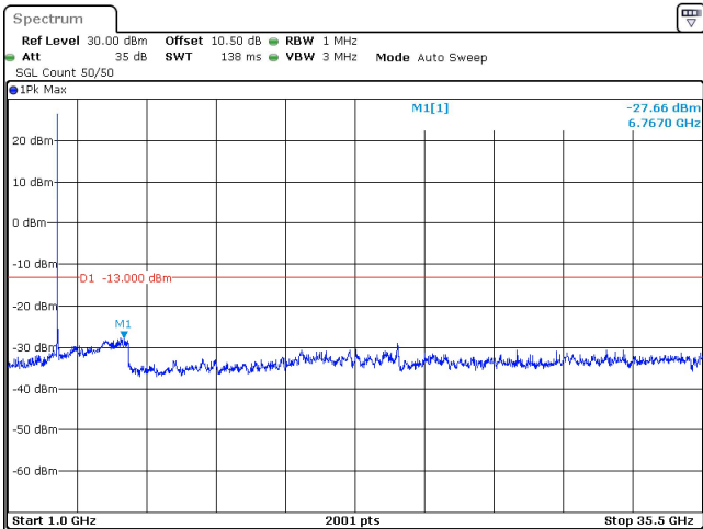
30MHz_15kHz_3465MHz_DFT-s-OFDM QPSK_RB1@159 -27.66 dBm
