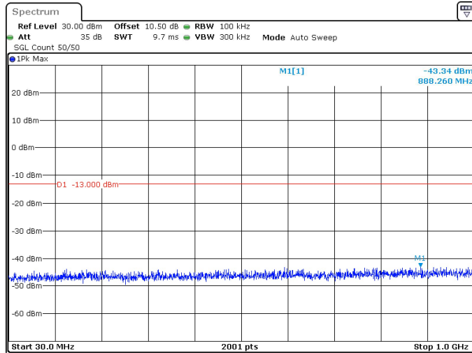
50MHz_15kHz_3500MHz_DFT-s-OFDM QPSK_RB1@269 -43.34 dBm
