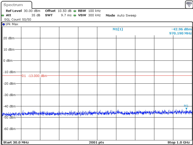
50MHz_15kHz_3500MHz_DFT-s-OFDM QPSK_RB1@0 -42.96 dBm
