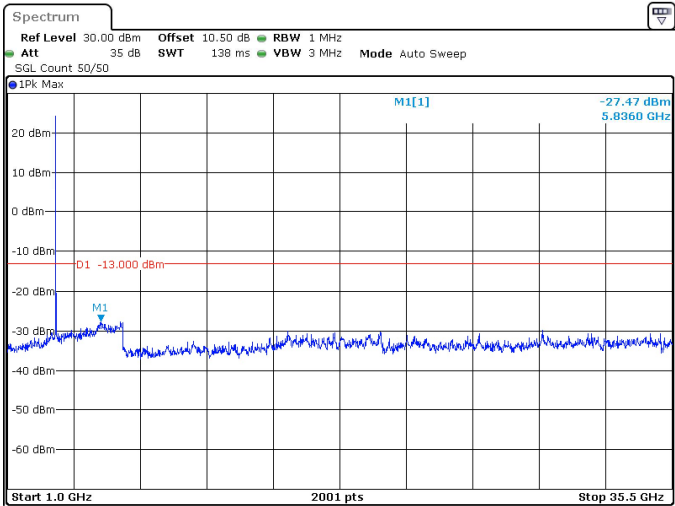
50MHz_15kHz_3525MHz_DFT-s-OFDM QPSK_RB1@0 -27.47 dBm
