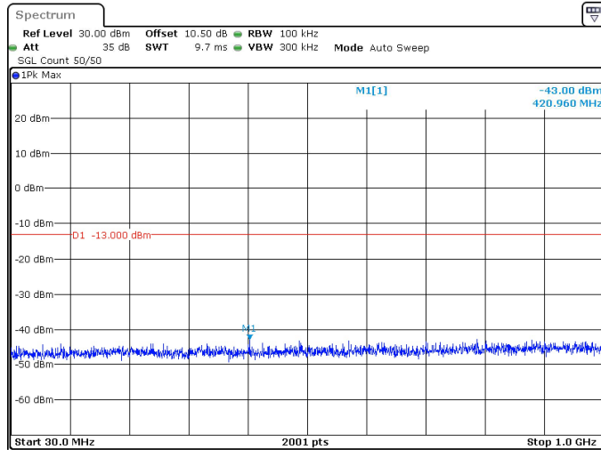
50MHz_30kHz_3475MHz_DFT-s-OFDM QPSK_RB1@132 -43.00 dBm
