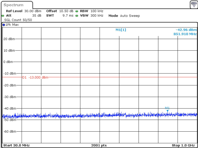
50MHz_15kHz_3500MHz_DFT-s-OFDM QPSK_RB270@0 -42.96 dBm
