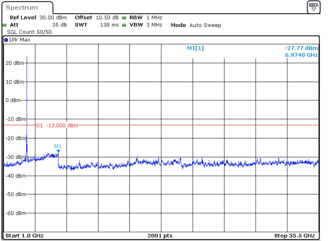
50MHz_15kHz_3525MHz_DFT-s-OFDM QPSK_RB1@269 -27.77 dBm
