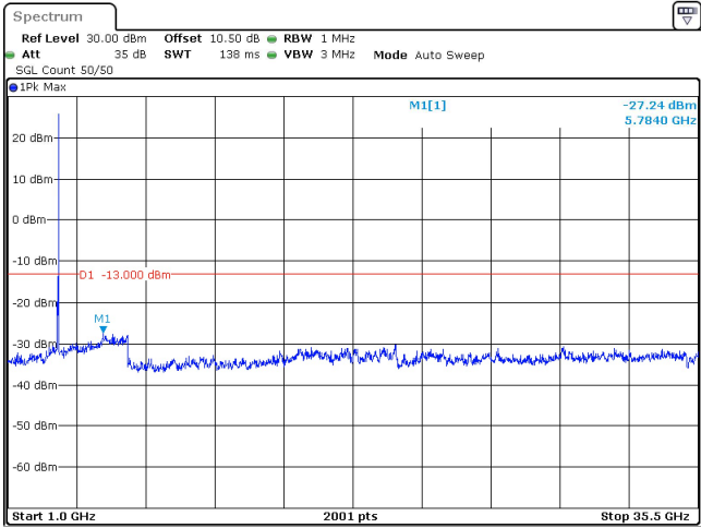
50MHz_15kHz_3500MHz_DFT-s-OFDM QPSK_RB1@269 -27.24 dBm
