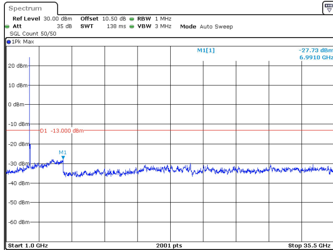
50MHz_15kHz_3500MHz_DFT-s-OFDM QPSK_RB1@0 -27.73 dBm
