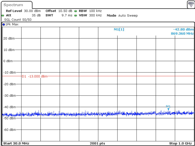
50MHz_15kHz_3475MHz_DFT-s-OFDM QPSK_RB270@0 -42.80 dBm
