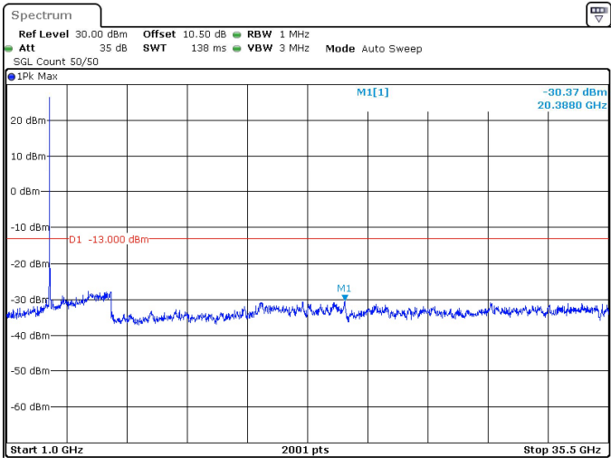
50MHz_30kHz_3475MHz_DFT-s-OFDM QPSK_RB1@0 -30.37 dBm
