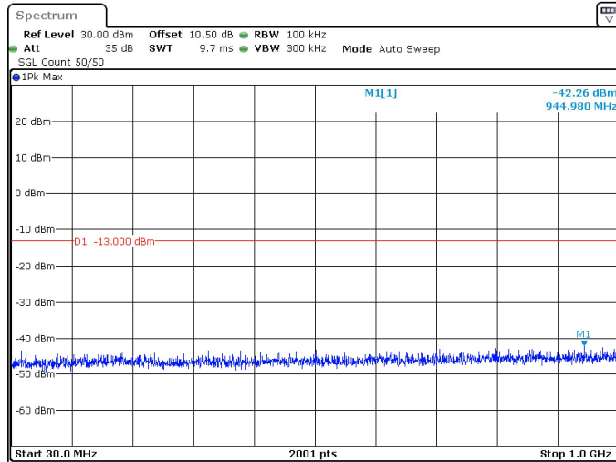
50MHz_30kHz_3475MHz_DFT-s-OFDM QPSK_RB1@0 -42.26 dBm
