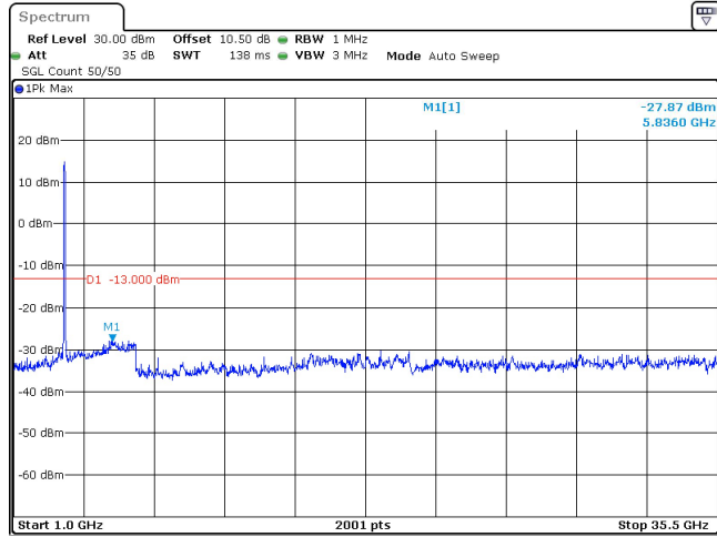
50MHz_15kHz_3500MHz_DFT-s-OFDM QPSK_RB270@0 -27.87 dBm
