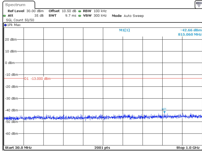
50MHz_30kHz_3475MHz_DFT-s-OFDM QPSK_RB128@0 -42.66 dBm
