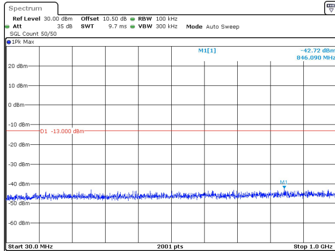
50MHz_15kHz_3525MHz_DFT-s-OFDM QPSK_RB1@269 -42.72 dBm
