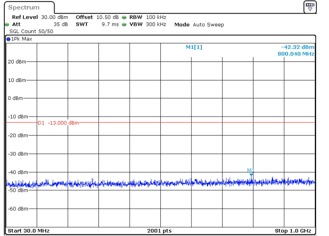
50MHz_15kHz_3525MHz_DFT-s-OFDM QPSK_RB270@0 -42.32 dBm
