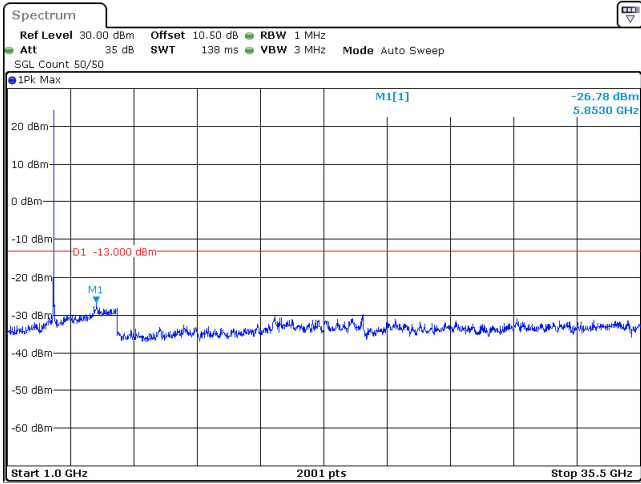
50MHz_30kHz_3525MHz_DFT-s-OFDM QPSK_RB1@132 -26.78 dBm
