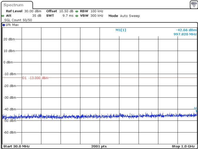
50MHz_30kHz_3500MHz_DFT-s-OFDM QPSK_RB128@0 -42.66 dBm
