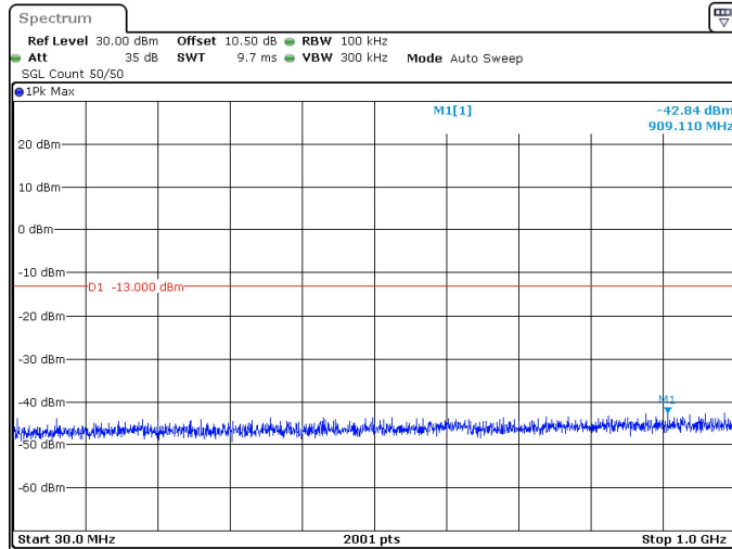
50MHz_30kHz_3525MHz_DFT-s-OFDM QPSK_RB1@132 -42.84 dBm
