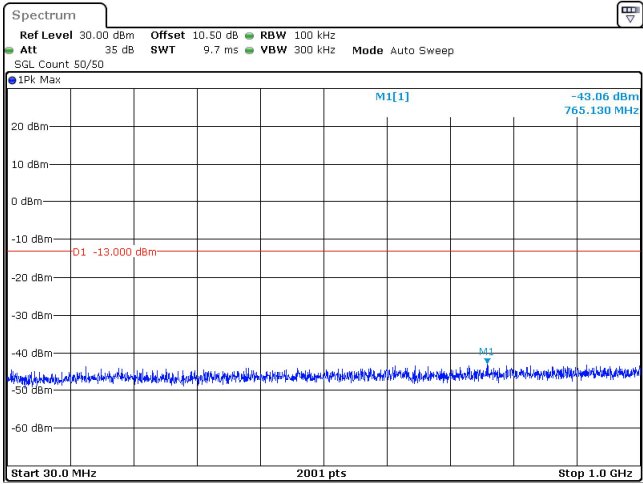
50MHz_30kHz_3500MHz_DFT-s-OFDM QPSK_RB1@132 -43.06 dBm
