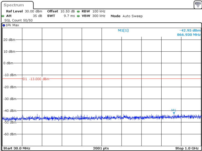
50MHz_30kHz_3525MHz_DFT-s-OFDM QPSK_RB128@0 -42.95 dBm
