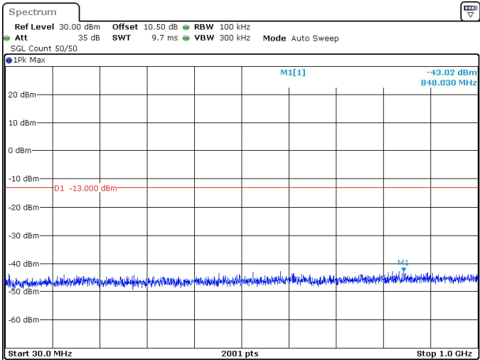
50MHz_30kHz_3525MHz_DFT-s-OFDM QPSK_RB1@0 -43.02 dBm
