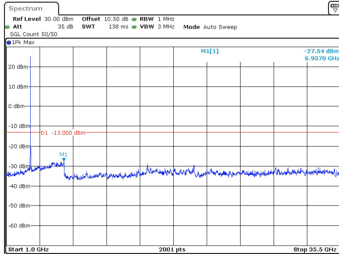
50MHz_30kHz_3525MHz_DFT-s-OFDM QPSK_RB1@0 -27.54 dBm
