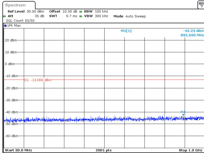
90MHz_30kHz_3505MHz_DFT-s-OFDM QPSK_RB1@244 -43.23 dBm
