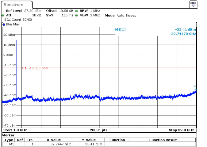
10MHz_30kHz_3840MHz_DFT-s-OFDM QPSK_RB1@23 -35.41 dBm
