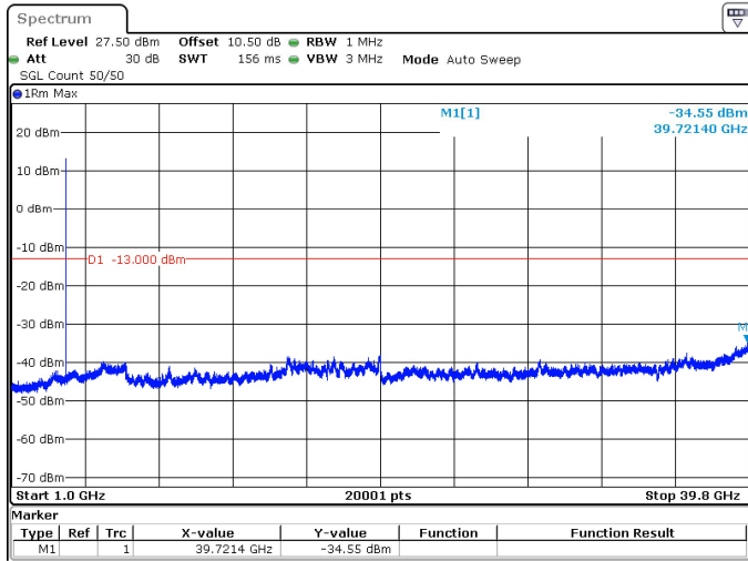
15MHz_30kHz_3840MHz_DFT-s-OFDM QPSK_RB1@0 -34.55 dBm
