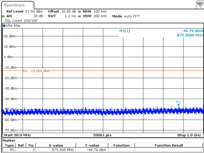
15MHz_30kHz_3972.5MHz_DFT-s-OFDM QPSK_RB1@0 -46.79 dBm
