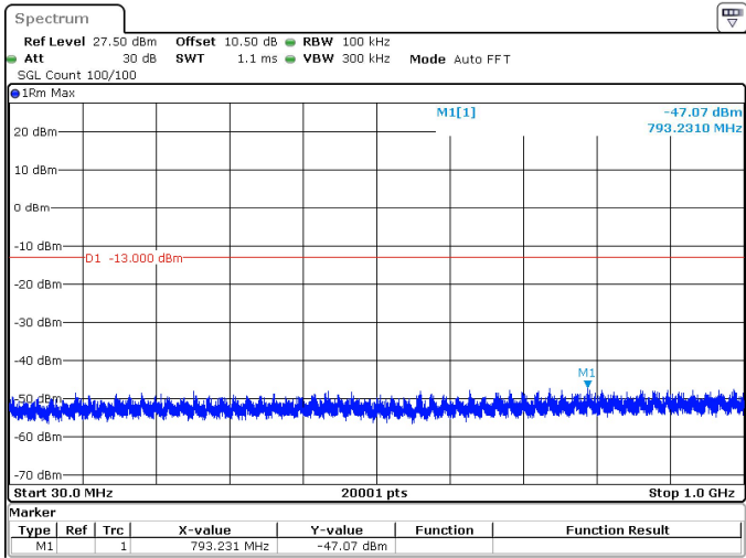
15MHz_30kHz_3972.5MHz_DFT-s-OFDM QPSK_RB1@37 -47.07 dBm
