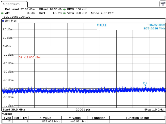
15MHz_30kHz_3707.5MHz_DFT-s-OFDM QPSK_RB1@37 -46.92 dBm
