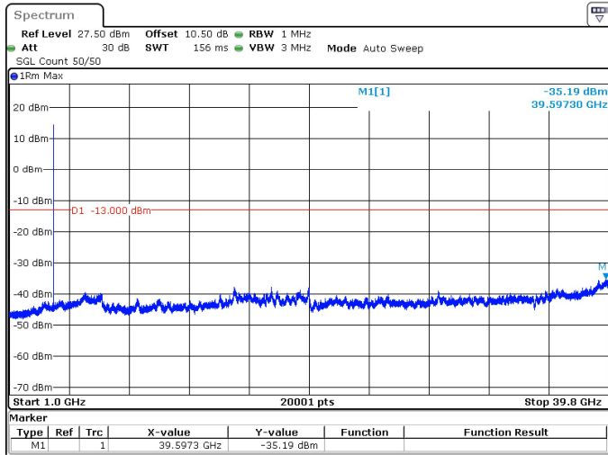
15MHz_30kHz_3840MHz_DFT-s-OFDM QPSK_RB1@37 -35.19 dBm
