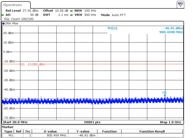
15MHz_30kHz_3707.5MHz_DFT-s-OFDM QPSK_RB36@0 -46.91 dBm
