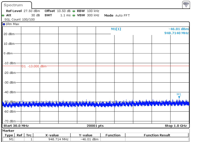
15MHz_30kHz_3972.5MHz_DFT-s-OFDM QPSK_RB36@0 -46.01 dBm
