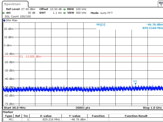
20MHz_15kHz_3840MHz_DFT-s-OFDM QPSK_RB1@0 -46.76 dBm
