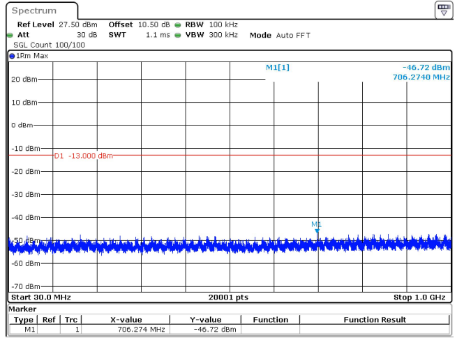
20MHz_15kHz_3840MHz_DFT-s-OFDM QPSK_RB100@0 -46.72 dBm
