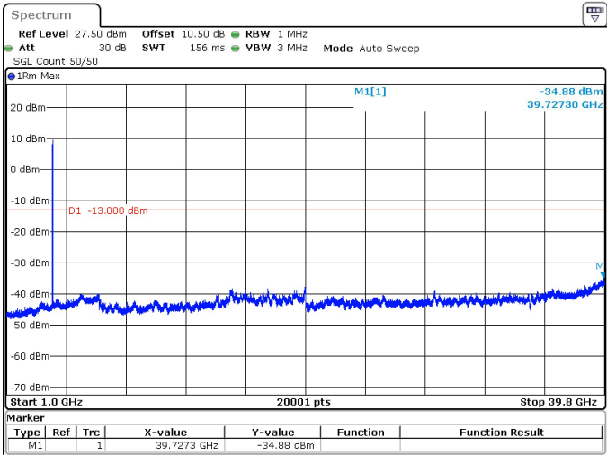
15MHz_30kHz_3972.5MHz_DFT-s-OFDM QPSK_RB36@0 -34.88 dBm
