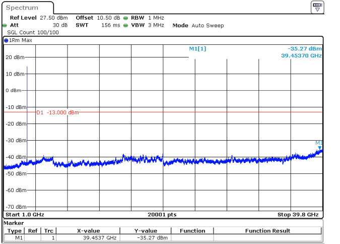
20MHz_15kHz_3840MHz_DFT-s-OFDM QPSK_RB1@105 -35.27 dBm
