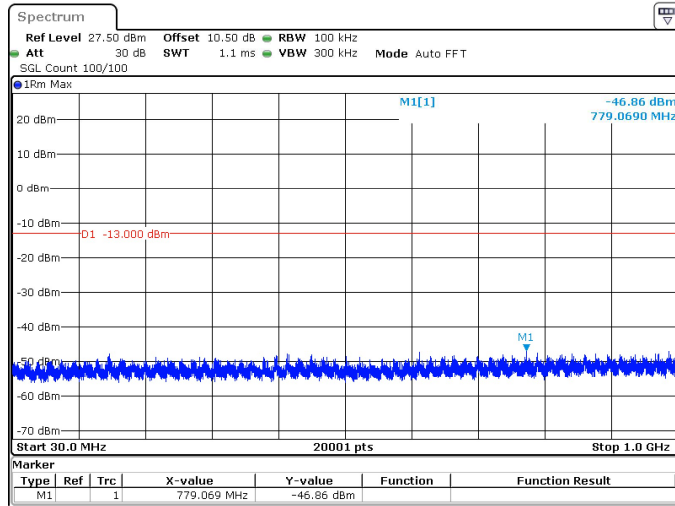
20MHz_15kHz_3840MHz_DFT-s-OFDM QPSK_RB1@105 -46.86 dBm
