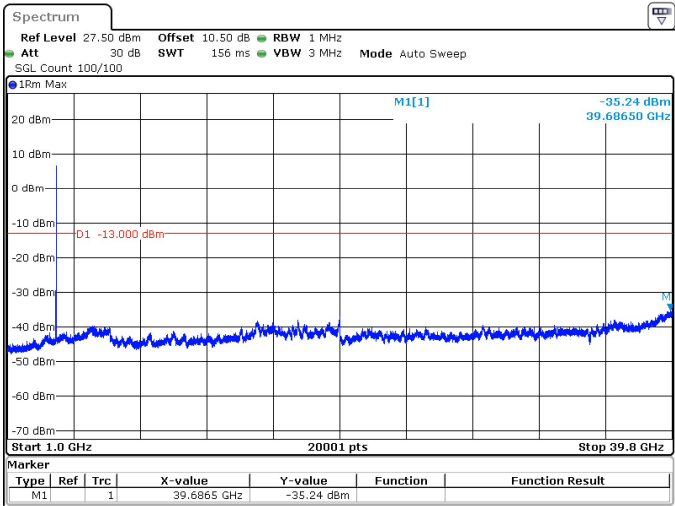
20MHz_15kHz_3840MHz_DFT-s-OFDM QPSK_RB100@0 -35.24 dBm
