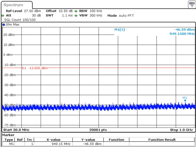
30MHz_15kHz_3840MHz_DFT-s-OFDM QPSK_RB1@0 -46.59 dBm
