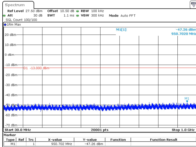
30MHz_15kHz_3840MHz_DFT-s-OFDM QPSK_RB1@159 -47.26 dBm
