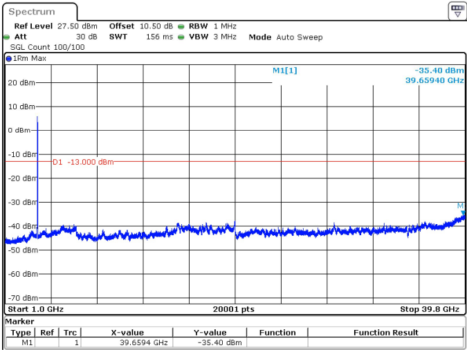
30MHz_15kHz_3715MHz_DFT-s-OFDM QPSK_RB160@0 -35.40 dBm
