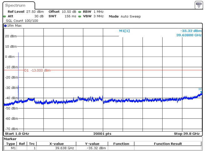
30MHz_15kHz_3840MHz_DFT-s-OFDM QPSK_RB160@0 -35.32 dBm
