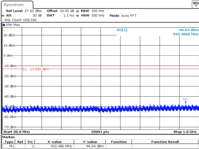
30MHz_15kHz_3715MHz_DFT-s-OFDM QPSK_RB160@0 -46.64 dBm
