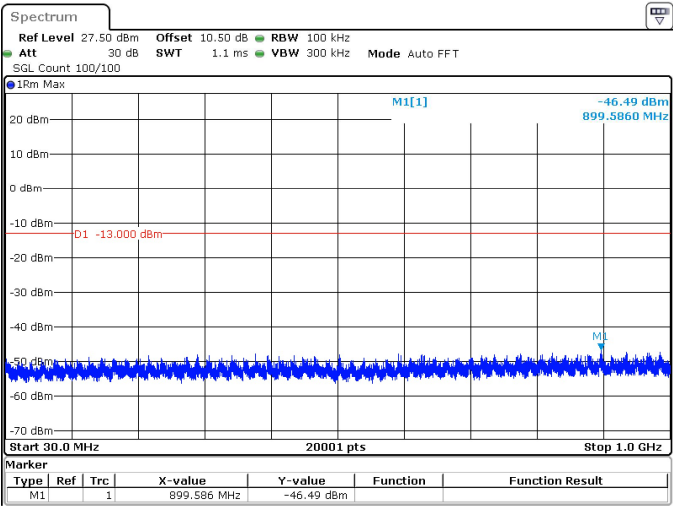
30MHz_15kHz_3715MHz_DFT-s-OFDM QPSK_RB1@0 -46.49 dBm
