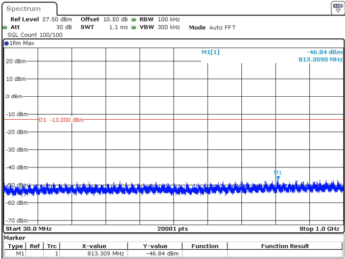
30MHz_15kHz_3840MHz_DFT-s-OFDM QPSK_RB160@0 -46.84 dBm
