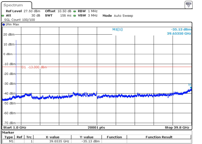
30MHz_15kHz_3840MHz_DFT-s-OFDM QPSK_RB1@159 -35.13 dBm
