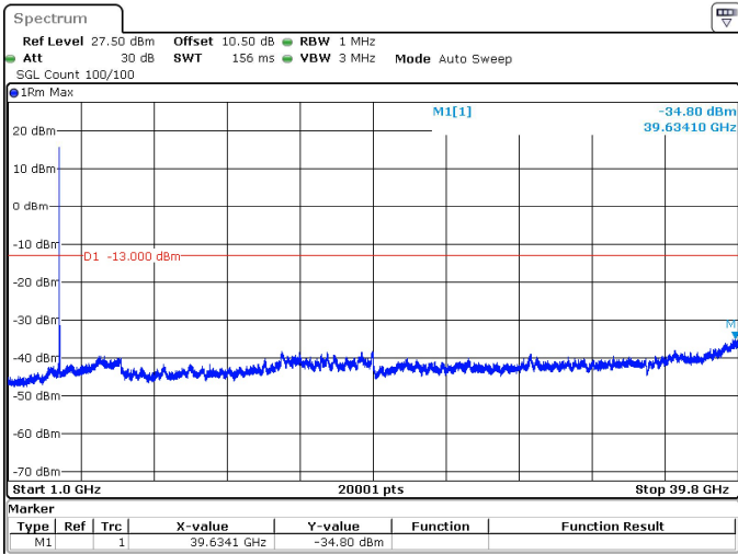
30MHz_15kHz_3715MHz_DFT-s-OFDM QPSK_RB1@0 -34.80 dBm
