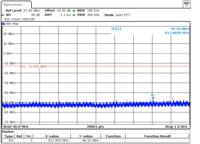
30MHz_15kHz_3965MHz_DFT-s-OFDM QPSK_RB1@159 -46.53 dBm
