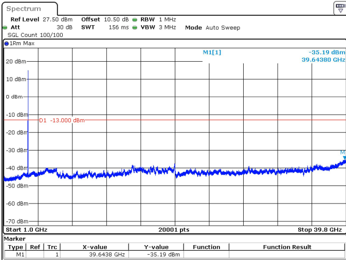
30MHz_15kHz_3715MHz_DFT-s-OFDM QPSK_RB1@159 -35.19 dBm
