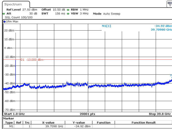
30MHz_15kHz_3840MHz_DFT-s-OFDM QPSK_RB1@0 -34.92 dBm
