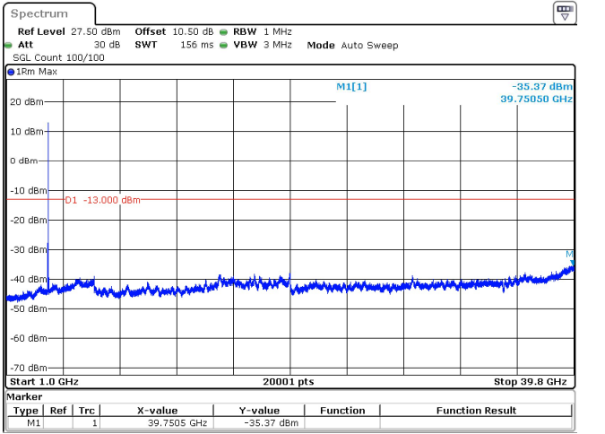
40MHz_15kHz_3840MHz_DFT-s-OFDM QPSK_RB1@215 -35.37 dBm
