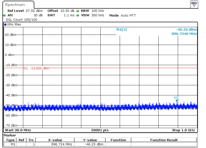
40MHz_15kHz_3840MHz_DFT-s-OFDM QPSK_RB216@0 -46.25 dBm
