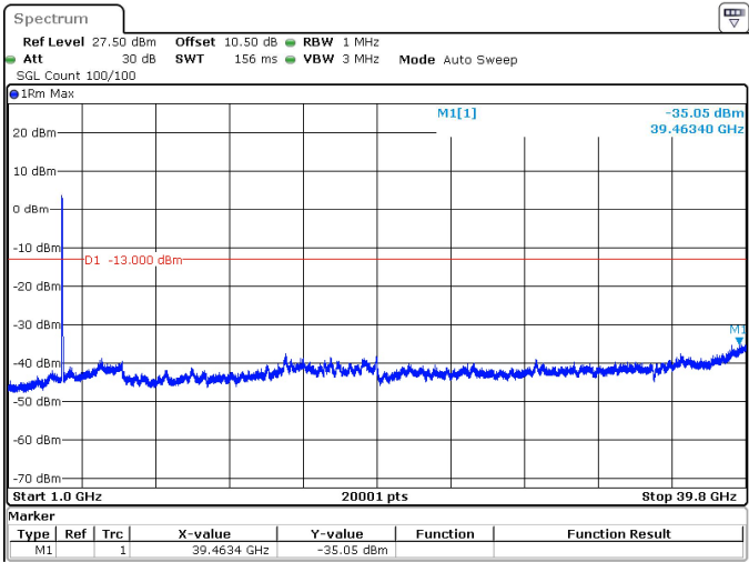
40MHz_15kHz_3840MHz_DFT-s-OFDM QPSK_RB216@0 -35.05 dBm
