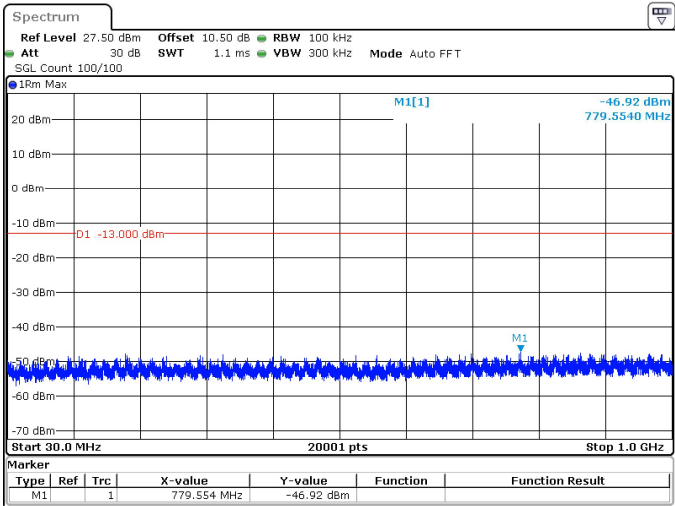
40MHz_15kHz_3840MHz_DFT-s-OFDM QPSK_RB1@0 -46.92 dBm
