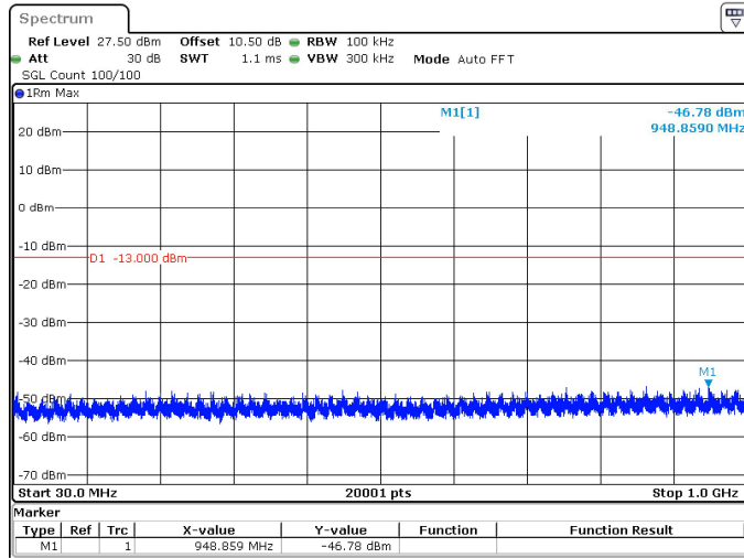
40MHz_15kHz_3840MHz_DFT-s-OFDM QPSK_RB1@215 -46.78 dBm
