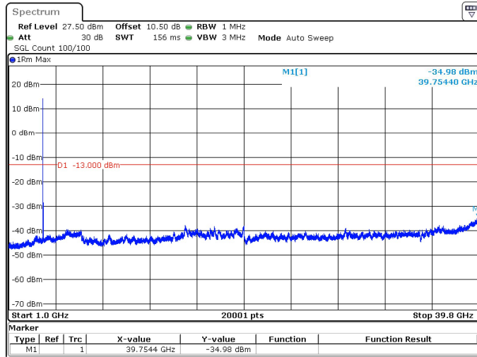
40MHz_15kHz_3840MHz_DFT-s-OFDM QPSK_RB1@0 -34.98 dBm
