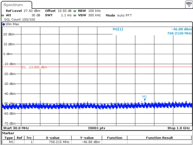
50MHz_15kHz_3840MHz_DFT-s-OFDM QPSK_RB270@0 -46.88 dBm
