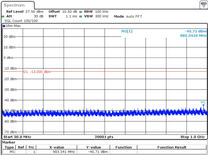
50MHz_15kHz_3840MHz_DFT-s-OFDM QPSK_RB1@0 -45.71 dBm
