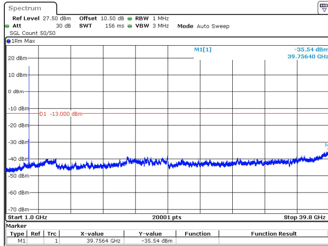
50MHz_15kHz_3725MHz_DFT-s-OFDM QPSK_RB1@269 -35.54 dBm
