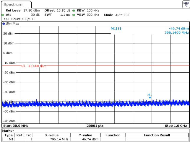
50MHz_15kHz_3955MHz_DFT-s-OFDM QPSK_RB1@269 -46.74 dBm
