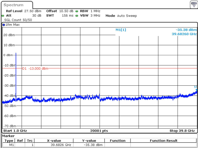
50MHz_15kHz_3725MHz_DFT-s-OFDM QPSK_RB270@0 -35.38 dBm
