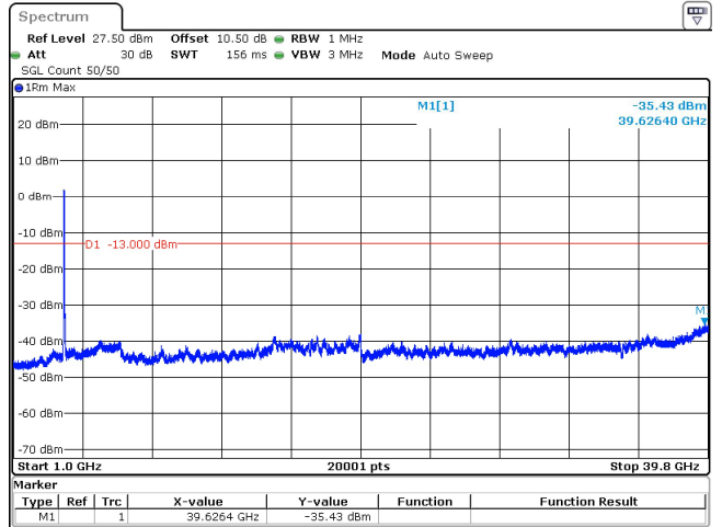
50MHz_15kHz_3840MHz_DFT-s-OFDM QPSK_RB270@0 -35.43 dBm
