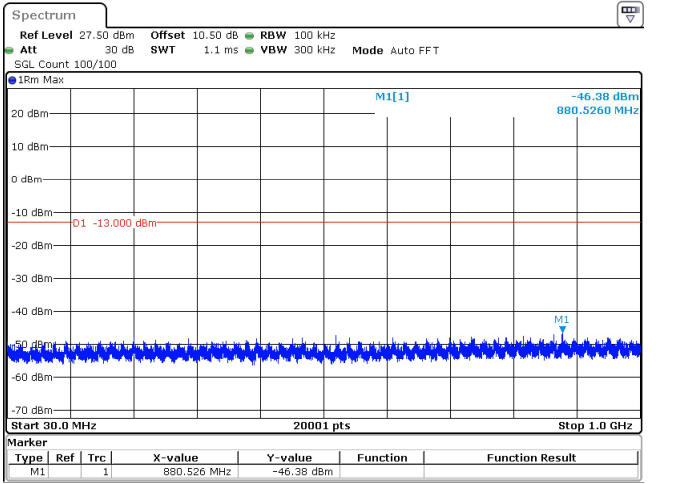
50MHz_15kHz_3725MHz_DFT-s-OFDM QPSK_RB1@269 -46.38 dBm
