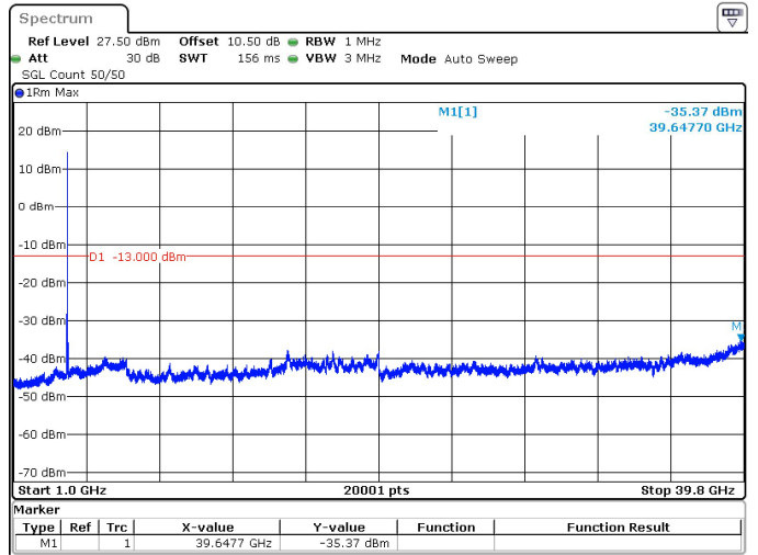
50MHz_15kHz_3840MHz_DFT-s-OFDM QPSK_RB1@269 -35.37 dBm
