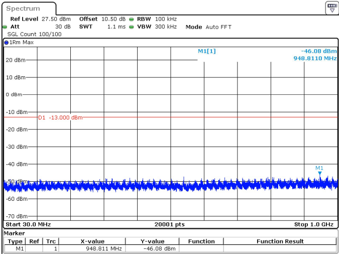
50MHz_15kHz_3955MHz_DFT-s-OFDM QPSK_RB1@0 -46.08 dBm
