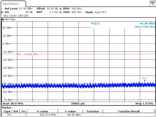
50MHz_15kHz_3840MHz_DFT-s-OFDM QPSK_RB1@269 -46.98 dBm
