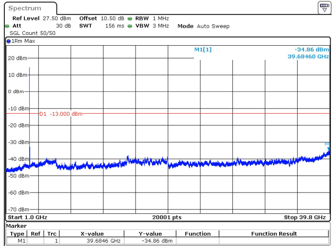
50MHz_15kHz_3840MHz_DFT-s-OFDM QPSK_RB1@0 -34.86 dBm
