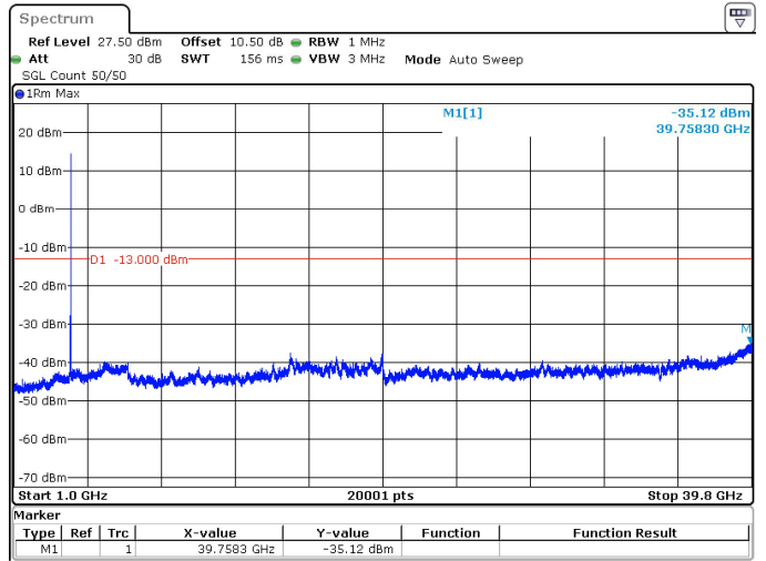
50MHz_15kHz_3955MHz_DFT-s-OFDM QPSK_RB1@269 -35.12 dBm
