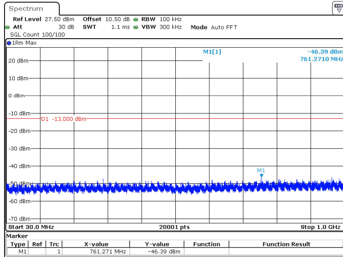
50MHz_15kHz_3725MHz_DFT-s-OFDM QPSK_RB1@0 -46.39 dBm
