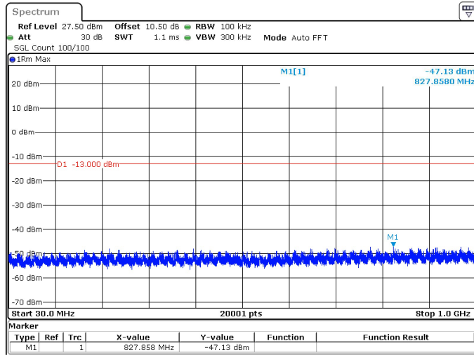
80MHz_30kHz_3840MHz_DFT-s-OFDM QPSK_RB1@216 -47.13 dBm
