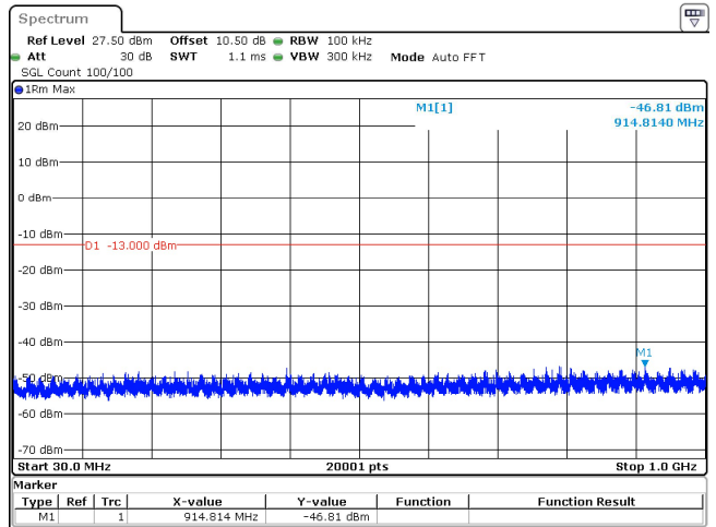
80MHz_30kHz_3740MHz_DFT-s-OFDM QPSK_RB216@0 -46.81 dBm
