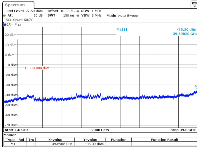
80MHz_30kHz_3840MHz_DFT-s-OFDM QPSK_RB1@0 -35.39 dBm
