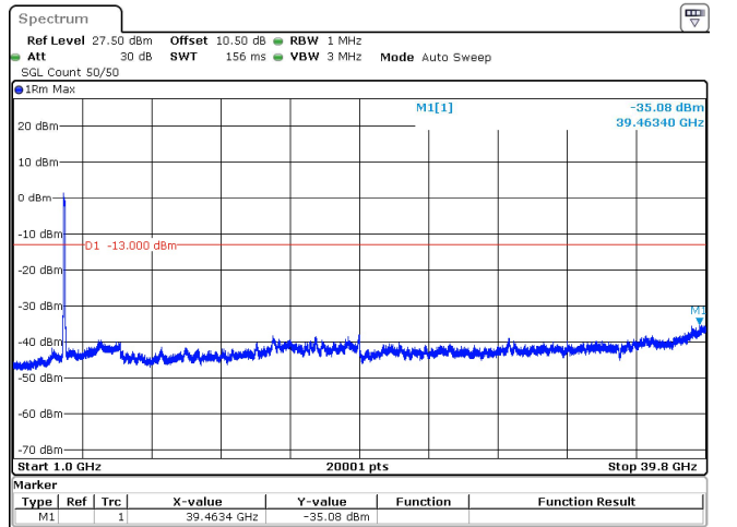
80MHz_30kHz_3840MHz_DFT-s-OFDM QPSK_RB216@0 -35.08 dBm
