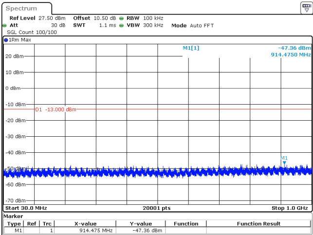
90MHz_30kHz_3840MHz_DFT-s-OFDM QPSK_RB1@244 -47.36 dBm
