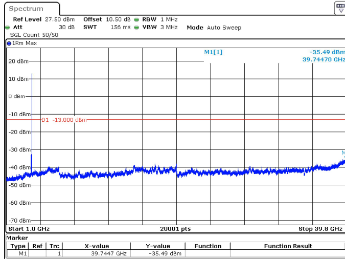
90MHz_30kHz_3840MHz_DFT-s-OFDM QPSK_RB1@244 -35.49 dBm
