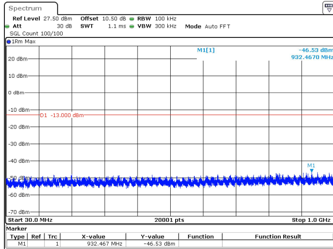
90MHz_30kHz_3840MHz_DFT-s-OFDM QPSK_RB1@0 -46.53 dBm
