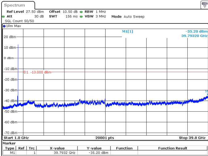
100MHz_30kHz_3840MHz_DFT-s-OFDM QPSK_RB1@272 -35.20 dBm
