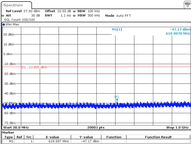
100MHz_30kHz_3840MHz_DFT-s-OFDM QPSK_RB1@272 -47.17 dBm
