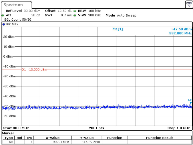
10MHz_30kHz_3545MHz_DFT-s-OFDM QPSK_RB1@0 -47.59 dBm
