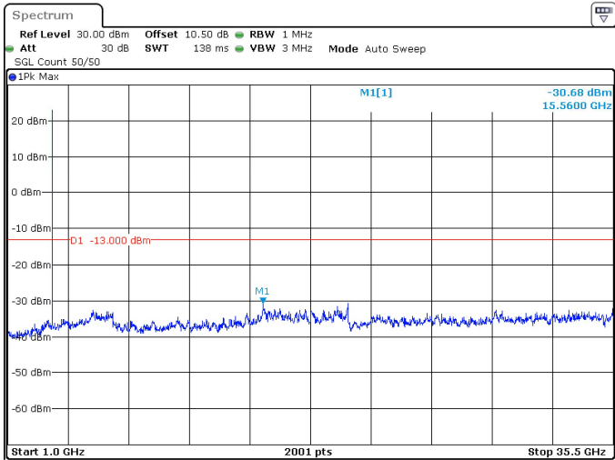
10MHz_30kHz_3545MHz_DFT-s-OFDM QPSK_RB1@0 -30.68 dBm
