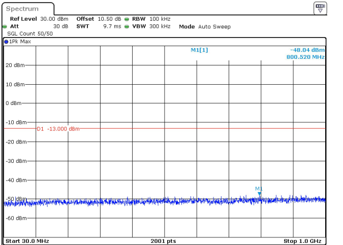
10MHz_30kHz_3545MHz_DFT-s-OFDM QPSK_RB1@0 -48.04 dBm
