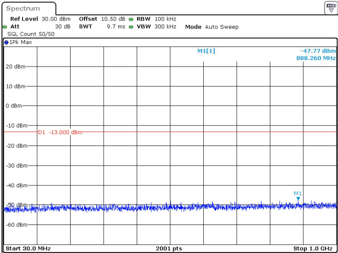
10MHz_30kHz_3545MHz_DFT-s-OFDM QPSK_RB1@23 -47.77 dBm
