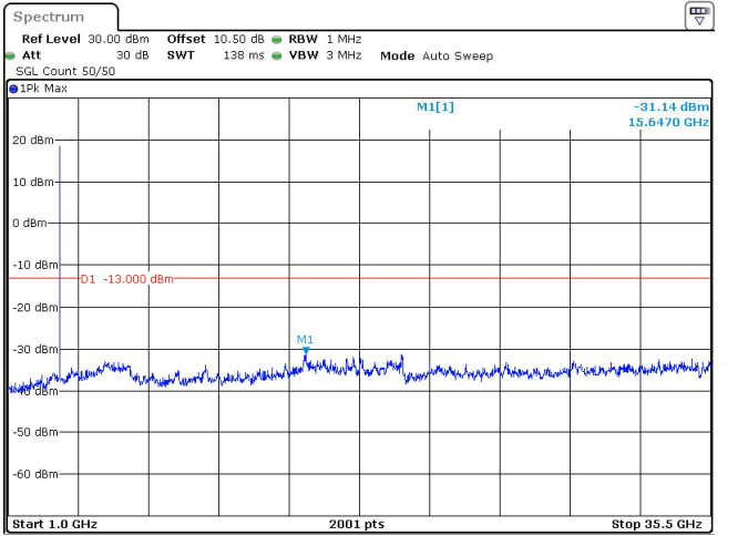
10MHz_30kHz_3545MHz_DFT-s-OFDM QPSK_RB24@0 -31.14 dBm
