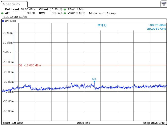
10MHz_30kHz_3545MHz_DFT-s-OFDM QPSK_RB1@23 -30.70 dBm
