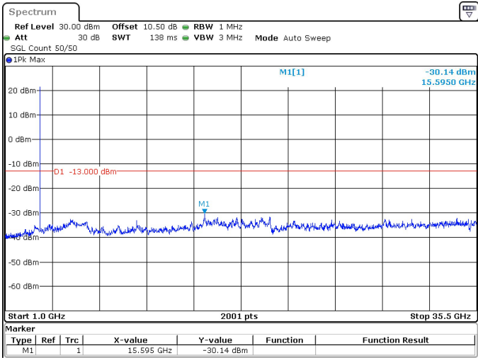
10MHz_30kHz_3545MHz_DFT-s-OFDM QPSK_RB24@0 -30.14 dBm
