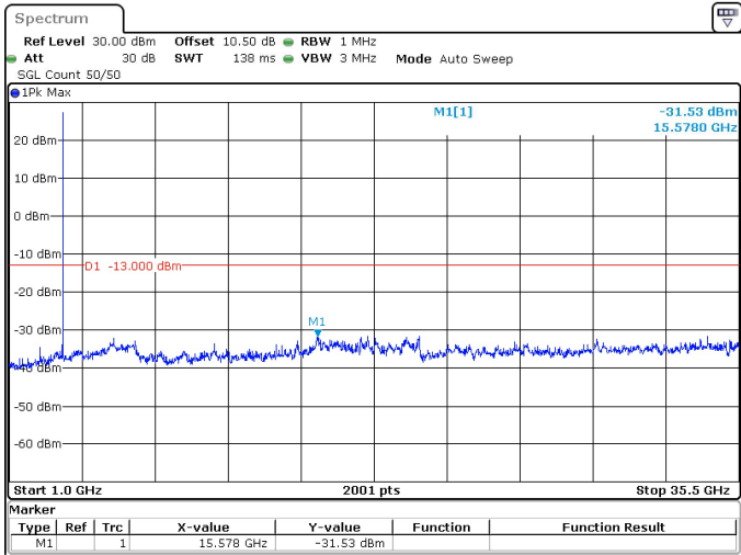
10MHz_30kHz_3545MHz_DFT-s-OFDM QPSK_RB1@0 -31.53 dBm
