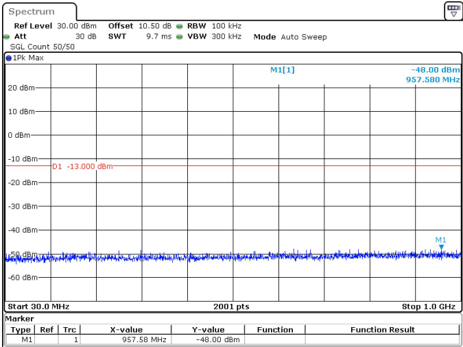
10MHz_30kHz_3545MHz_DFT-s-OFDM QPSK_RB1@23 -48.00 dBm
