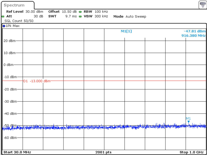
15MHz_30kHz_3500MHz_DFT-s-OFDM QPSK_RB36@0 -47.81 dBm
