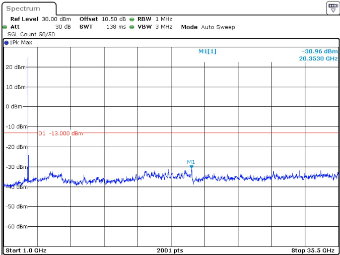
15MHz_30kHz_3500MHz_DFT-s-OFDM QPSK_RB1@37 -30.96 dBm
