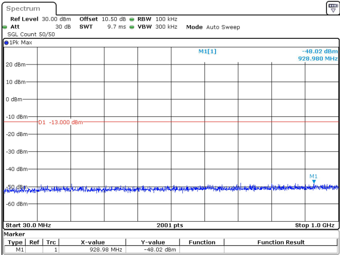
15MHz_30kHz_3457.5MHz_DFT-s-OFDM QPSK_RB1@37 -48.02 dBm
