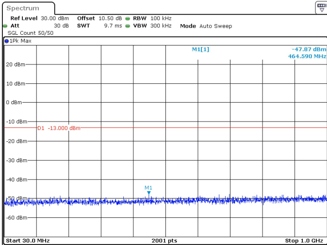
15MHz_30kHz_3457.5MHz_DFT-s-OFDM QPSK_RB1@0 -47.87 dBm
