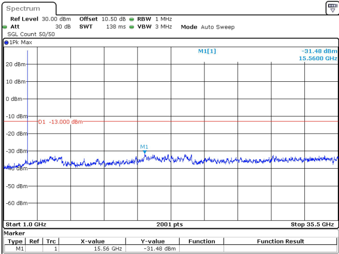
15MHz_30kHz_3457.5MHz_DFT-s-OFDM QPSK_RB1@37 -31.48 dBm
