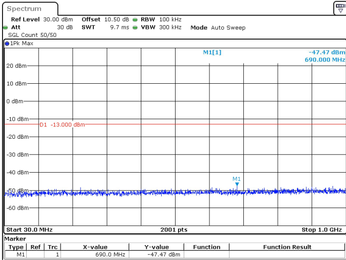
15MHz_30kHz_3457.5MHz_DFT-s-OFDM QPSK_RB1@0 -47.47 dBm
