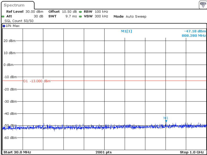
15MHz_30kHz_3500MHz_DFT-s-OFDM QPSK_RB1@37 -47.18 dBm
