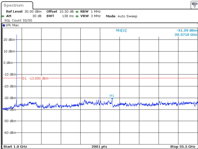
15MHz_30kHz_3542.5MHz_DFT-s-OFDM QPSK_RB1@0 -31.59 dBm
