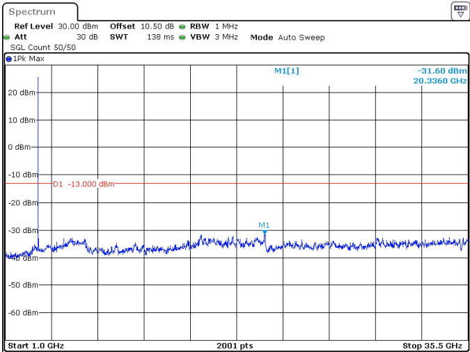
15MHz_30kHz_3457.5MHz_DFT-s-OFDM QPSK_RB1@0 -31.60 dBm
