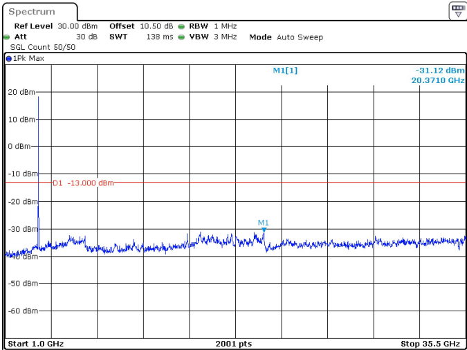
15MHz_30kHz_3500MHz_DFT-s-OFDM QPSK_RB36@0 -31.12 dBm
