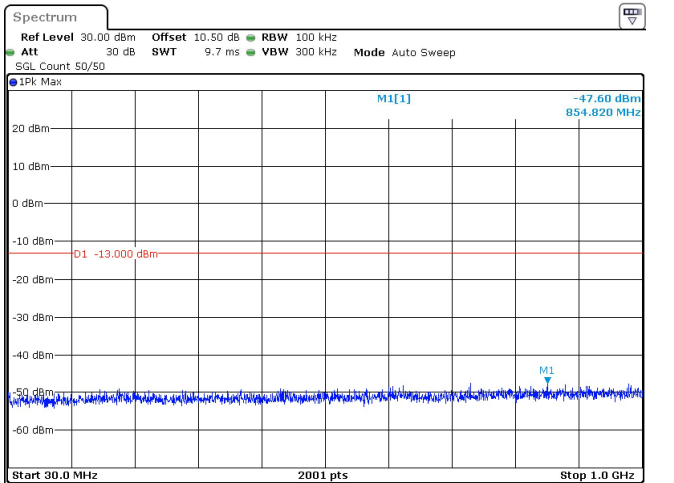
15MHz_30kHz_3457.5MHz_DFT-s-OFDM QPSK_RB1@37 -47.60 dBm
