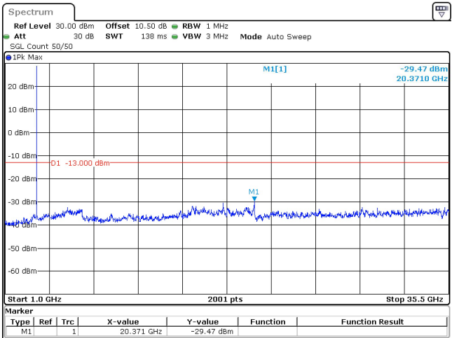
15MHz_30kHz_3457.5MHz_DFT-s-OFDM QPSK_RB1@0 -29.47 dBm
