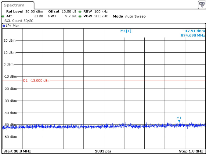
15MHz_30kHz_3457.5MHz_DFT-s-OFDM QPSK_RB36@0 -47.91 dBm
