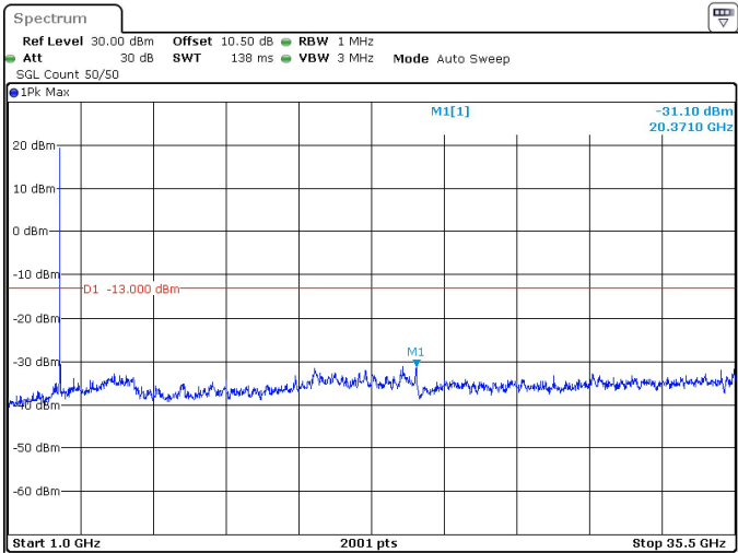
15MHz_30kHz_3457.5MHz_DFT-s-OFDM QPSK_RB36@0 -31.10 dBm
