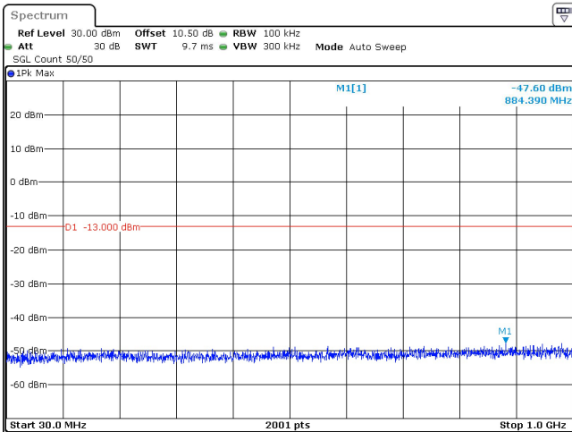
15MHz_30kHz_3500MHz_DFT-s-OFDM QPSK_RB1@0 -47.60 dBm
