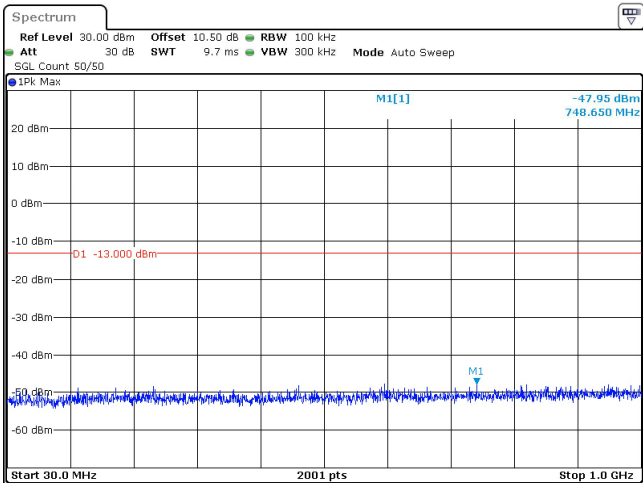
15MHz_30kHz_3542.5MHz_DFT-s-OFDM QPSK_RB1@0 -47.95 dBm
