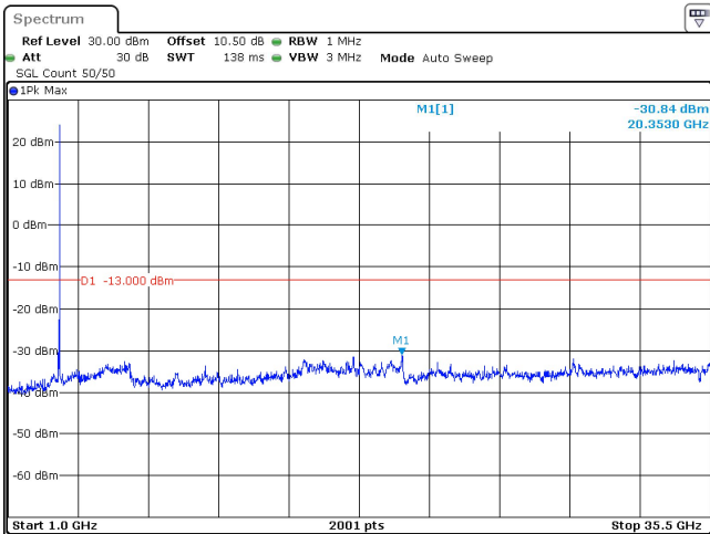
30MHz_30kHz_3535MHz_DFT-s-OFDM QPSK_RB1@0 -30.84 dBm
