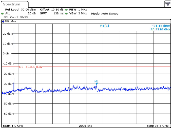
30MHz_30kHz_3465MHz_DFT-s-OFDM QPSK_RB1@77 -31.16 dBm
