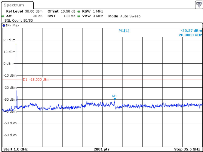
25MHz_30kHz_3537.5MHz_DFT-s-OFDM QPSK_RB64@0 -30.57 dBm
