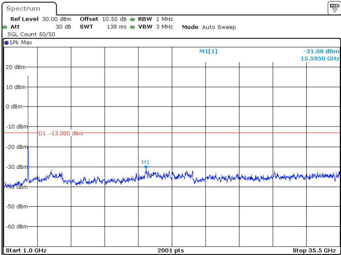
30MHz_30kHz_3500MHz_DFT-s-OFDM QPSK_RB75@0 -31.08 dBm
