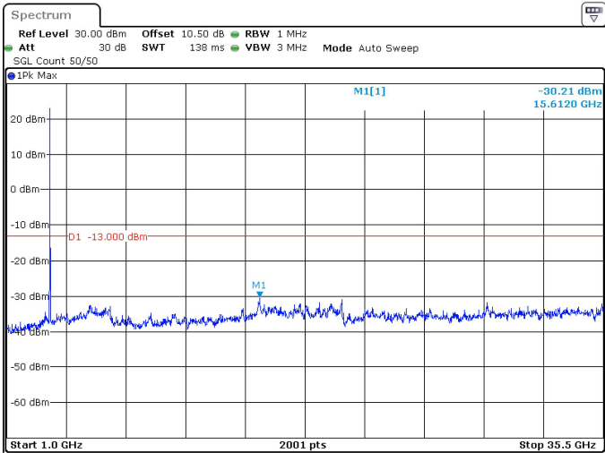
30MHz_30kHz_3500MHz_DFT-s-OFDM QPSK_RB1@77 -30.21 dBm
