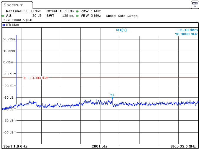
25MHz_30kHz_3537.5MHz_DFT-s-OFDM QPSK_RB1@64 -31.18 dBm
