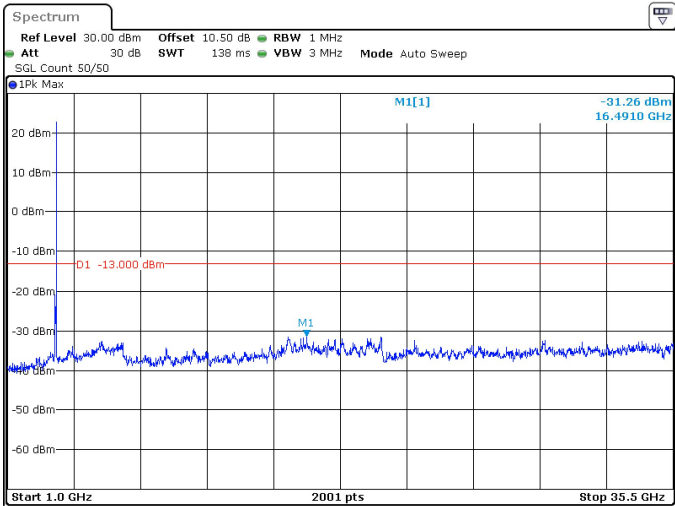
60MHz_30kHz_3500MHz_DFT-s-OFDM QPSK_RB1@161 -31.26 dBm
