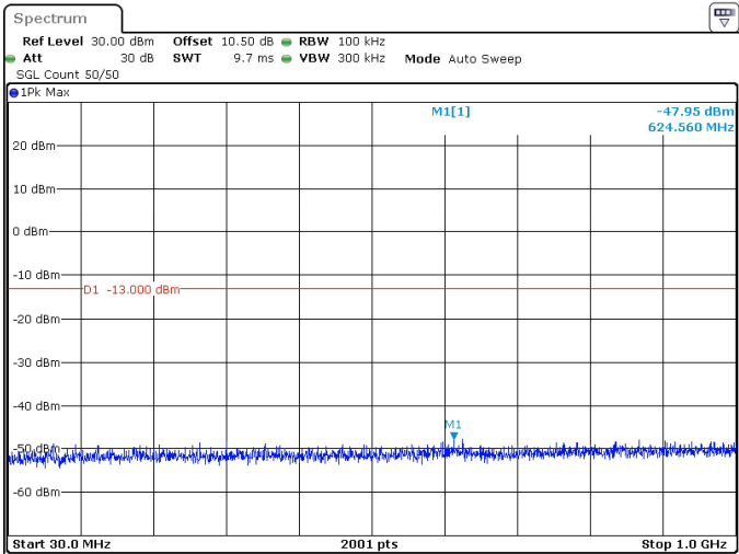
50MHz_30kHz_3525MHz_DFT-s-OFDM QPSK_RB1@132 -47.95 dBm
