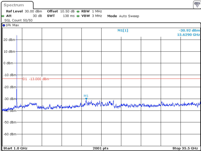
50MHz_30kHz_3525MHz_DFT-s-OFDM QPSK_RB1@132 -30.92 dBm
