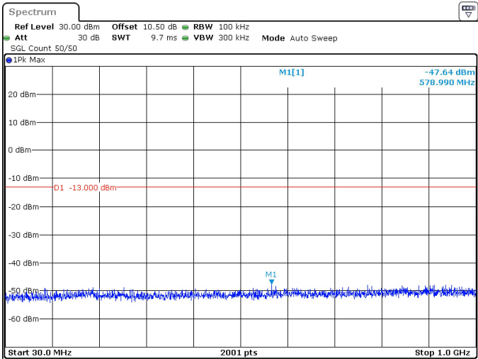
50MHz_30kHz_3525MHz_DFT-s-OFDM QPSK_RB128@0 -47.64 dBm
