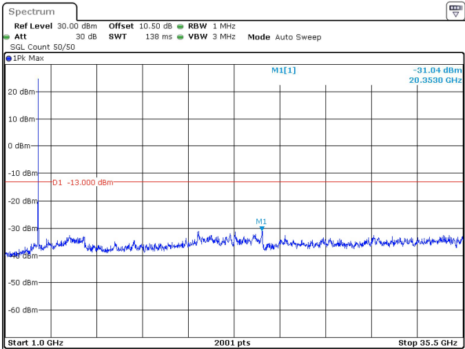
60MHz_30kHz_3480MHz_DFT-s-OFDM QPSK_RB1@161 -31.04 dBm
