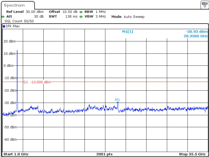
60MHz_30kHz_3500MHz_DFT-s-OFDM QPSK_RB162@0 -30.93 dBm
