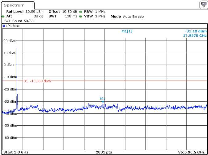
60MHz_30kHz_3480MHz_DFT-s-OFDM QPSK_RB162@0 -31.10 dBm
