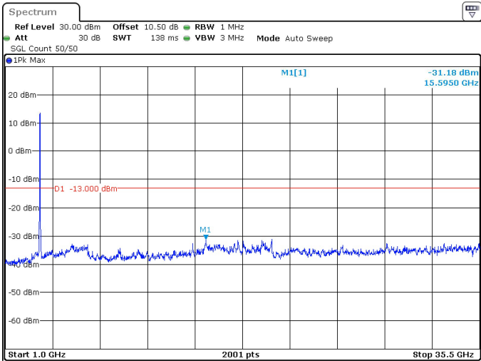
50MHz_30kHz_3525MHz_DFT-s-OFDM QPSK_RB128@0 -31.18 dBm
