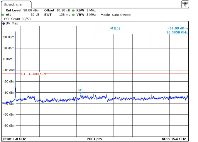
90MHz_30kHz_3505MHz_DFT-s-OFDM QPSK_RB1@0 -31.09 dBm
