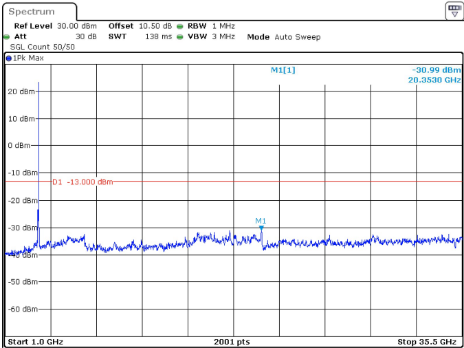
90MHz_30kHz_3495MHz_DFT-s-OFDM QPSK_RB1@244 -30.99 dBm
