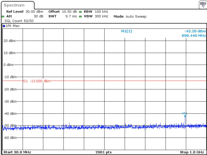
90MHz_30kHz_3495MHz_DFT-s-OFDM QPSK_RB1@244 -43.20 dBm
