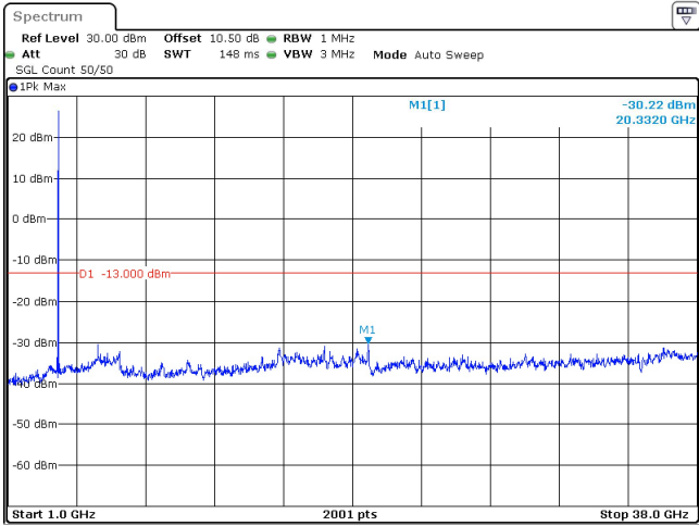
15MHz_15kHz_3707.5MHz_DFT-s-OFDM QPSK_RB1@0 -30.22 dBm
