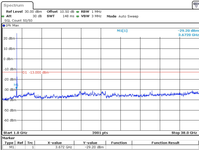
15MHz_15kHz_3750MHz_DFT-s-OFDM QPSK_RB1@0 -29.20 dBm
