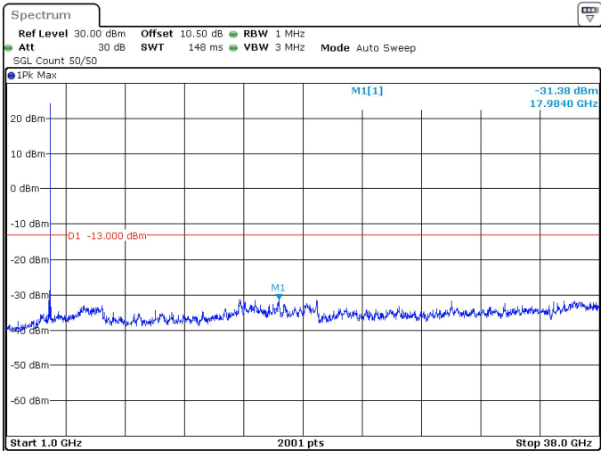
15MHz_15kHz_3707.5MHz_DFT-s-OFDM QPSK_RB1@78 -31.38 dBm
