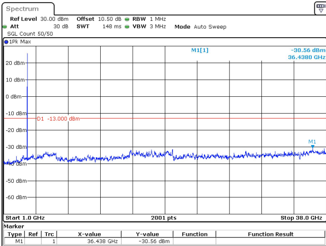
15MHz_30kHz_3707.5MHz_DFT-s-OFDM QPSK_RB1@0 -30.56 dBm
