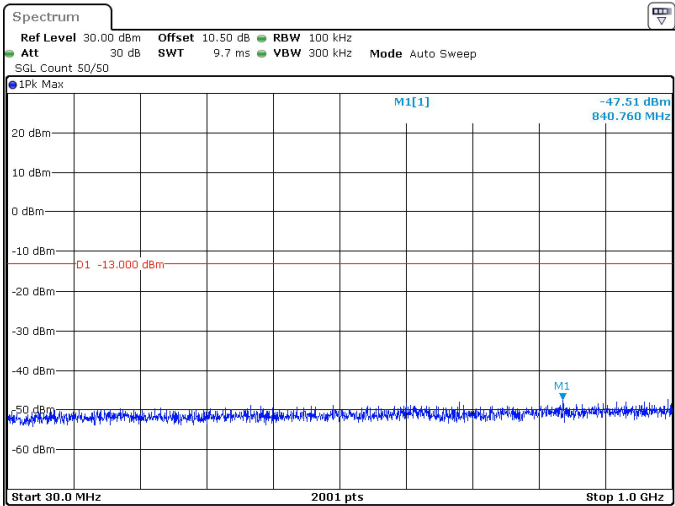
15MHz_15kHz_3750MHz_DFT-s-OFDM QPSK_RB1@78 -47.51 dBm
