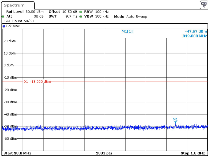
15MHz_15kHz_3792.5MHz_DFT-s-OFDM QPSK_RB75@0 -47.67 dBm
