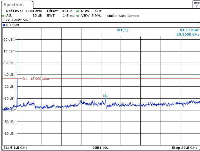
15MHz_15kHz_3792.5MHz_DFT-s-OFDM QPSK_RB1@0 -31.17 dBm
