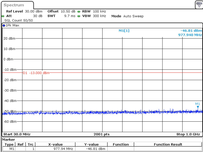
15MHz_30kHz_3707.5MHz_DFT-s-OFDM QPSK_RB36@0 -46.81 dBm
