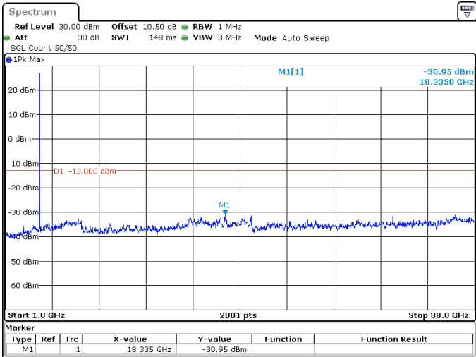
15MHz_30kHz_3707.5MHz_DFT-s-OFDM QPSK_RB1@37 -30.95 dBm
