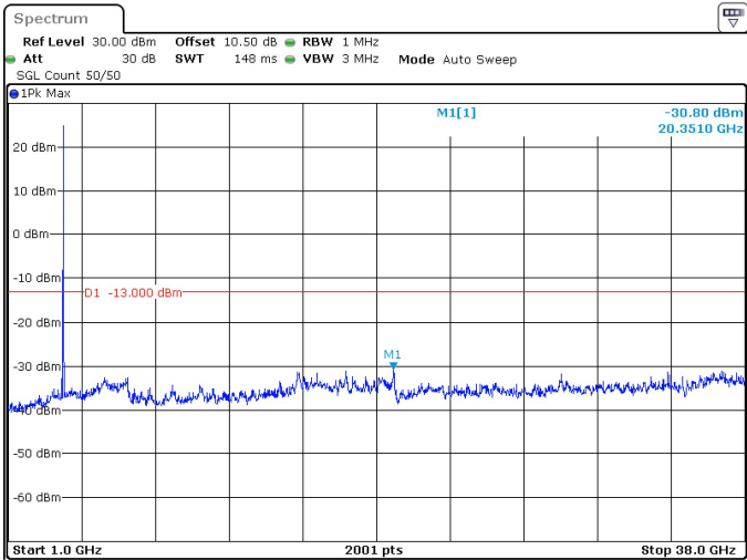
15MHz_15kHz_3750MHz_DFT-s-OFDM QPSK_RB1@78 -30.80 dBm
