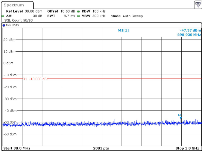
15MHz_15kHz_3750MHz_DFT-s-OFDM QPSK_RB75@0 -47.37 dBm
