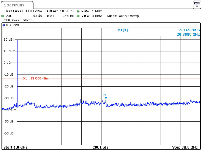
15MHz_15kHz_3792.5MHz_DFT-s-OFDM QPSK_RB75@0 -30.63 dBm
