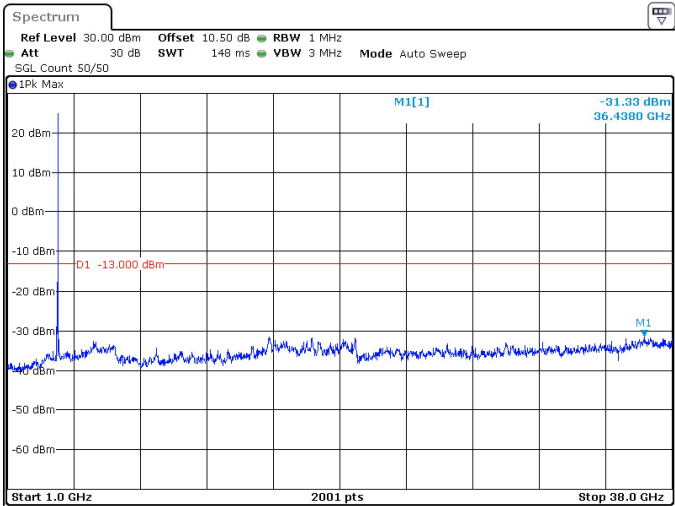
15MHz_15kHz_3792.5MHz_DFT-s-OFDM QPSK_RB1@78 -31.33 dBm
