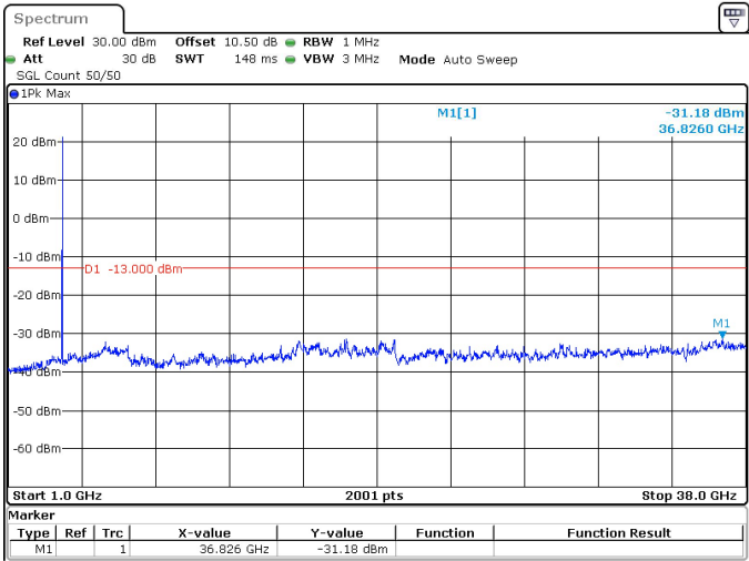
15MHz_30kHz_3707.5MHz_DFT-s-OFDM QPSK_RB36@0 -31.18 dBm
