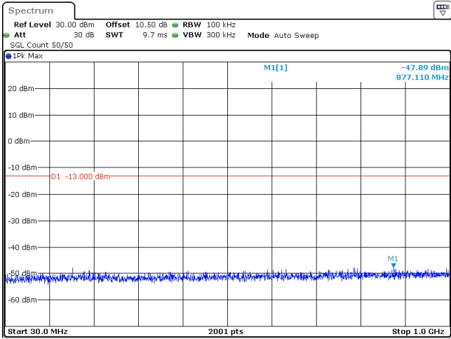
15MHz_15kHz_3792.5MHz_DFT-s-OFDM QPSK_RB1@0 -47.89 dBm
