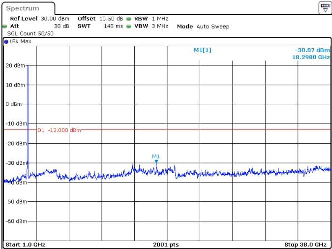
15MHz_15kHz_3750MHz_DFT-s-OFDM QPSK_RB75@0 -30.07 dBm
