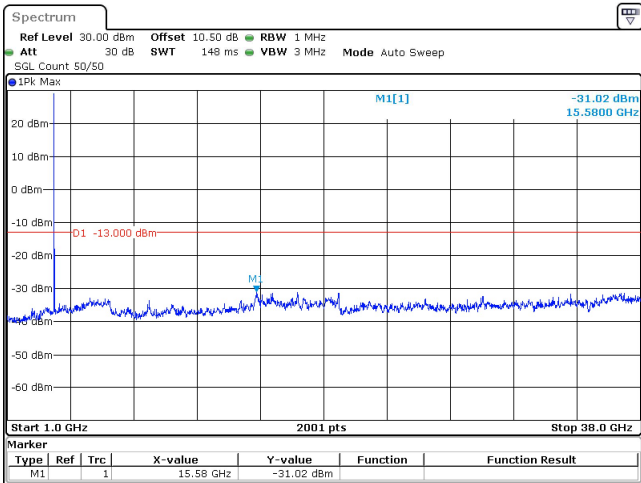
15MHz_30kHz_3750MHz_DFT-s-OFDM QPSK_RB1@0 -31.02 dBm
