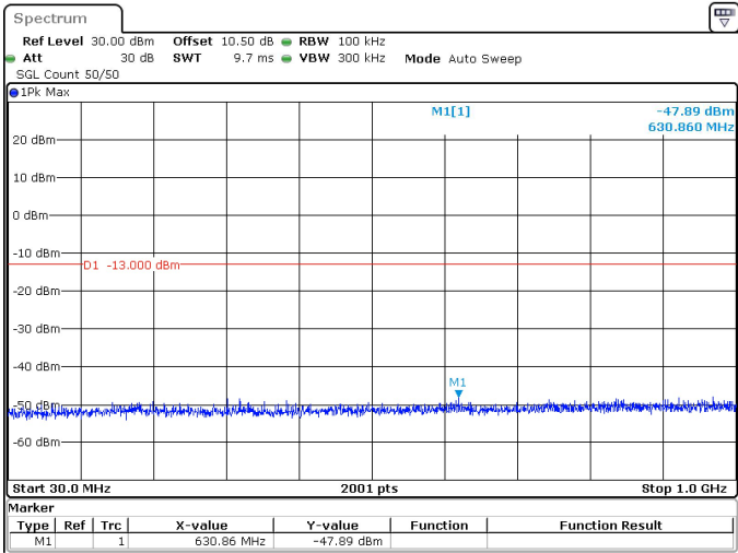
15MHz_30kHz_3750MHz_DFT-s-OFDM QPSK_RB1@37 -47.89 dBm
