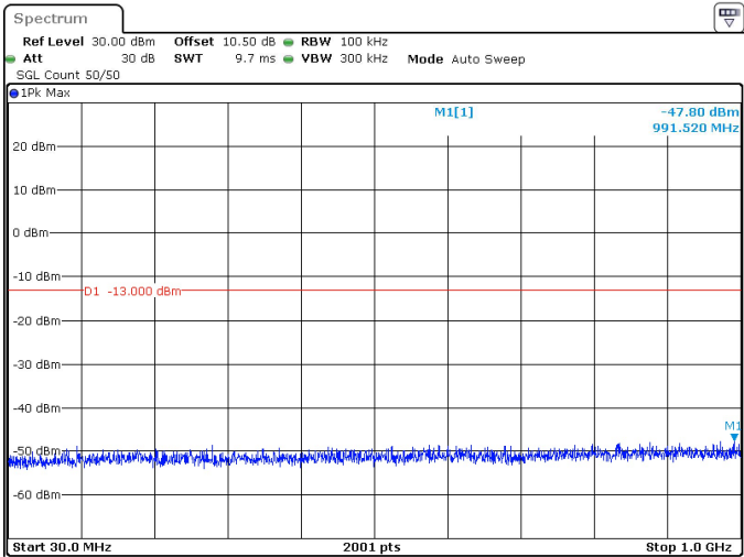
25MHz_15kHz_3712.5MHz_DFT-s-OFDM QPSK_RB1@132 -47.80 dBm
