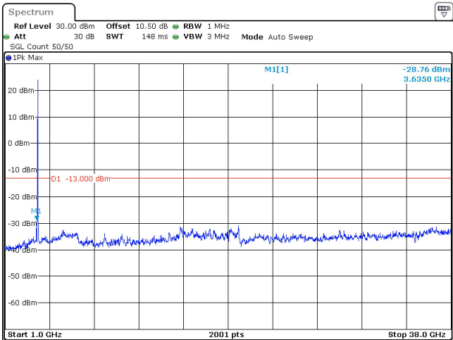
25MHz_15kHz_3712.5MHz_DFT-s-OFDM QPSK_RB1@0 -28.76 dBm
