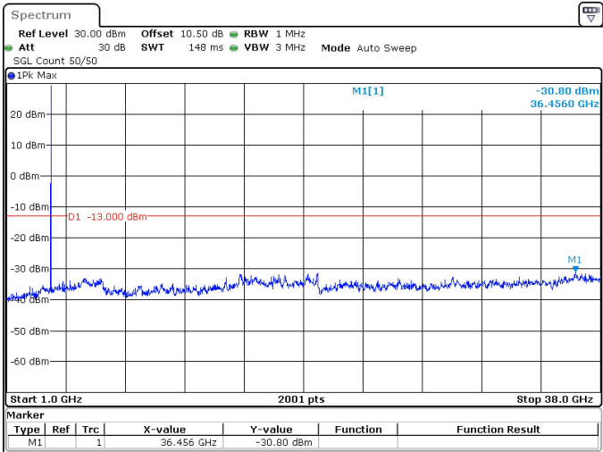
15MHz_30kHz_3750MHz_DFT-s-OFDM QPSK_RB1@37 -30.80 dBm
