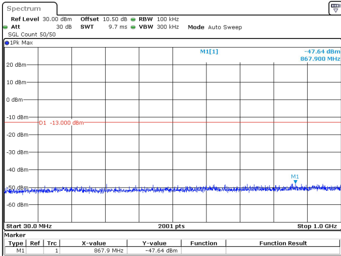
15MHz_30kHz_3792.5MHz_DFT-s-OFDM QPSK_RB36@0 -47.64 dBm
