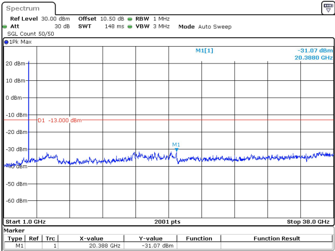
15MHz_30kHz_3792.5MHz_DFT-s-OFDM QPSK_RB36@0 -31.07 dBm
