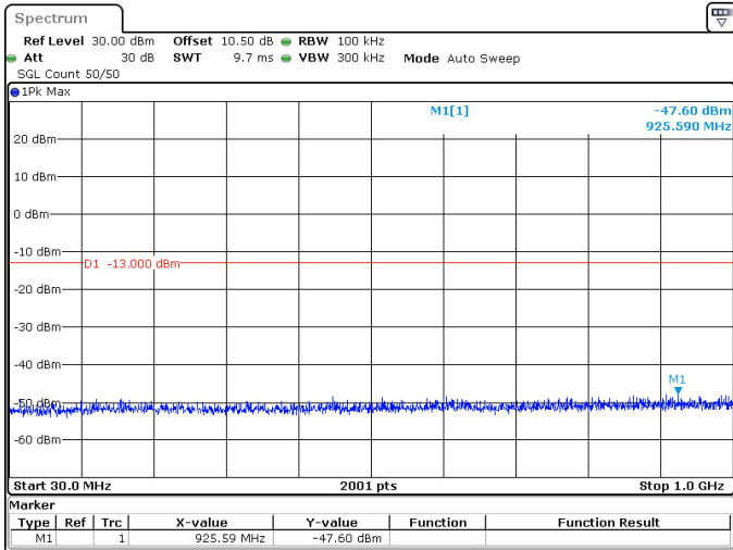
15MHz_30kHz_3792.5MHz_DFT-s-OFDM QPSK_RB1@37 -47.60 dBm
