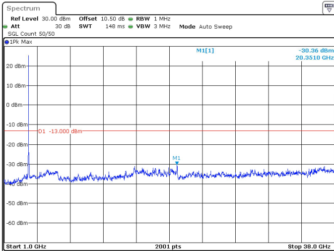
25MHz_15kHz_3712.5MHz_DFT-s-OFDM QPSK_RB1@132 -30.36 dBm
