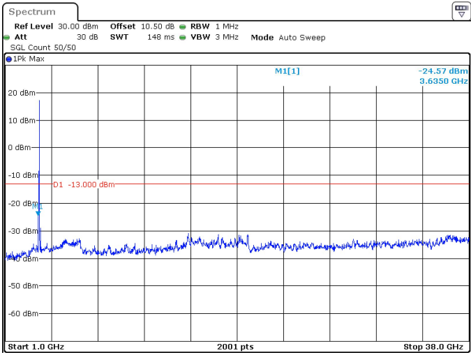
25MHz_15kHz_3712.5MHz_DFT-s-OFDM QPSK_RB128@0 -24.57 dBm
