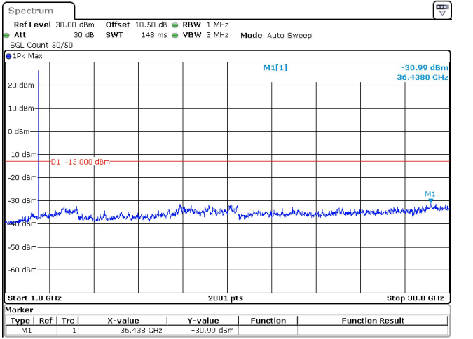
15MHz_30kHz_3792.5MHz_DFT-s-OFDM QPSK_RB1@0 -30.99 dBm
