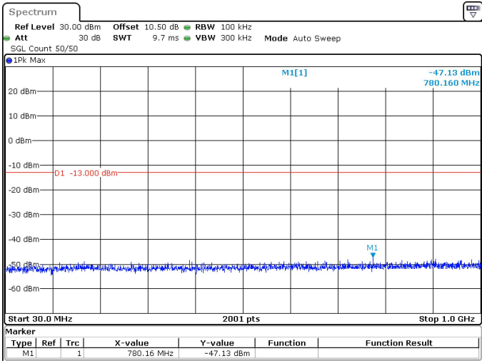
15MHz_30kHz_3750MHz_DFT-s-OFDM QPSK_RB36@0 -47.13 dBm
