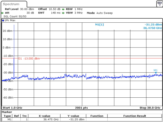
15MHz_30kHz_3792.5MHz_DFT-s-OFDM QPSK_RB1@37 -31.25 dBm
