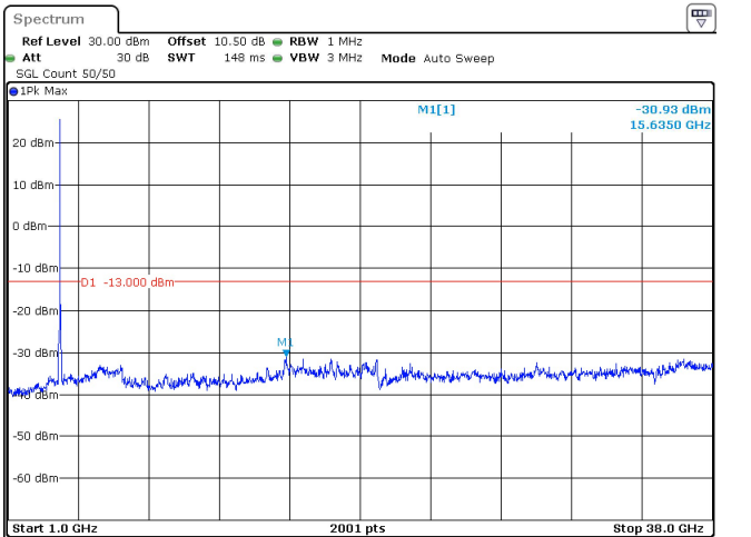
25MHz_15kHz_3750MHz_DFT-s-OFDM QPSK_RB1@0 -30.93 dBm
