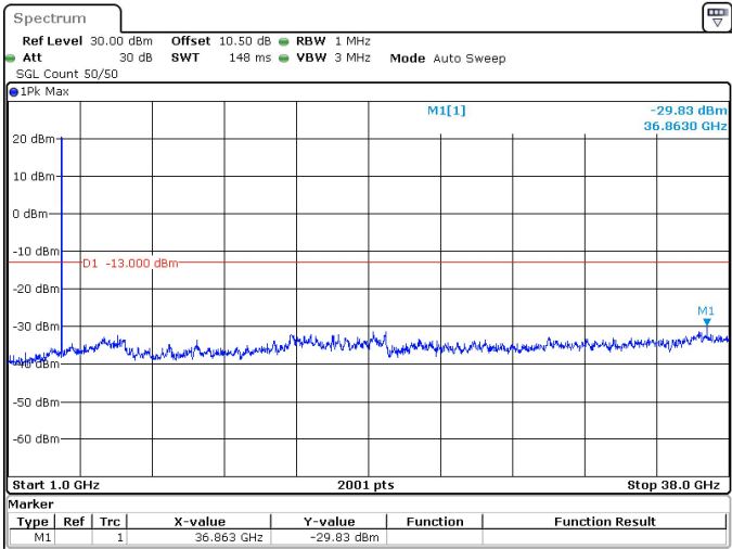
15MHz_30kHz_3750MHz_DFT-s-OFDM QPSK_RB36@0 -29.83 dBm
