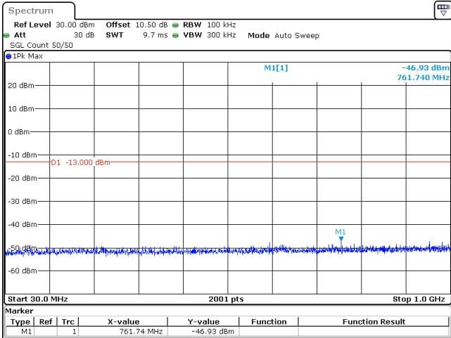
25MHz_15kHz_3787.5MHz_DFT-s-OFDM QPSK_RB1@0 -46.93 dBm
