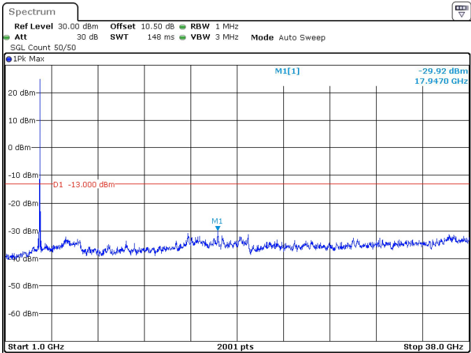
25MHz_15kHz_3750MHz_DFT-s-OFDM QPSK_RB1@132 -29.92 dBm
