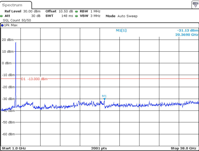
25MHz_15kHz_3787.5MHz_DFT-s-OFDM QPSK_RB128@0 -31.13 dBm
