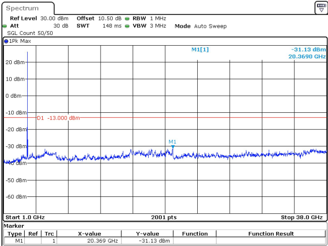
25MHz_30kHz_3712.5MHz_DFT-s-OFDM QPSK_RB1@64 -31.13 dBm
