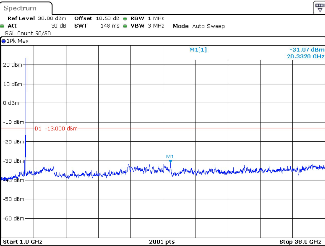
25MHz_15kHz_3787.5MHz_DFT-s-OFDM QPSK_RB1@132 -31.07 dBm
