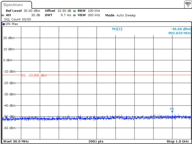
25MHz_15kHz_3750MHz_DFT-s-OFDM QPSK_RB128@0 -46.66 dBm
