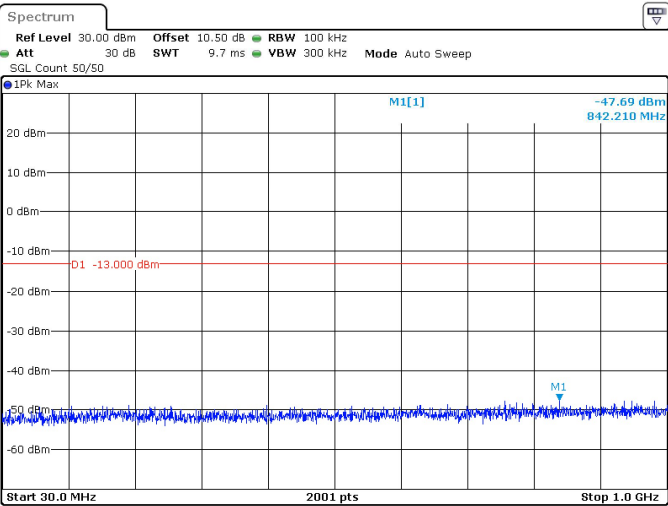
25MHz_15kHz_3787.5MHz_DFT-s-OFDM QPSK_RB1@132 -47.69 dBm
