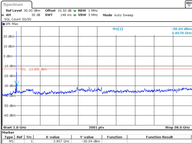
25MHz_15kHz_3787.5MHz_DFT-s-OFDM QPSK_RB1@0 -30.04 dBm
