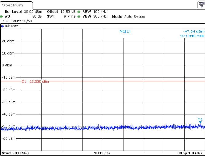
25MHz_15kHz_3787.5MHz_DFT-s-OFDM QPSK_RB128@0 -47.64 dBm
