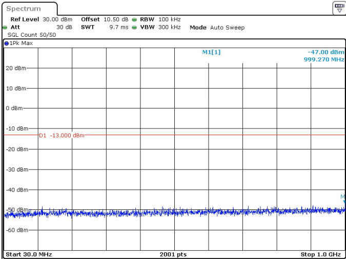
25MHz_15kHz_3750MHz_DFT-s-OFDM QPSK_RB1@132 -47.00 dBm
