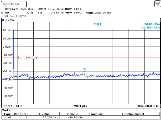
25MHz_30kHz_3712.5MHz_DFT-s-OFDM QPSK_RB64@0 -30.86 dBm
