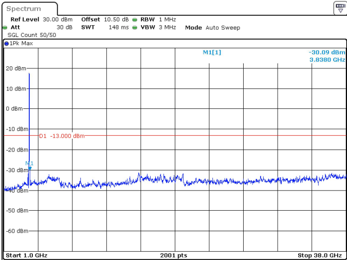
25MHz_15kHz_3750MHz_DFT-s-OFDM QPSK_RB128@0 -30.09 dBm
