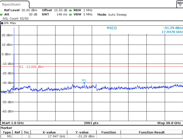
25MHz_30kHz_3712.5MHz_DFT-s-OFDM QPSK_RB1@0 -31.29 dBm
