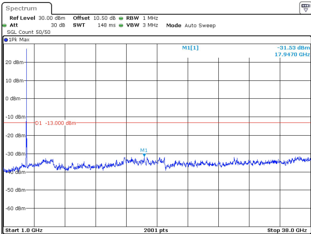
40MHz_15kHz_3780MHz_DFT-s-OFDM QPSK_RB1@0 -31.53 dBm
