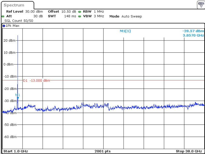
40MHz_15kHz_3780MHz_DFT-s-OFDM QPSK_RB1@215 -28.57 dBm
