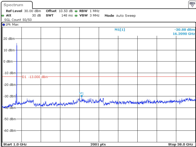
40MHz_15kHz_3780MHz_DFT-s-OFDM QPSK_RB216@0 -30.88 dBm
