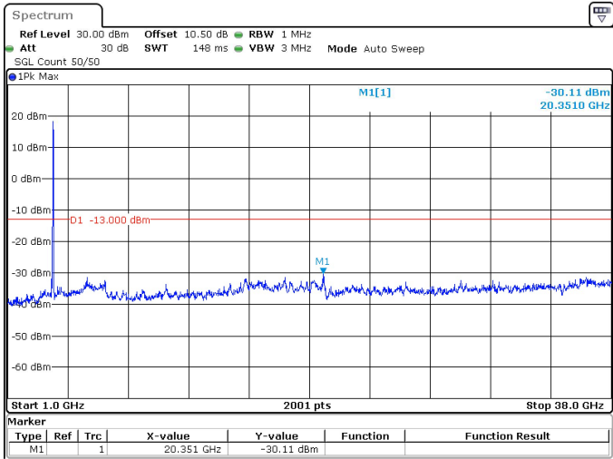
40MHz_30kHz_3780MHz_DFT-s-OFDM QPSK_RB100@0 -30.11 dBm
