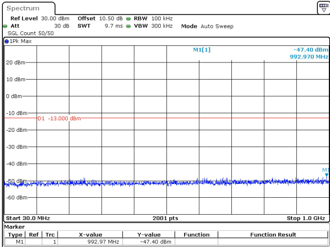
40MHz_30kHz_3780MHz_DFT-s-OFDM QPSK_RB1@105 -47.40 dBm
