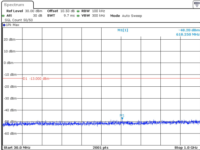
50MHz_15kHz_3725MHz_DFT-s-OFDM QPSK_RB1@0 -48.20 dBm
