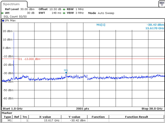
50MHz_15kHz_3725MHz_DFT-s-OFDM QPSK_RB270@0 -30.42 dBm
