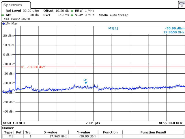
50MHz_15kHz_3750MHz_DFT-s-OFDM QPSK_RB1@0 -30.90 dBm
