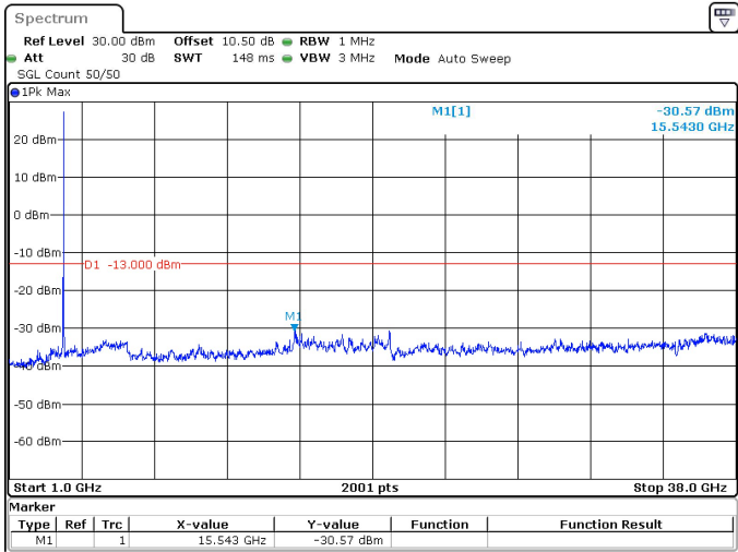
40MHz_30kHz_3750MHz_DFT-s-OFDM QPSK_RB1@105 -30.57 dBm
