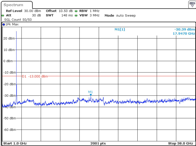
50MHz_15kHz_3725MHz_DFT-s-OFDM QPSK_RB1@269 -30.39 dBm
