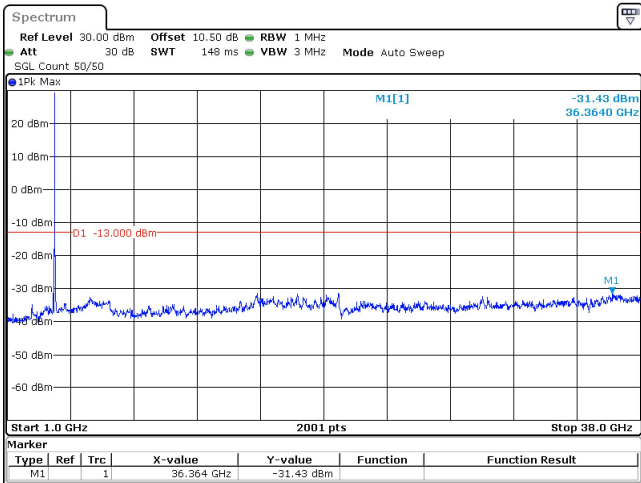
40MHz_30kHz_3780MHz_DFT-s-OFDM QPSK_RB1@0 -31.43 dBm
