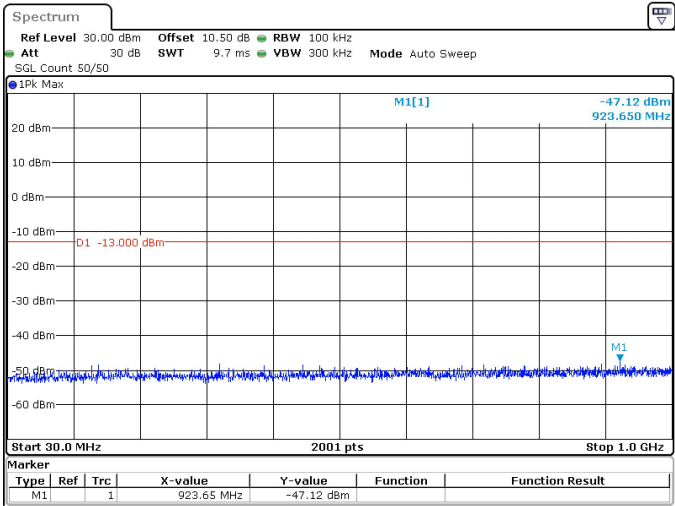
50MHz_30kHz_3775MHz_DFT-s-OFDM QPSK_RB128@0 -47.12 dBm
