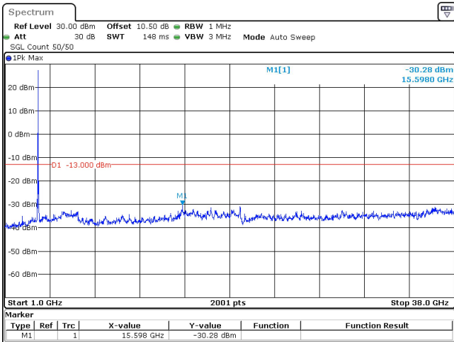
70MHz_30kHz_3735MHz_DFT-s-OFDM QPSK_RB1@0 -30.28 dBm
