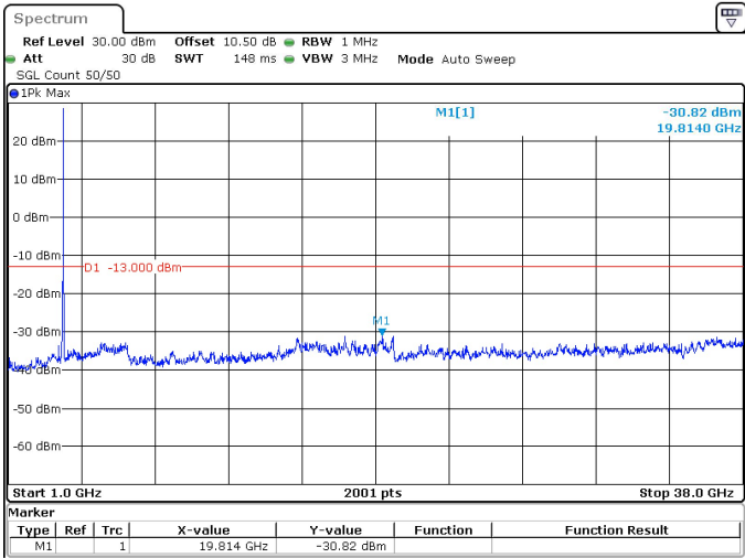
60MHz_30kHz_3750MHz_DFT-s-OFDM QPSK_RB1@161 -30.82 dBm
