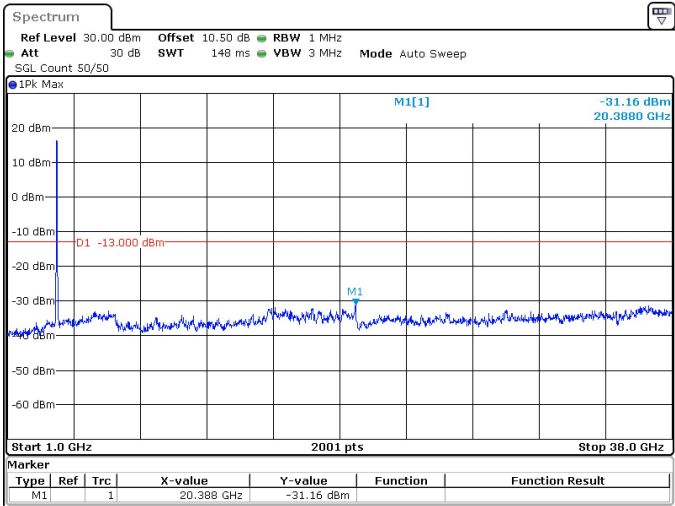
60MHz_30kHz_3750MHz_DFT-s-OFDM QPSK_RB162@0 -31.16 dBm
