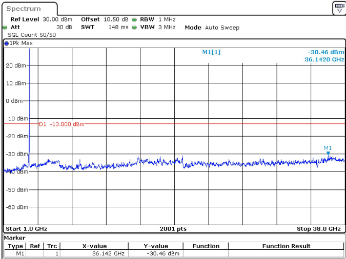
70MHz_30kHz_3735MHz_DFT-s-OFDM QPSK_RB1@188 -30.46 dBm
