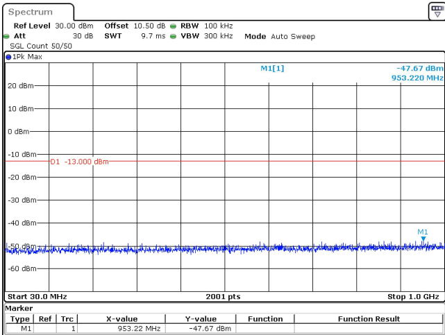
70MHz_30kHz_3735MHz_DFT-s-OFDM QPSK_RB1@0 -47.67 dBm
