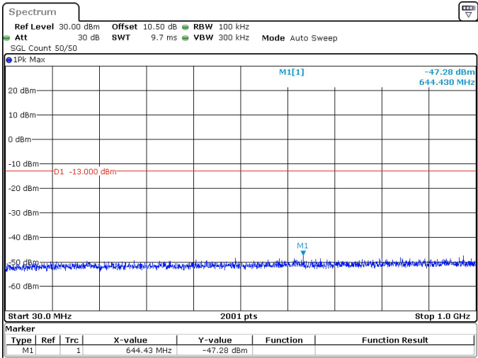
70MHz_30kHz_3735MHz_DFT-s-OFDM QPSK_RB1@188 -47.28 dBm
