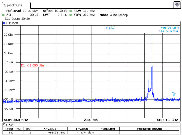
20MHz_15kHz_836.5MHz_DFT-s-OFDM QPSK_RB1@105&-46.74 dBm
