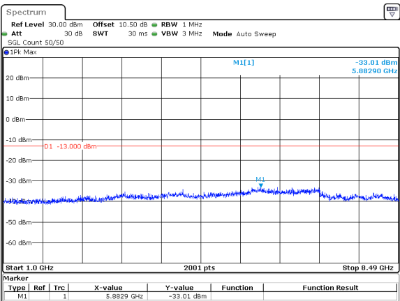
5MHz_15kHz_836.5MHz_DFT-s-OFDM QPSK_RB25@0&-33.01 dBm
