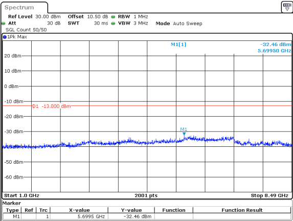
5MHz_15kHz_836.5MHz_DFT-s-OFDM QPSK_RB1@24&-32.46 dBm
