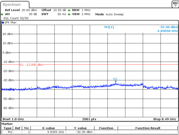
5MHz_15kHz_836.5MHz_DFT-s-OFDM QPSK_RB1@0&-32.30 dBm
