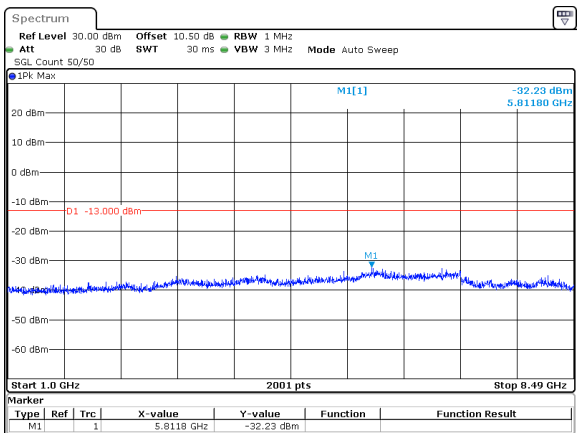
20MHz_15kHz_836.5MHz_DFT-s-OFDM QPSK_RB100@0&-32.23 dBm
