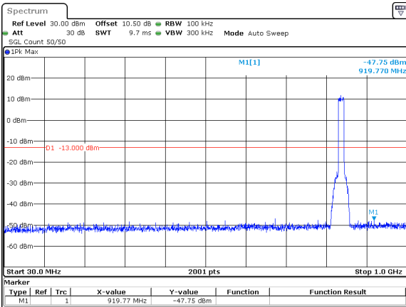
15MHz_15kHz_841.5MHz_DFT-s-OFDM QPSK_RB75@0&-47.75 dBm
