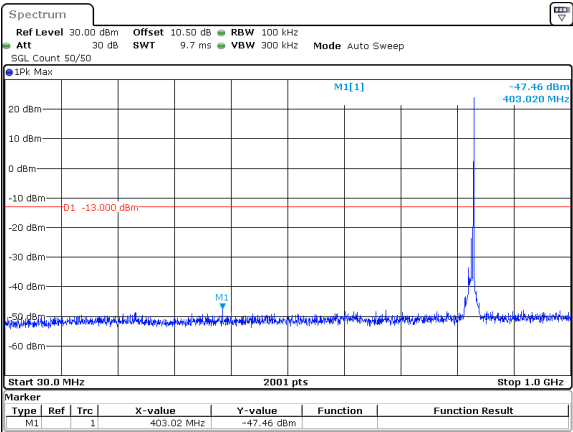
10MHz_15kHz_829MHz_DFT-s-OFDM QPSK_RB1@51&-47.46 dBm
