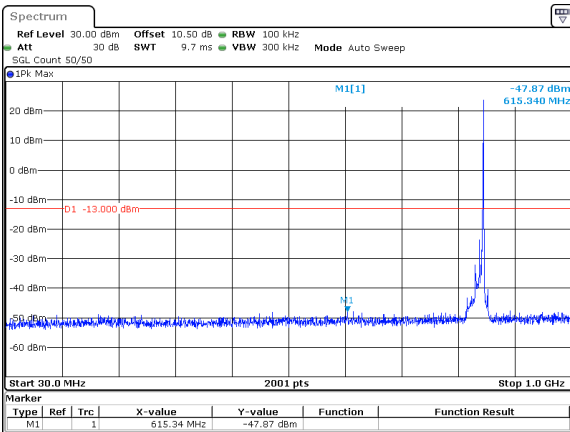
15MHz_15kHz_841.5MHz_DFT-s-OFDM QPSK_RB1@78&-47.87 dBm
