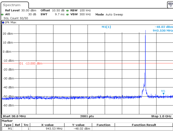
10MHz_15kHz_836.5MHz_DFT-s-OFDM QPSK_RB1@51&-48.02 dBm
