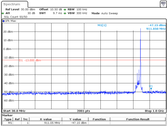
20MHz_15kHz_839MHz_DFT-s-OFDM QPSK_RB1@105&-47.15 dBm
