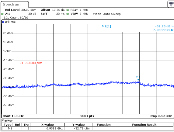
15MHz_15kHz_831.5MHz_DFT-s-OFDM QPSK_RB1@0&-32.73 dBm
