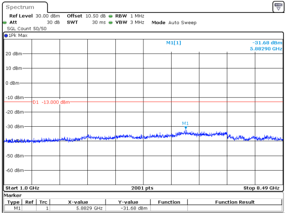
20MHz_15kHz_836.5MHz_DFT-s-OFDM QPSK_RB1@0&-31.68 dBm
