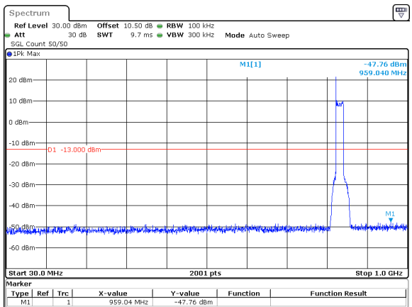
20MHz_15kHz_836.5MHz_DFT-s-OFDM QPSK_RB100@0&-47.76 dBm
