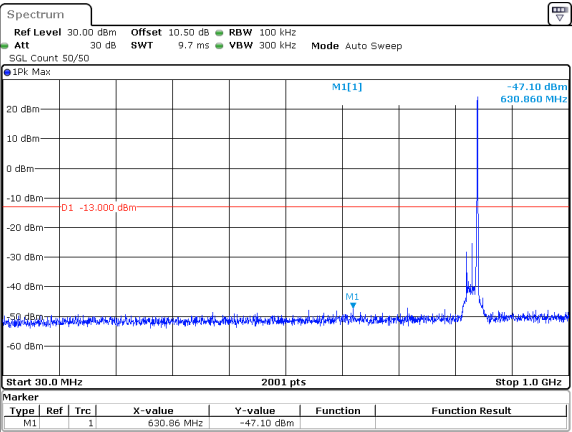
20MHz_15kHz_834MHz_DFT-s-OFDM QPSK_RB1@105&-47.10 dBm
