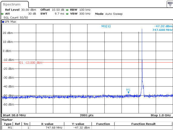
5MHz_15kHz_826.5MHz_DFT-s-OFDM QPSK_RB1@0&-47.32 dBm
