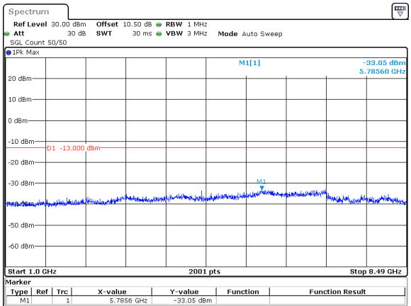
20MHz_15kHz_836.5MHz_DFT-s-OFDM QPSK_RB1@105&-33.05 dBm
