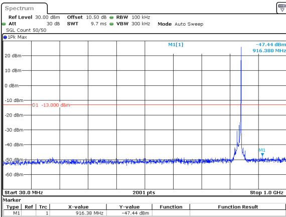
15MHz_15kHz_836.5MHz_DFT-s-OFDM QPSK_RB1@78&-47.44 dBm
