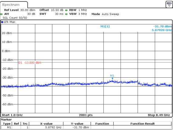
20MHz_15kHz_834MHz_DFT-s-OFDM QPSK_RB100@0&-31.70 dBm
