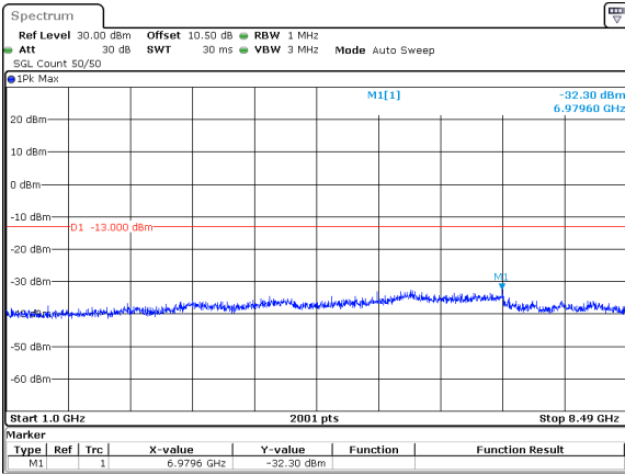
15MHz_15kHz_836.5MHz_DFT-s-OFDM QPSK_RB1@0&-32.30 dBm
