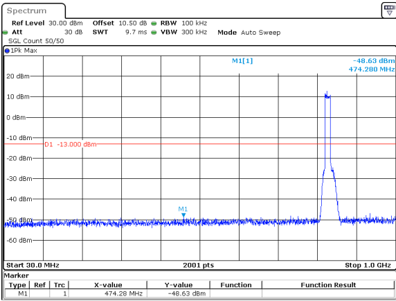
15MHz_15kHz_831.5MHz_DFT-s-OFDM QPSK_RB75@0&-48.63 dBm
