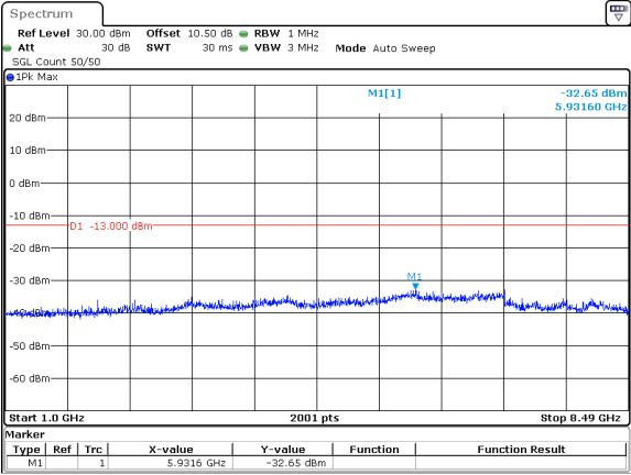
5MHz_15kHz_846.5MHz_DFT-s-OFDM QPSK_RB1@24&-32.65 dBm
