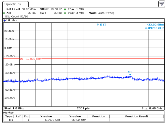
20MHz_15kHz_839MHz_DFT-s-OFDM QPSK_RB1@105&-33.02 dBm
