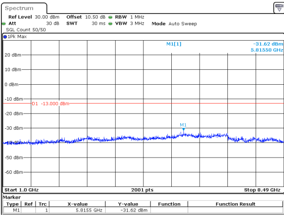
15MHz_15kHz_831.5MHz_DFT-s-OFDM QPSK_RB1@78&-31.62 dBm
