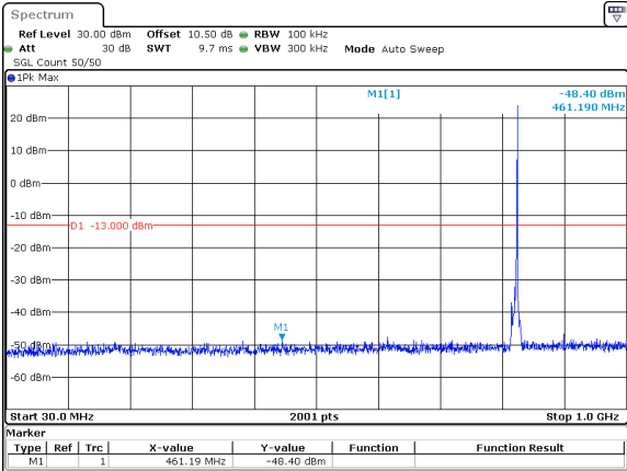
5MHz_15kHz_826.5MHz_DFT-s-OFDM QPSK_RB1@24&-48.40 dBm
