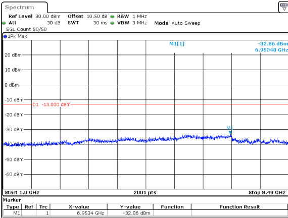
15MHz_15kHz_841.5MHz_DFT-s-OFDM QPSK_RB1@0&-32.86 dBm
