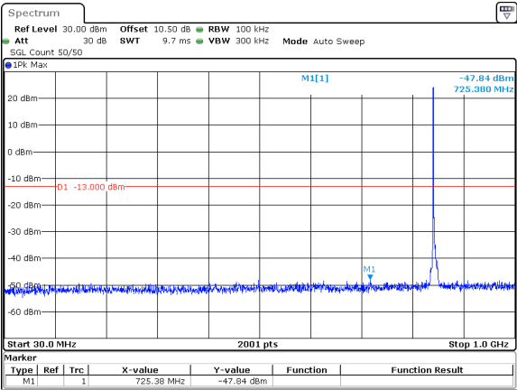
5MHz_15kHz_846.5MHz_DFT-s-OFDM QPSK_RB1@0&-47.84 dBm
