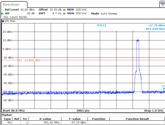
15MHz_15kHz_836.5MHz_DFT-s-OFDM QPSK_RB75@0&-47.70 dBm
