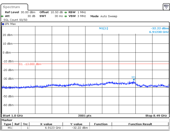
10MHz_15kHz_844MHz_DFT-s-OFDM QPSK_RB1@51&-32.22 dBm
