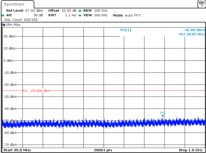
15MHz_30kHz_2595MHz_DFT-s-OFDM QPSK_RB36@0 -46.80 dBm
