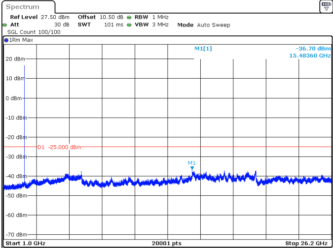
15MHz_30kHz_2595MHz_DFT-s-OFDM QPSK_RB1@37 -36.70 dBm
