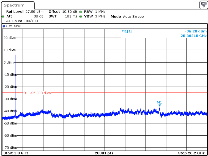
25MHz_30kHz_2582.5MHz_DFT-s-OFDM QPSK_RB64@0 -36.28 dBm
