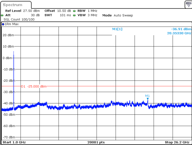
40MHz_30kHz_2595MHz_DFT-s-OFDM QPSK_RB100@0 -36.91 dBm
