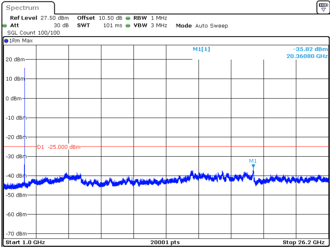
30MHz_30kHz_2605MHz_DFT-s-OFDM QPSK_RB1@77 -35.82 dBm
