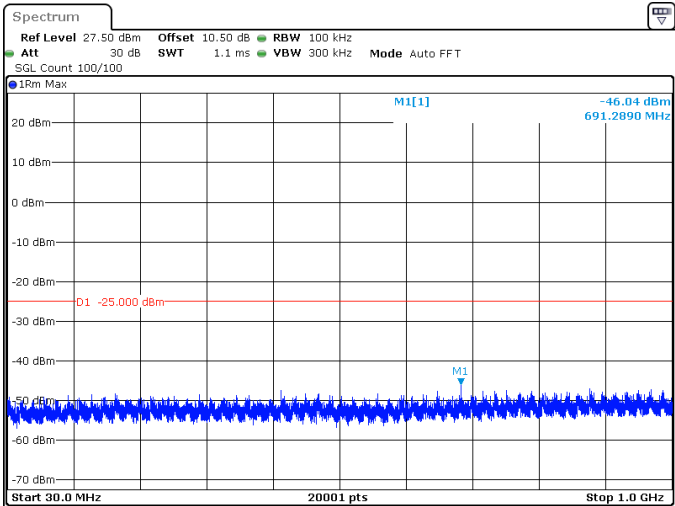
25MHz_30kHz_2582.5MHz_DFT-s-OFDM QPSK_RB1@0 -46.04 dBm
