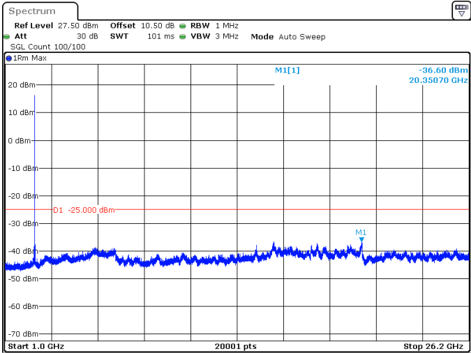
25MHz_30kHz_2582.5MHz_DFT-s-OFDM QPSK_RB1@64 -36.60 dBm
