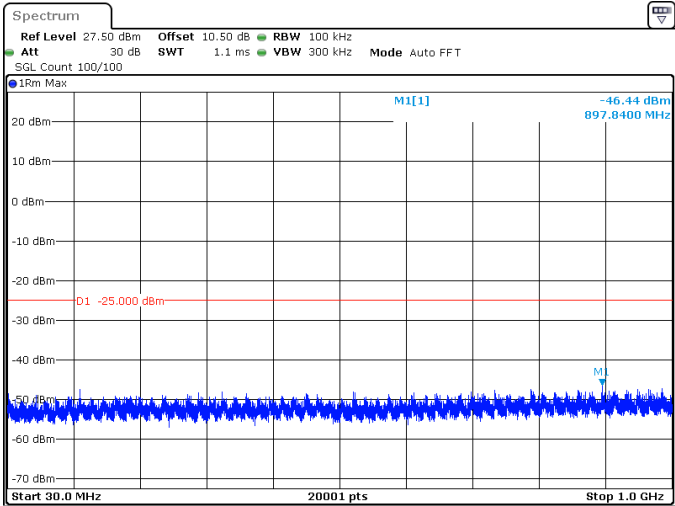
40MHz_30kHz_2590MHz_DFT-s-OFDM QPSK_RB1@105 -46.44 dBm
