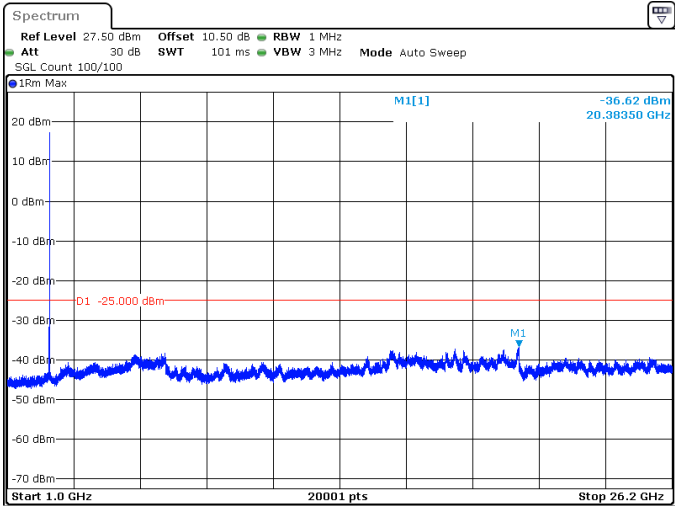
15MHz_30kHz_2577.5MHz_DFT-s-OFDM QPSK_RB1@37 -36.62 dBm
