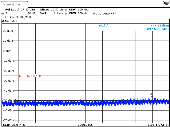
15MHz_30kHz_2577.5MHz_DFT-s-OFDM QPSK_RB1@0 -47.13 dBm
