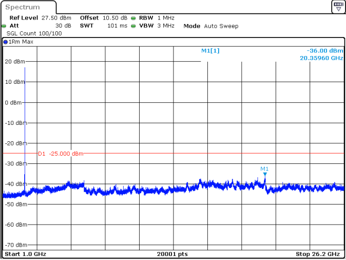
15MHz_30kHz_2612.5MHz_DFT-s-OFDM QPSK_RB1@37 -36.00 dBm
