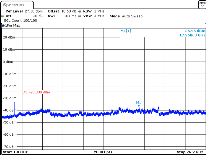
40MHz_30kHz_2600MHz_DFT-s-OFDM QPSK_RB1@105 -36.96 dBm
