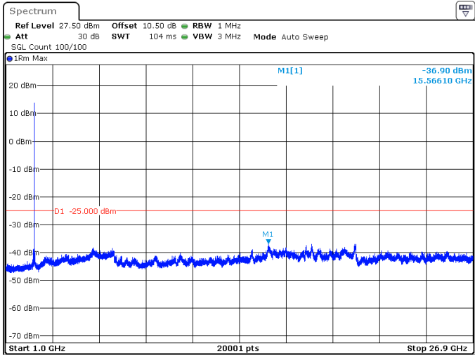
80MHz_30kHz_2536.02MHz_DFT-s-OFDM QPSK_RB1@216 -36.90 dBm
