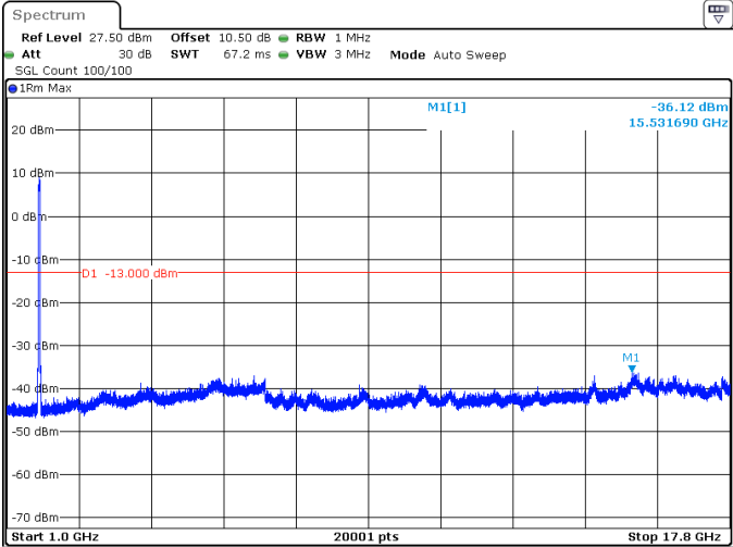
25MHz_15kHz_1745MHz_DFT-s-OFDM QPSK_RB128@0 -36.12 dBm
