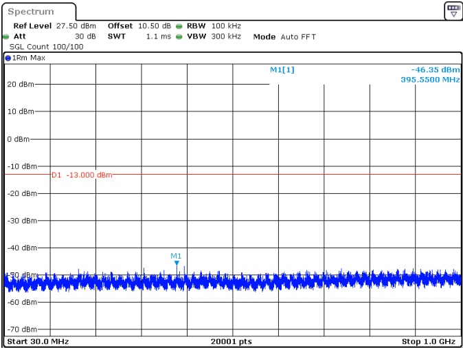
10MHz_30kHz_3545MHz_DFT-s-OFDM QPSK_RB24@0 -46.35 dBm
