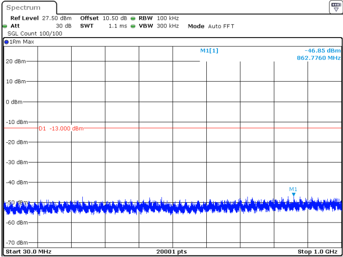
5MHz_15kHz_1712.5MHz_DFT-s-OFDM QPSK_RB1@0 -46.85 dBm
