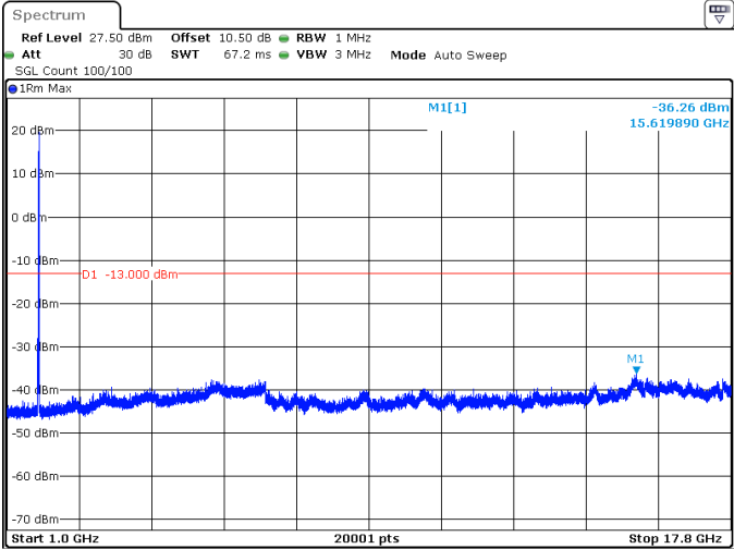
25MHz_15kHz_1722.5MHz_DFT-s-OFDM QPSK_RB1@132 -36.26 dBm
