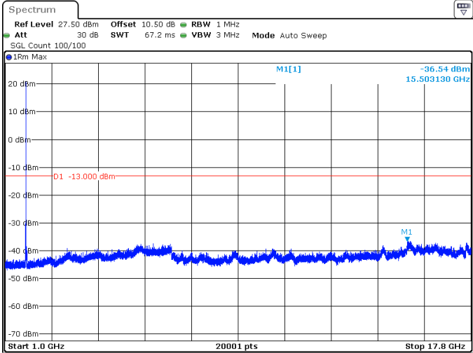
15MHz_15kHz_1745MHz_DFT-s-OFDM QPSK_RB1@78 -36.54 dBm
