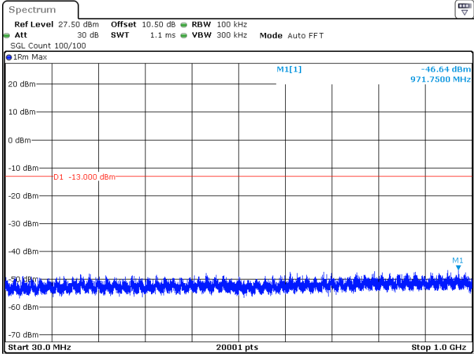
25MHz_15kHz_1767.5MHz_DFT-s-OFDM QPSK_RB1@132 -46.64 dBm
