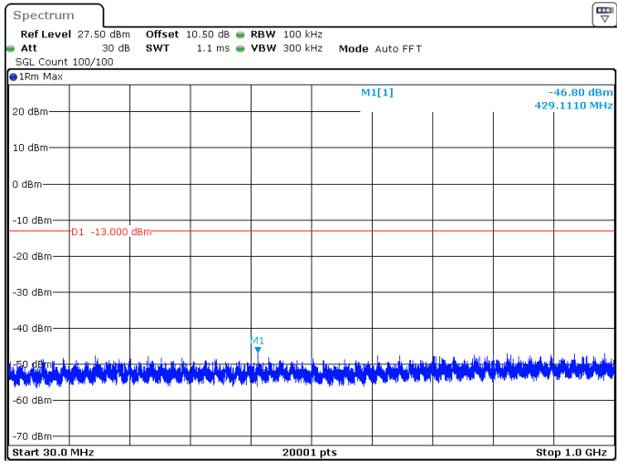
20MHz_15kHz_1745MHz_DFT-s-OFDM QPSK_RB100@0 -46.80 dBm
