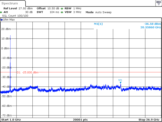
100MHz_30kHz_2546.01MHz_DFT-s-OFDM QPSK_RB1@272 -36.58 dBm
