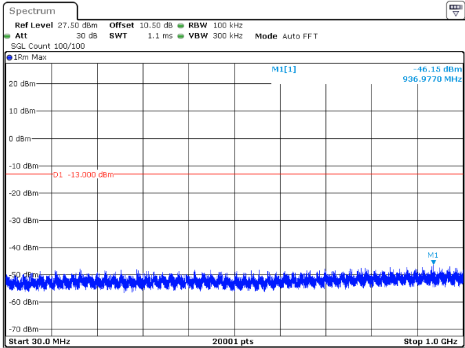
15MHz_15kHz_1717.5MHz_DFT-s-OFDM QPSK_RB1@78 -46.15 dBm
