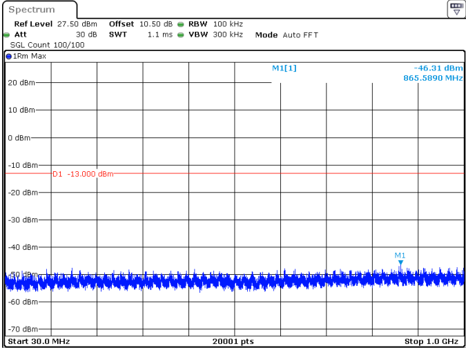
10MHz_15kHz_1775MHz_DFT-s-OFDM QPSK_RB1@51 -46.31 dBm
