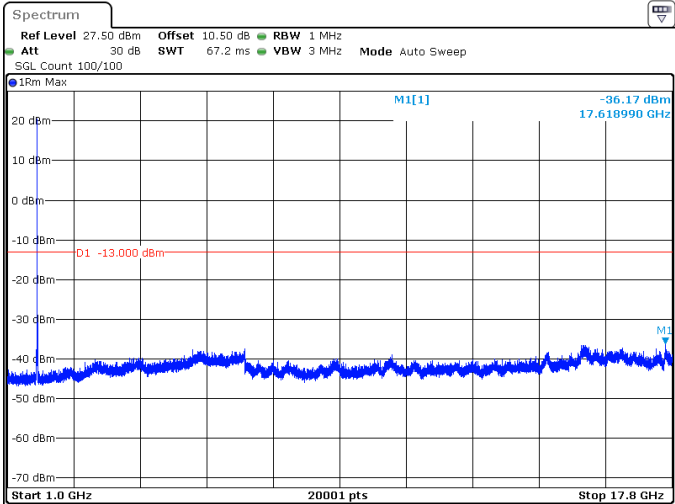
15MHz_15kHz_1745MHz_DFT-s-OFDM QPSK_RB1@0 -36.17 dBm
