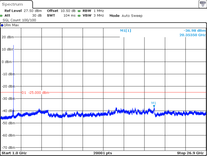
100MHz_30kHz_2592.99MHz_DFT-s-OFDM QPSK_RB1@272 -36.98 dBm
