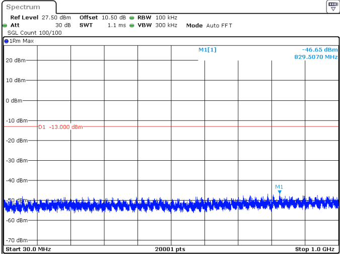
30MHz_15kHz_1745MHz_DFT-s-OFDM QPSK_RB1@159 -46.65 dBm
