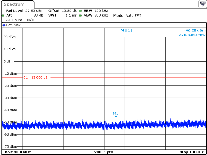
20MHz_15kHz_1770MHz_DFT-s-OFDM QPSK_RB1@105 -46.20 dBm
