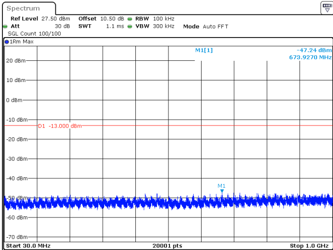
5MHz_15kHz_1777.5MHz_DFT-s-OFDM QPSK_RB1@0 -47.24 dBm
