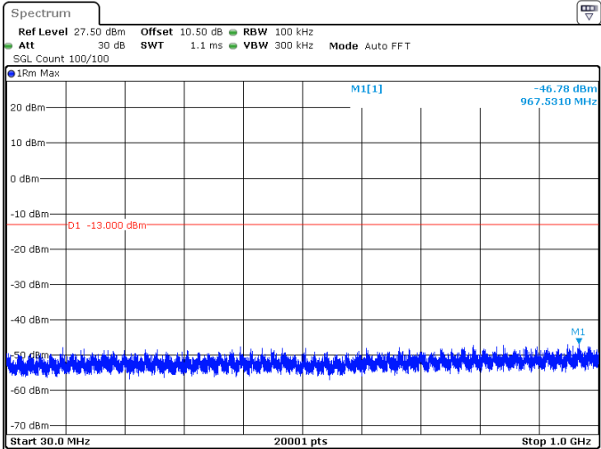
10MHz_15kHz_1745MHz_DFT-s-OFDM QPSK_RB1@0 -46.78 dBm
