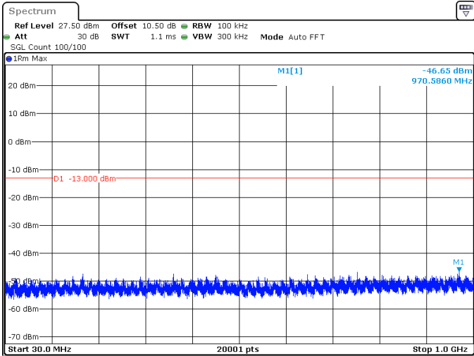
15MHz_30kHz_3542.5MHz_DFT-s-OFDM QPSK_RB1@37 -46.65 dBm
