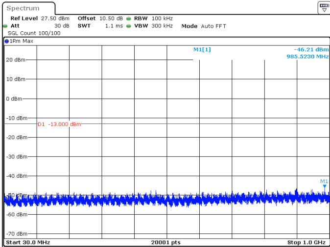
5MHz_15kHz_1777.5MHz_DFT-s-OFDM QPSK_RB25@0 -46.21 dBm
