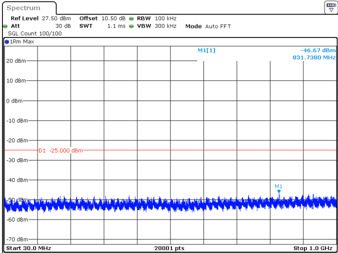
90MHz_30kHz_2592.99MHz_DFT-s-OFDM QPSK_RB1@244 -46.67 dBm
