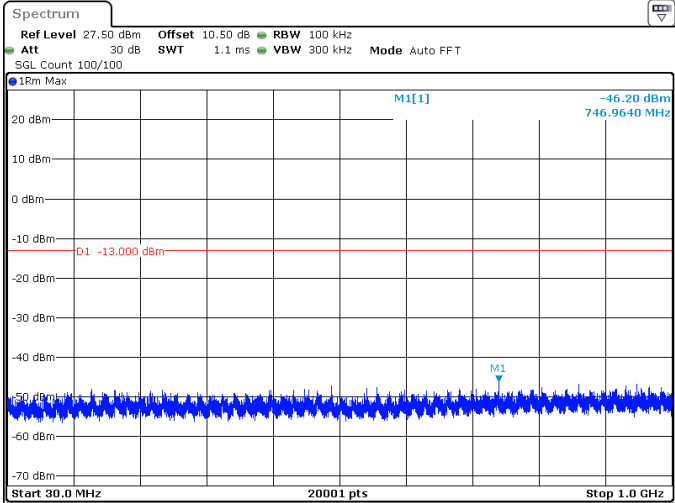
30MHz_15kHz_1745MHz_DFT-s-OFDM QPSK_RB160@0 -46.20 dBm
