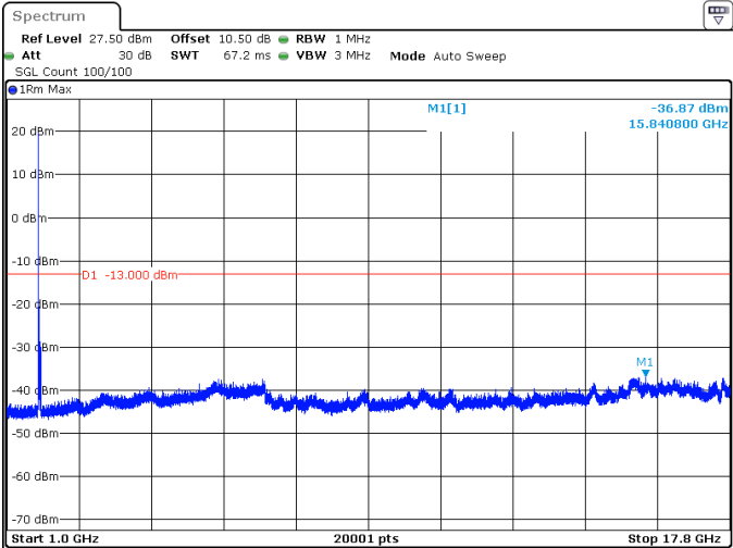
30MHz_15kHz_1745MHz_DFT-s-OFDM QPSK_RB1@0 -36.87 dBm
