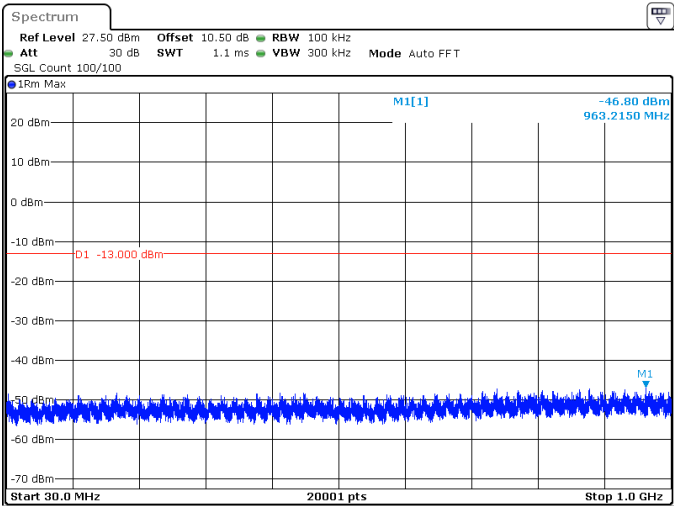
30MHz_15kHz_1765MHz_DFT-s-OFDM QPSK_RB160@0 -46.80 dBm
