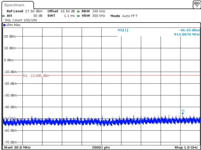
15MHz_30kHz_3500MHz_DFT-s-OFDM QPSK_RB1@0 -46.45 dBm
