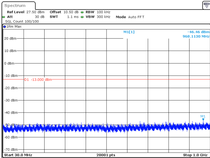
10MHz_30kHz_3500MHz_DFT-s-OFDM QPSK_RB1@23 -46.46 dBm
