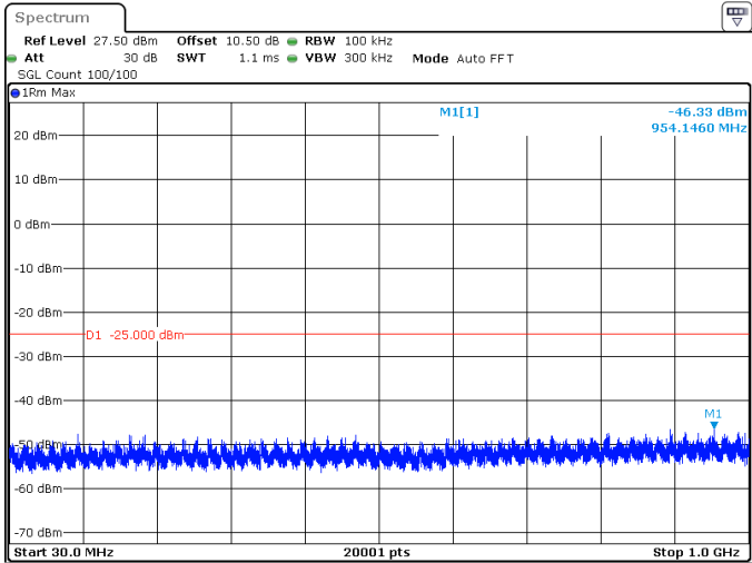
80MHz_30kHz_2536.02MHz_DFT-s-OFDM QPSK_RB1@216 -46.33 dBm
