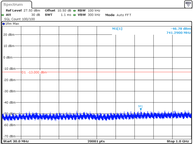
15MHz_30kHz_3500MHz_DFT-s-OFDM QPSK_RB1@37 -46.78 dBm
