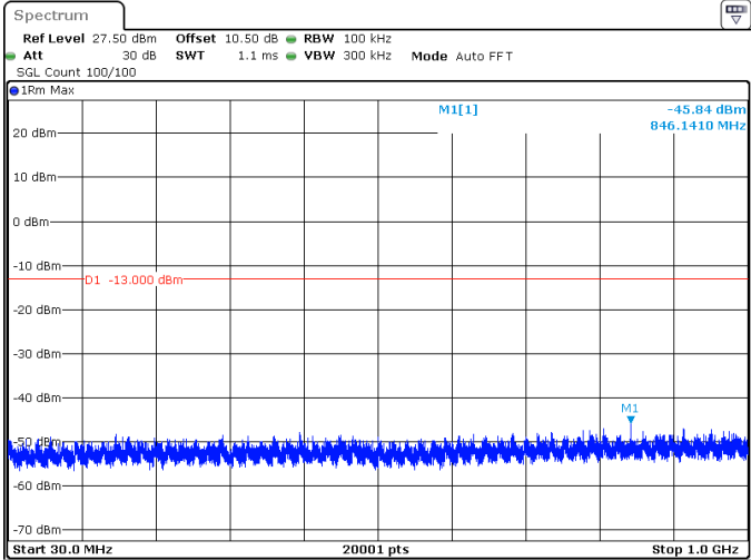
5MHz_15kHz_1745MHz_DFT-s-OFDM QPSK_RB25@0 -45.84 dBm
