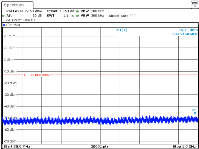
15MHz_15kHz_1772.5MHz_DFT-s-OFDM QPSK_RB1@0 -46.73 dBm
