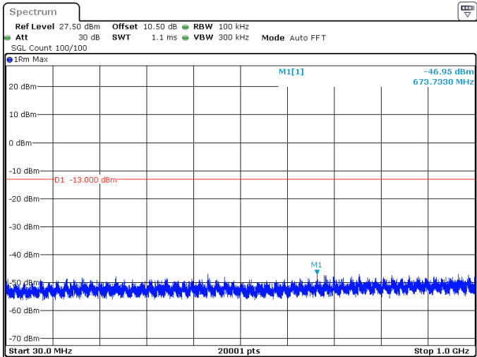
15MHz_15kHz_1717.5MHz_DFT-s-OFDM QPSK_RB1@0 -46.95 dBm
