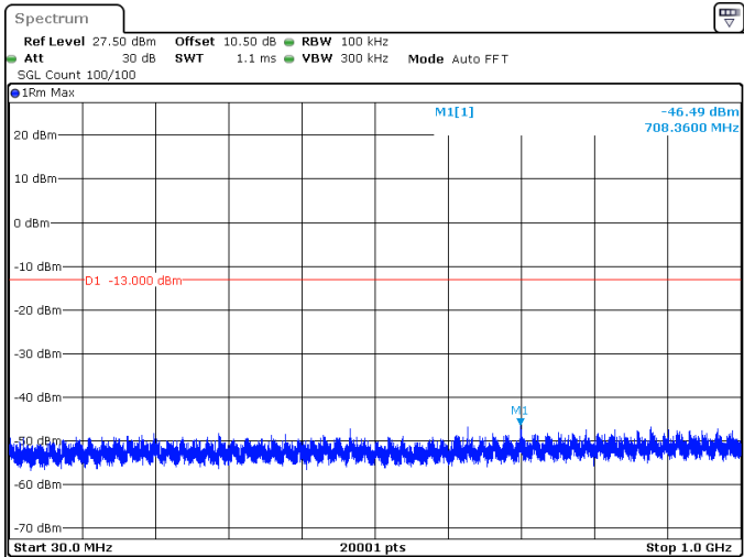
15MHz_30kHz_3457.5MHz_DFT-s-OFDM QPSK_RB1@0 -46.49 dBm
