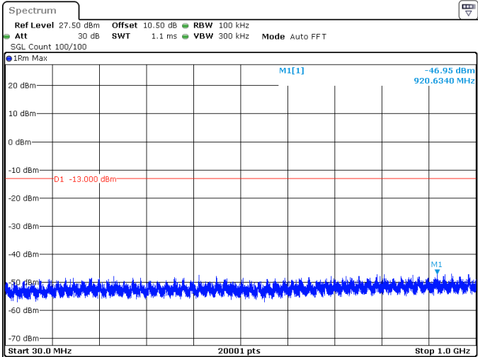
30MHz_15kHz_1745MHz_DFT-s-OFDM QPSK_RB1@0 -46.95 dBm
