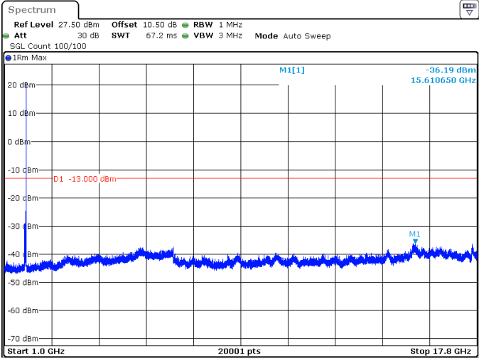
30MHz_15kHz_1745MHz_DFT-s-OFDM QPSK_RB1@159 -36.19 dBm
