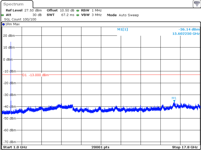
5MHz_15kHz_1745MHz_DFT-s-OFDM QPSK_RB25@0 -36.14 dBm
