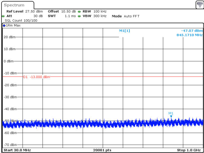
15MHz_30kHz_3457.5MHz_DFT-s-OFDM QPSK_RB36@0 -47.07 dBm
