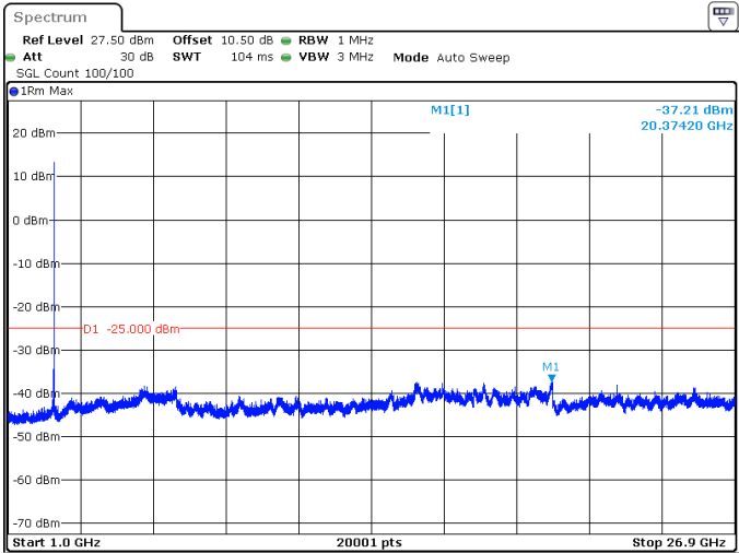
90MHz_30kHz_2592.99MHz_DFT-s-OFDM QPSK_RB1@244 -37.21 dBm
