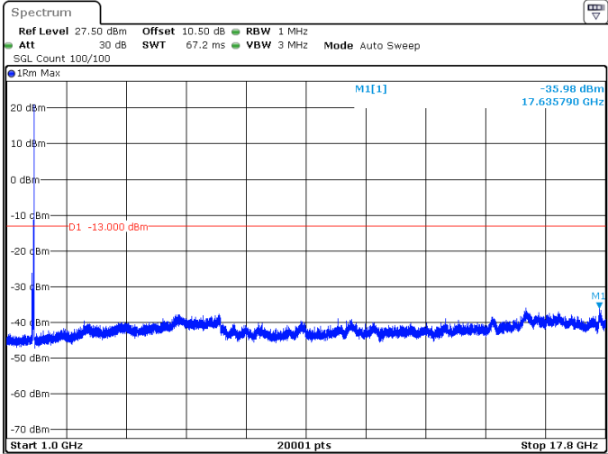
25MHz_15kHz_1745MHz_DFT-s-OFDM QPSK_RB1@132 -35.98 dBm
