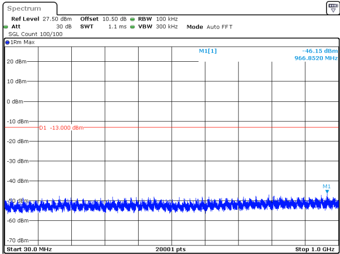
15MHz_30kHz_3500MHz_DFT-s-OFDM QPSK_RB36@0 -46.15 dBm
