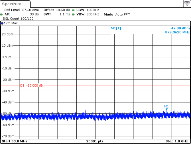
100MHz_30kHz_2592.99MHz_DFT-s-OFDM QPSK_RB1@272 -47.08 dBm
