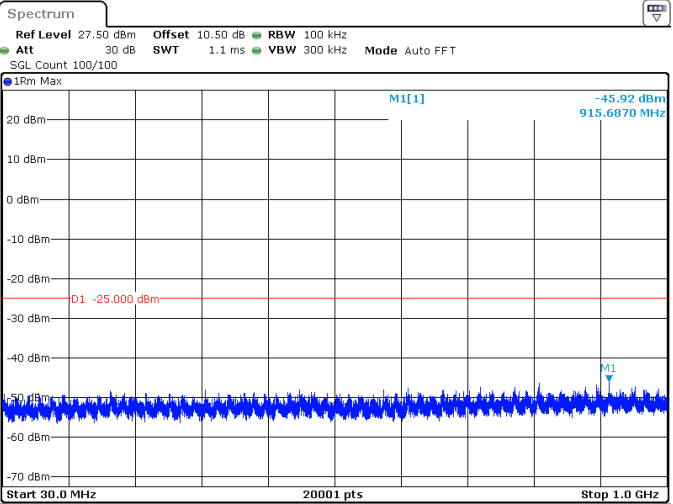
100MHz_30kHz_2546.01MHz_DFT-s-OFDM QPSK_RB1@272 -45.92 dBm
