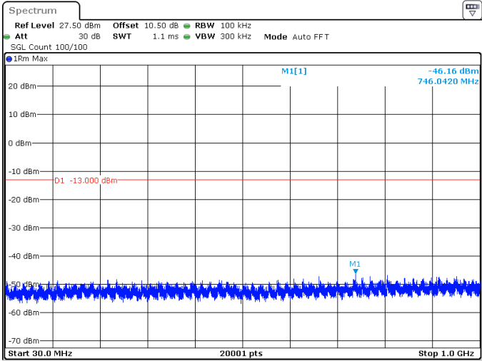
40MHz_15kHz_1760MHz_DFT-s-OFDM QPSK_RB1@0 -46.16 dBm
