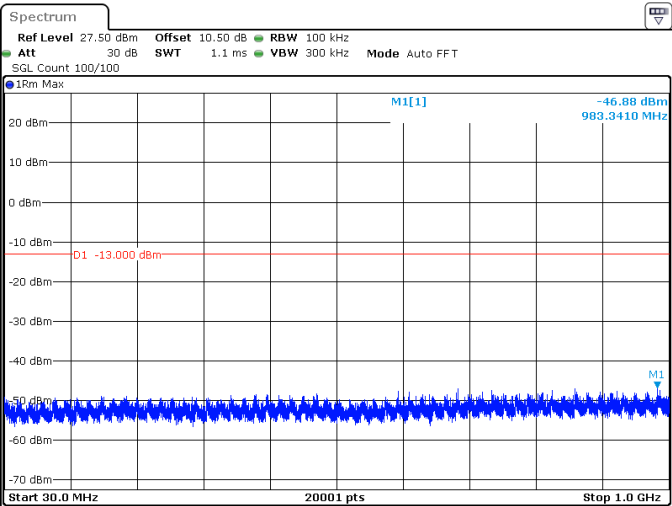
40MHz_15kHz_1730MHz_DFT-s-OFDM QPSK_RB1@0 -46.88 dBm
