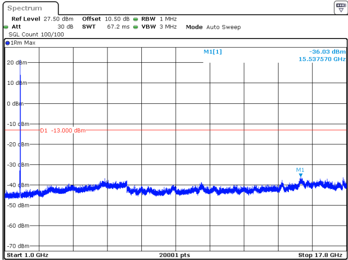
20MHz_15kHz_1745MHz_DFT-s-OFDM QPSK_RB1@105 -36.03 dBm
