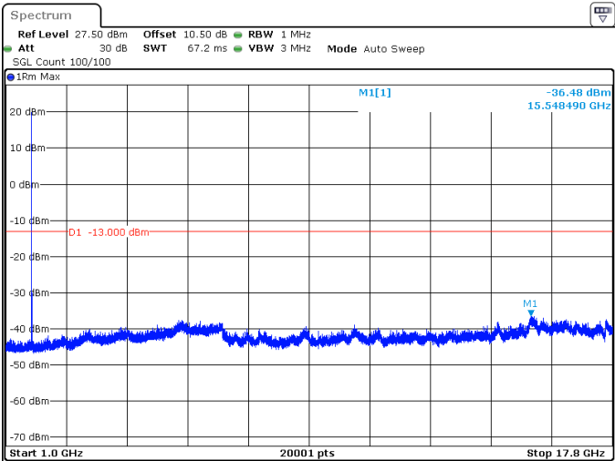
5MHz_15kHz_1712.5MHz_DFT-s-OFDM QPSK_RB1@0 -36.48 dBm
