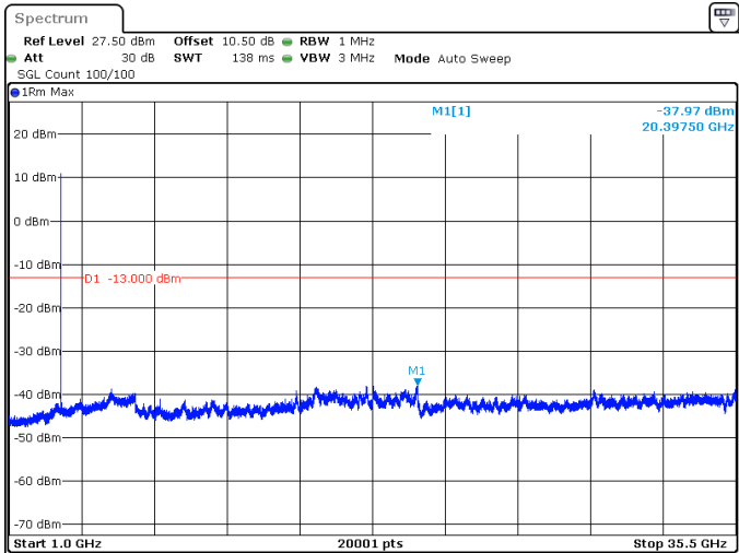
15MHz_30kHz_3457.5MHz_DFT-s-OFDM QPSK_RB1@0 -37.97 dBm
