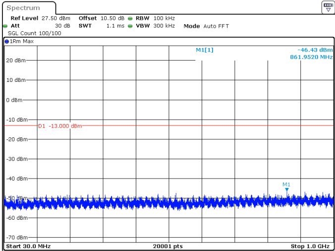
15MHz_15kHz_1772.5MHz_DFT-s-OFDM QPSK_RB1@78 -46.43 dBm
