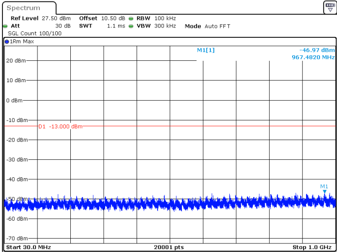
15MHz_30kHz_3457.5MHz_DFT-s-OFDM QPSK_RB1@37 -46.97 dBm
