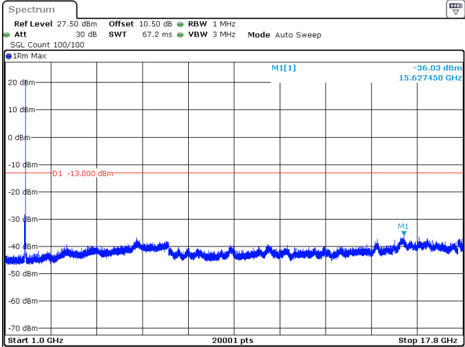
30MHz_15kHz_1725MHz_DFT-s-OFDM QPSK_RB1@159 -36.03 dBm
