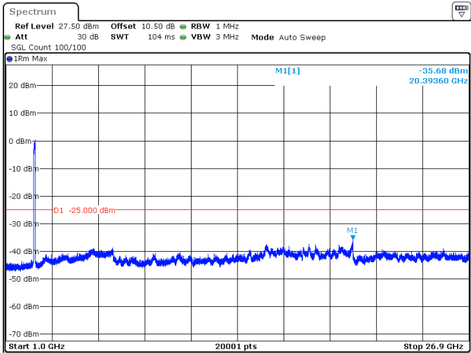
80MHz_30kHz_2592.99MHz_DFT-s-OFDM QPSK_RB216@0 -35.68 dBm
