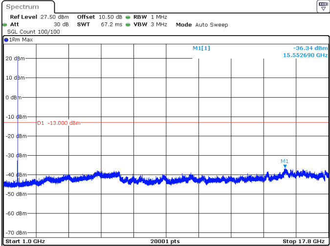
10MHz_15kHz_1715MHz_DFT-s-OFDM QPSK_RB1@51 -36.34 dBm
