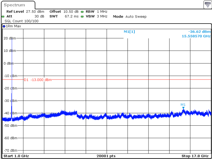
40MHz_15kHz_1745MHz_DFT-s-OFDM QPSK_RB1@215 -36.62 dBm
