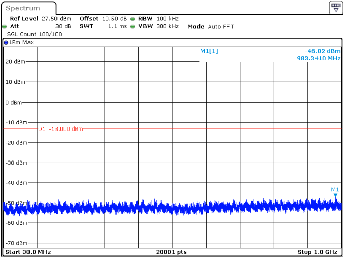
40MHz_15kHz_1745MHz_DFT-s-OFDM QPSK_RB1@215 -46.82 dBm
