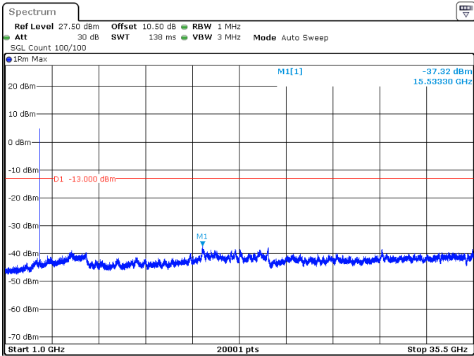
15MHz_30kHz_3542.5MHz_DFT-s-OFDM QPSK_RB36@0 -37.32 dBm
