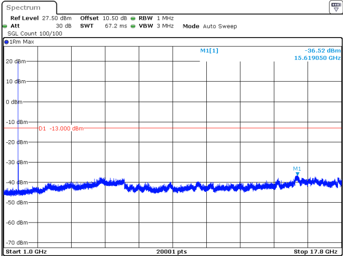
10MHz_15kHz_1715MHz_DFT-s-OFDM QPSK_RB1@0 -36.52 dBm
