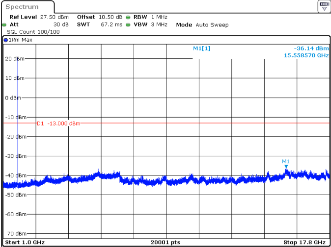
5MHz_15kHz_1745MHz_DFT-s-OFDM QPSK_RB1@24 -36.14 dBm
