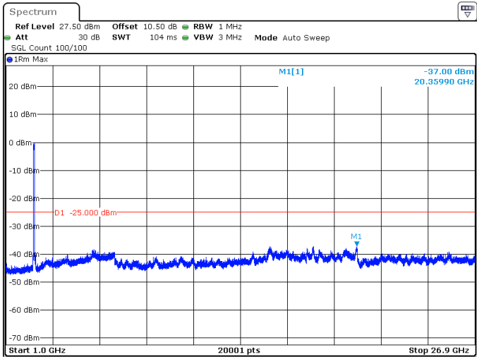
80MHz_30kHz_2536.02MHz_DFT-s-OFDM QPSK_RB216@0 -37.00 dBm
