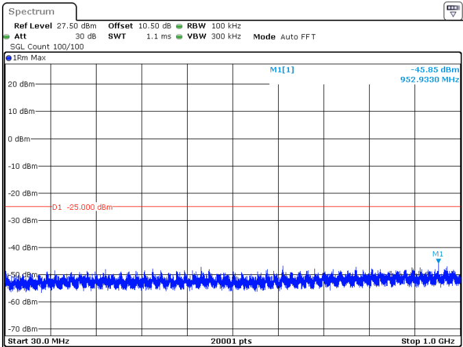
90MHz_30kHz_2592.99MHz_DFT-s-OFDM QPSK_RB1@0 -45.85 dBm
