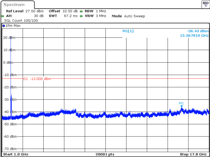
25MHz_15kHz_1722.5MHz_DFT-s-OFDM QPSK_RB1@0 -36.43 dBm
