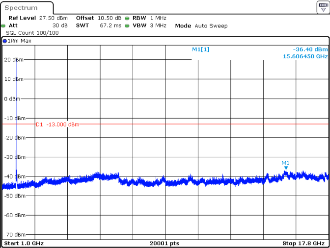
40MHz_15kHz_1730MHz_DFT-s-OFDM QPSK_RB1@215 -36.40 dBm
