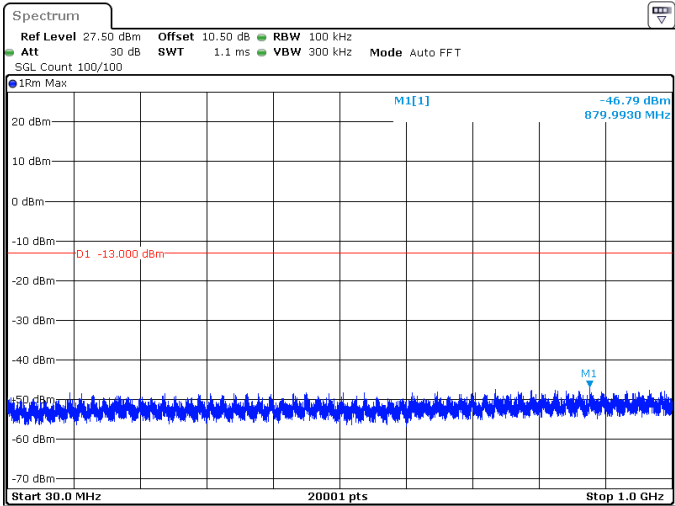
40MHz_30kHz_3530MHz_DFT-s-OFDM QPSK_RB1@105 -46.79 dBm
