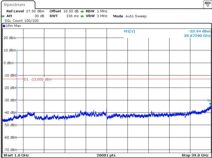
15MHz_30kHz_3707.5MHz_DFT-s-OFDM QPSK_RB1@0 -33.94 dBm
