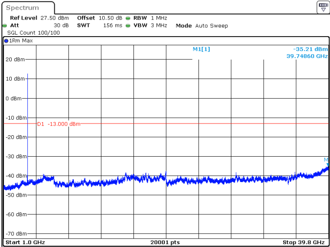
10MHz_15kHz_3840MHz_DFT-s-OFDM QPSK_RB1@51 -35.21 dBm
