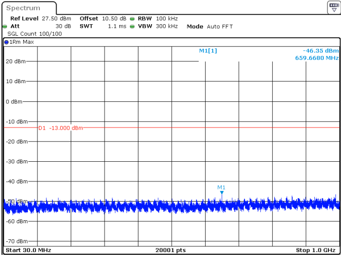
90MHz_30kHz_3505MHz_DFT-s-OFDM QPSK_RB1@244 -46.35 dBm
