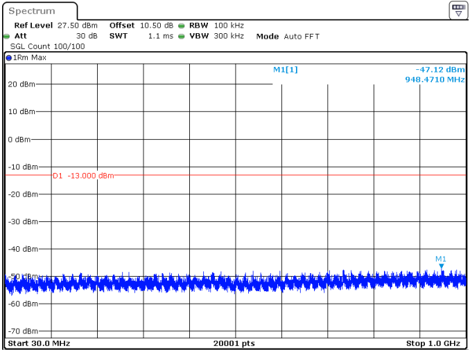
50MHz_30kHz_3525MHz_DFT-s-OFDM QPSK_RB1@132 -47.12 dBm
