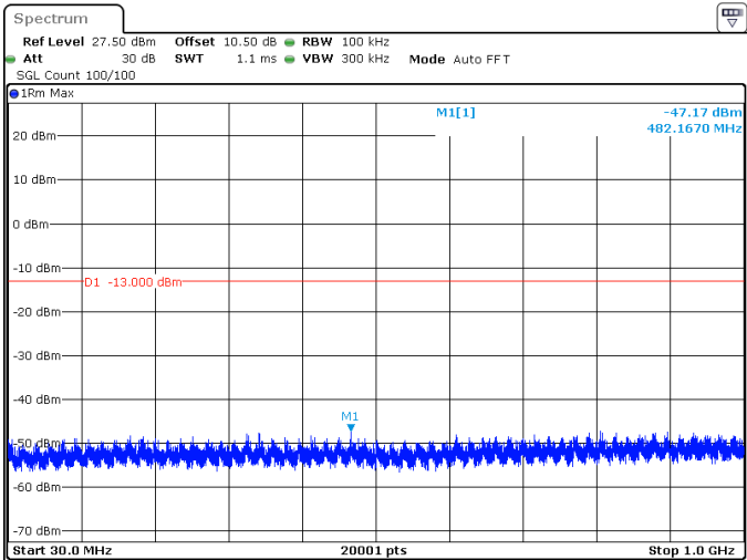
70MHz_30kHz_3515MHz_DFT-s-OFDM QPSK_RB1@0 -47.17 dBm
