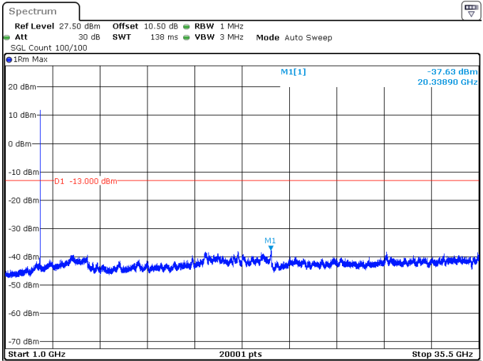
50MHz_30kHz_3500MHz_DFT-s-OFDM QPSK_RB1@132 -37.63 dBm
