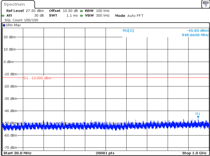
15MHz_30kHz_3840MHz_DFT-s-OFDM QPSK_RB36@0 -45.85 dBm
