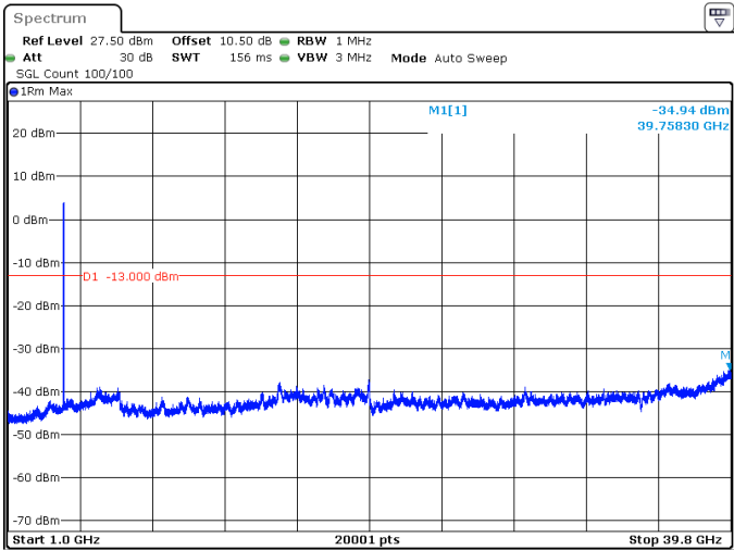
15MHz_15kHz_3972.5MHz_DFT-s-OFDM QPSK_RB75@0 -34.94 dBm
