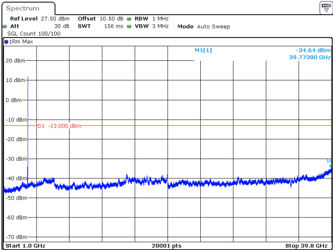
10MHz_15kHz_3840MHz_DFT-s-OFDM QPSK_RB1@0 -34.64 dBm
