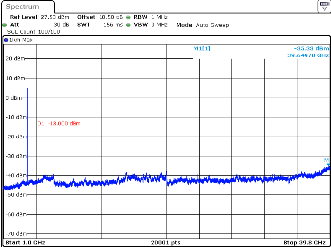
15MHz_15kHz_3840MHz_DFT-s-OFDM QPSK_RB75@0 -35.33 dBm
