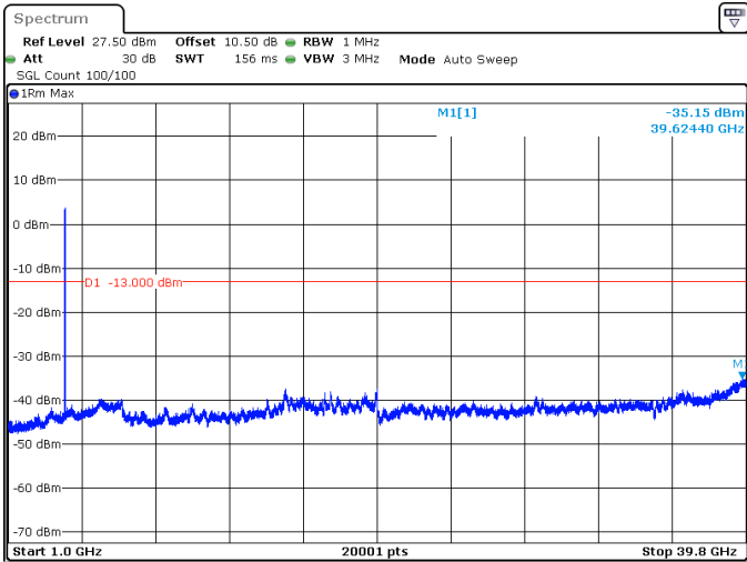
15MHz_30kHz_3972.5MHz_DFT-s-OFDM QPSK_RB36@0 -35.15 dBm
