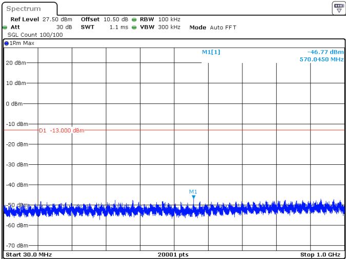
15MHz_15kHz_3972.5MHz_DFT-s-OFDM QPSK_RB1@0 -46.77 dBm
