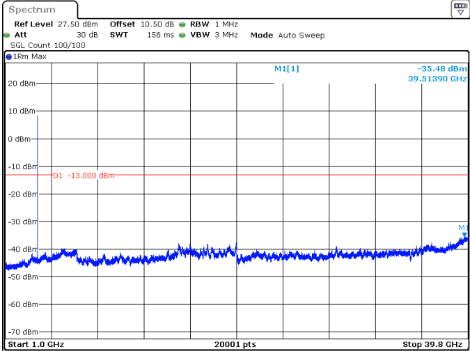
15MHz_30kHz_3707.5MHz_DFT-s-OFDM QPSK_RB1@37 -35.48 dBm
