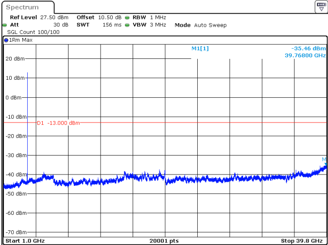
15MHz_15kHz_3840MHz_DFT-s-OFDM QPSK_RB1@0 -35.46 dBm
