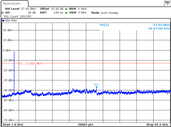
60MHz_30kHz_3500MHz_DFT-s-OFDM QPSK_RB162@0 -37.84 dBm
