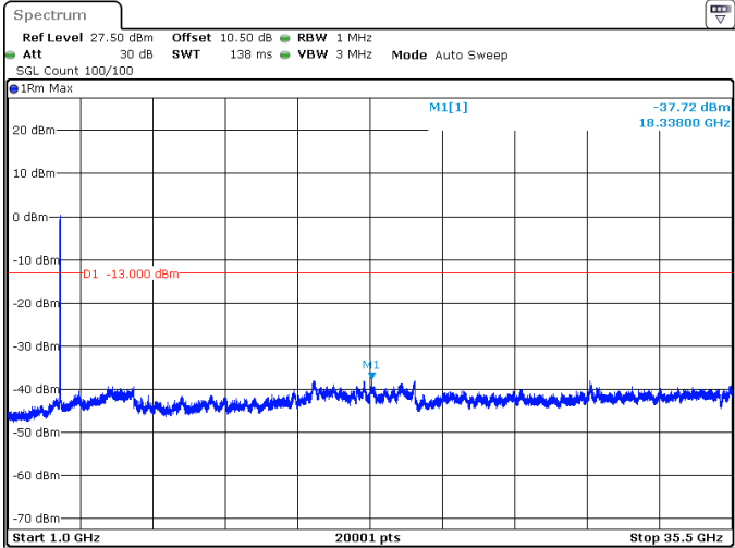
50MHz_30kHz_3475MHz_DFT-s-OFDM QPSK_RB128@0 -37.72 dBm
