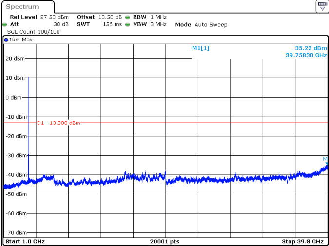
10MHz_15kHz_3975MHz_DFT-s-OFDM QPSK_RB1@51 -35.22 dBm
