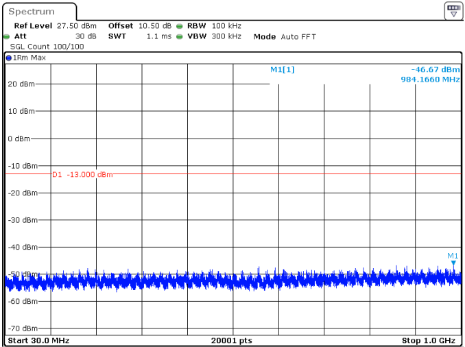
50MHz_30kHz_3525MHz_DFT-s-OFDM QPSK_RB128@0 -46.67 dBm
