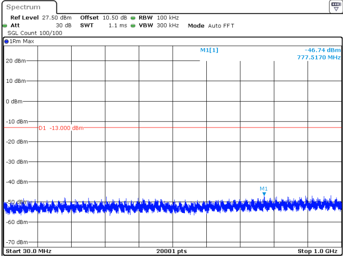
10MHz_30kHz_3840MHz_DFT-s-OFDM QPSK_RB1@23 -46.74 dBm
