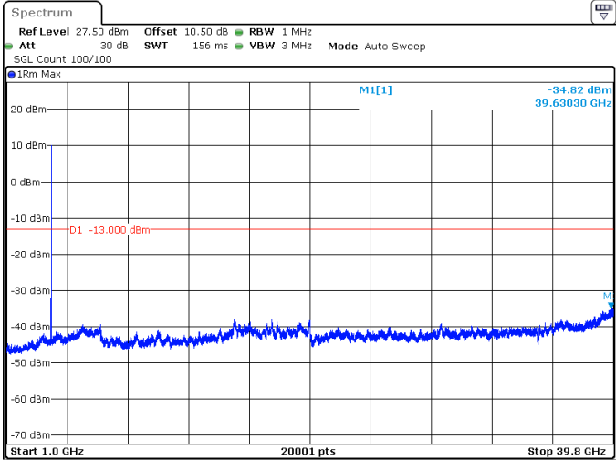
20MHz_15kHz_3840MHz_DFT-s-OFDM QPSK_RB1@105 -34.82 dBm
