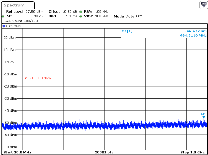
15MHz_15kHz_3707.5MHz_DFT-s-OFDM QPSK_RB1@0 -46.47 dBm
