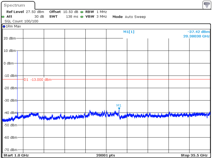
50MHz_30kHz_3525MHz_DFT-s-OFDM QPSK_RB1@0 -37.42 dBm
