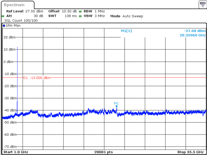
40MHz_30kHz_3500MHz_DFT-s-OFDM QPSK_RB1@105 -37.68 dBm
