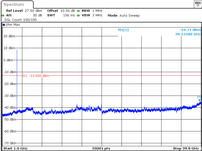
15MHz_30kHz_3840MHz_DFT-s-OFDM QPSK_RB1@0 -34.71 dBm
