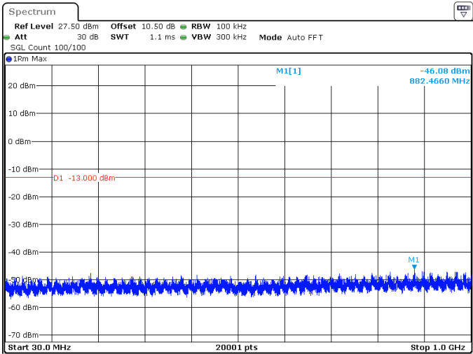
70MHz_30kHz_3515MHz_DFT-s-OFDM QPSK_RB180@0 -46.08 dBm
