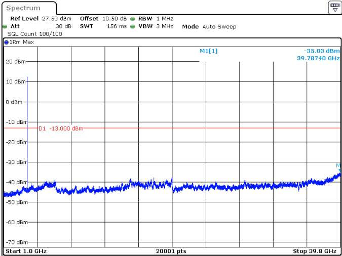
15MHz_15kHz_3707.5MHz_DFT-s-OFDM QPSK_RB1@78 -35.03 dBm
