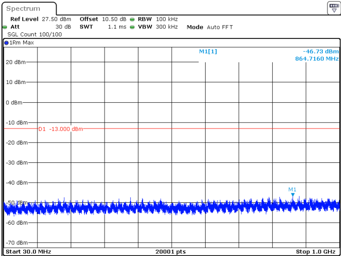
40MHz_30kHz_3500MHz_DFT-s-OFDM QPSK_RB1@0 -46.73 dBm
