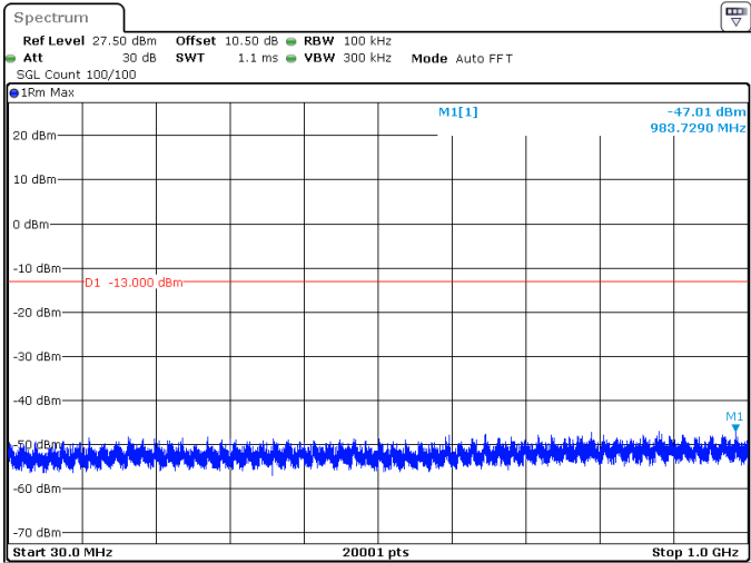
15MHz_15kHz_3972.5MHz_DFT-s-OFDM QPSK_RB1@78 -47.01 dBm
