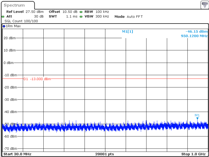
40MHz_30kHz_3500MHz_DFT-s-OFDM QPSK_RB100@0 -46.15 dBm
