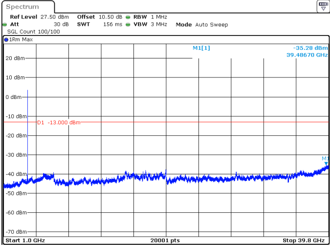
20MHz_15kHz_3840MHz_DFT-s-OFDM QPSK_RB100@0 -35.28 dBm
