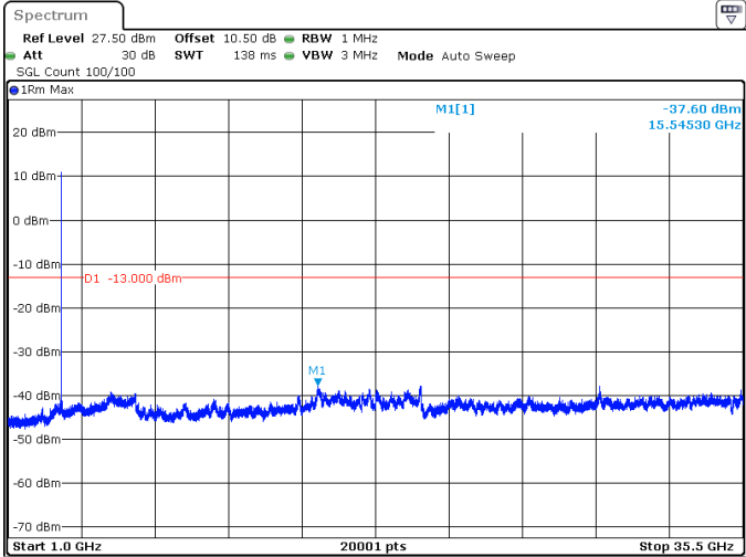
50MHz_30kHz_3475MHz_DFT-s-OFDM QPSK_RB1@132 -37.60 dBm
