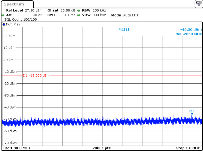
15MHz_15kHz_3840MHz_DFT-s-OFDM QPSK_RB1@78 -46.50 dBm
