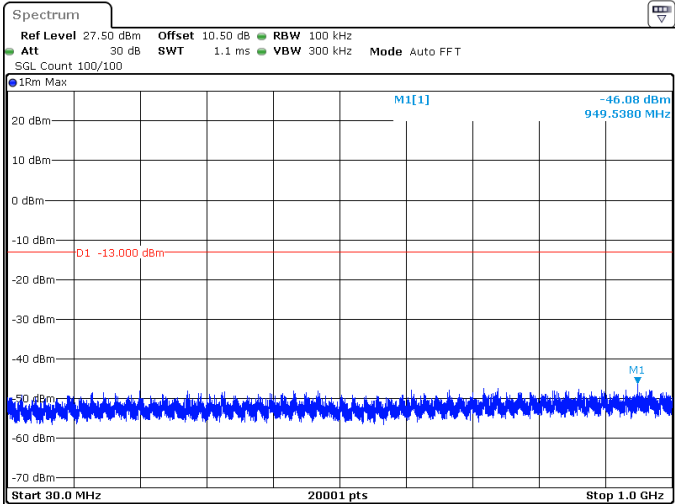
50MHz_30kHz_3475MHz_DFT-s-OFDM QPSK_RB1@0 -46.08 dBm
