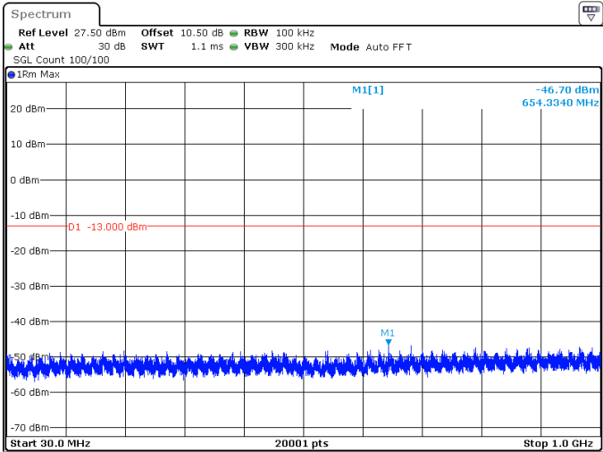
70MHz_30kHz_3500MHz_DFT-s-OFDM QPSK_RB1@188 -46.70 dBm
