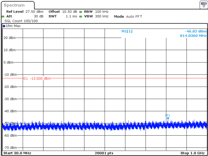
15MHz_15kHz_3707.5MHz_DFT-s-OFDM QPSK_RB75@0 -46.82 dBm
