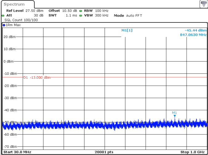
15MHz_30kHz_3840MHz_DFT-s-OFDM QPSK_RB1@37 -45.44 dBm
