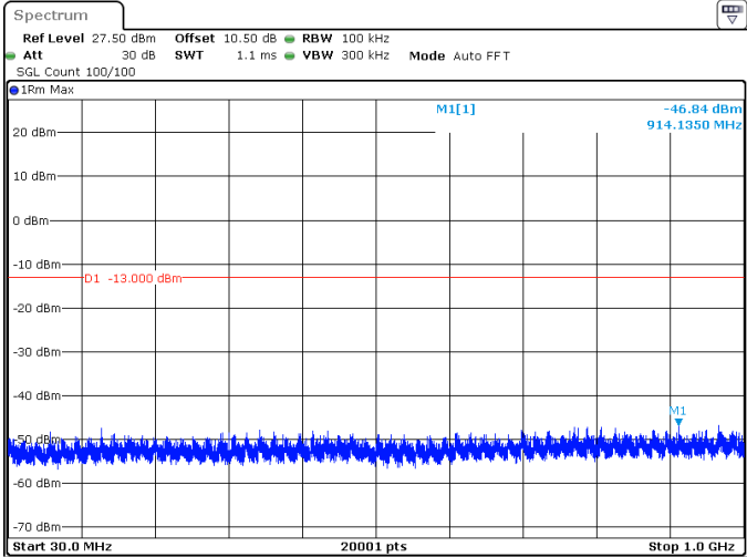
15MHz_30kHz_3707.5MHz_DFT-s-OFDM QPSK_RB36@0 -46.84 dBm
