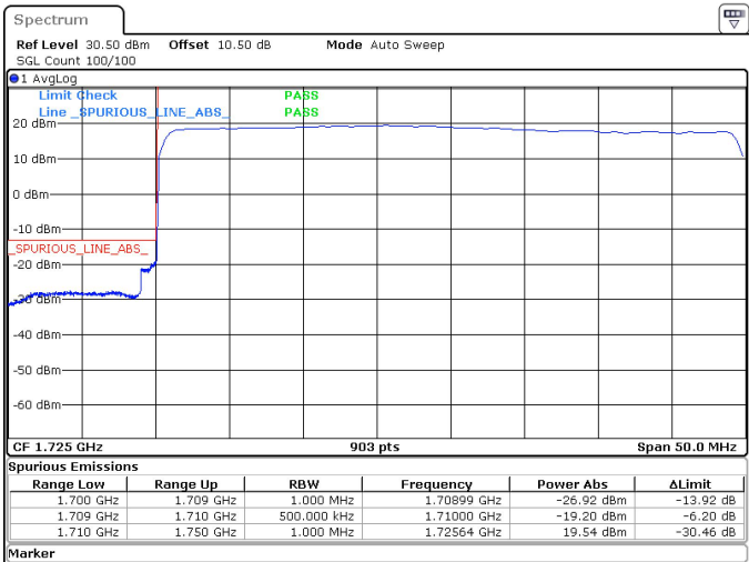
40MHz_15kHz_1730MHz_DFT-s-OFDM QPSK_RB216@0 -19.20 dBm
