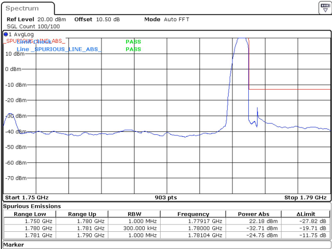
30MHz_15kHz_1765MHz_DFT-s-OFDM QPSK_RB1@159 -24.75 dBm
