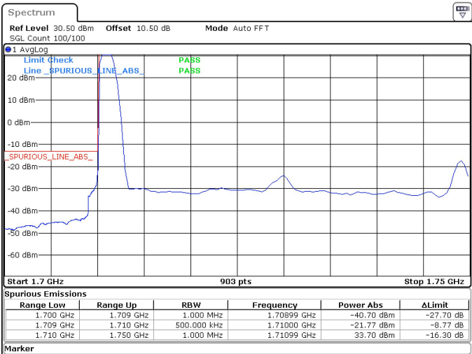
40MHz_15kHz_1730MHz_DFT-s-OFDM QPSK_RB1@0 -21.77 dBm
