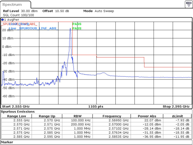
15MHz_15kHz_2562.5MHz_DFT-s-OFDM QPSK_RB1@78 -12.05 dBm
