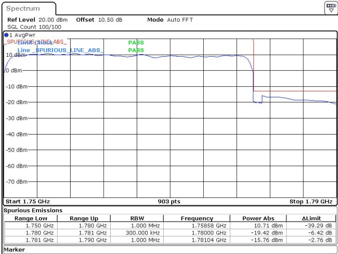
30MHz_15kHz_1765MHz_DFT-s-OFDM QPSK_RB160@0 -15.76 dBm
