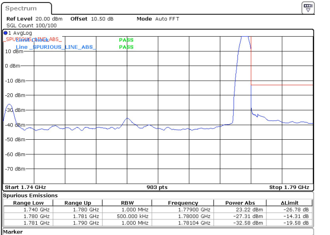
40MHz_15kHz_1760MHz_DFT-s-OFDM QPSK_RB1@215 -27.31 dBm
