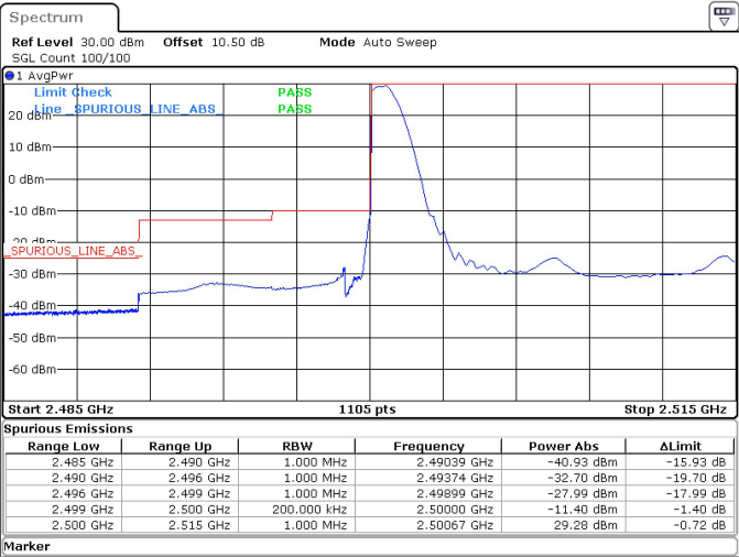
15MHz_15kHz_2507.5MHz_DFT-s-OFDM QPSK_RB1@0 29.28 dBm
