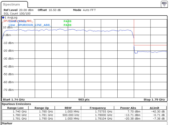
40MHz_15kHz_1760MHz_DFT-s-OFDM QPSK_RB216@0 -13.71 dBm
