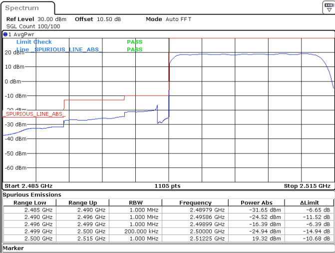
15MHz_15kHz_2507.5MHz_DFT-s-OFDM QPSK_RB75@0 -16.39 dBm
