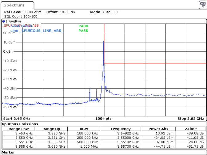
15MHz_30kHz_3542.5MHz_DFT-s-OFDM QPSK_RB1@37 -24.05 dBm
