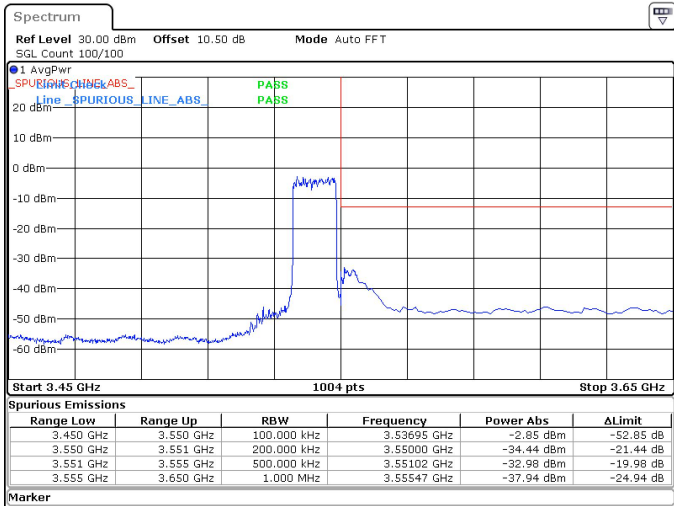
15MHz_30kHz_3542.5MHz_DFT-s-OFDM QPSK_RB36@0 -32.98 dBm
