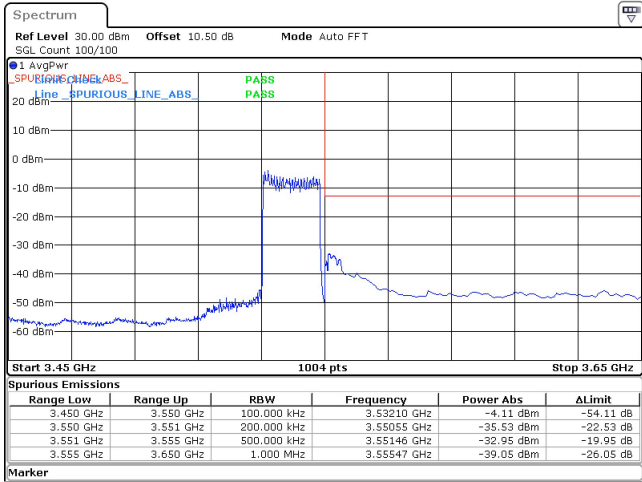
20MHz_15kHz_3540MHz_DFT-s-OFDM QPSK_RB100@0 -32.95 dBm
