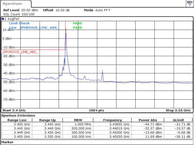
30MHz_15kHz_3465MHz_DFT-s-OFDM QPSK_RB1@0 -13.68 dBm
