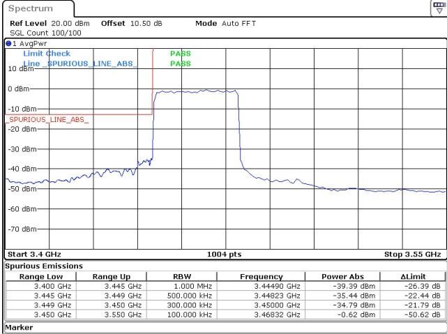
30MHz_15kHz_3465MHz_DFT-s-OFDM QPSK_RB160@0 -34.79 dBm
