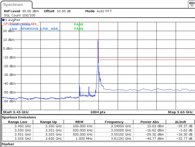
20MHz_15kHz_3540MHz_DFT-s-OFDM QPSK_RB1@105 -16.62 dBm
