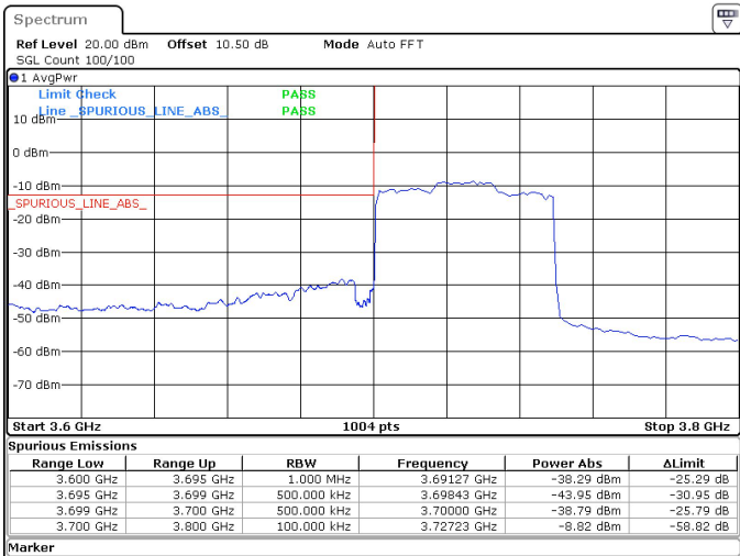
50MHz_15kHz_3725MHz_DFT-s-OFDM QPSK_RB270@0 -38.29 dBm
