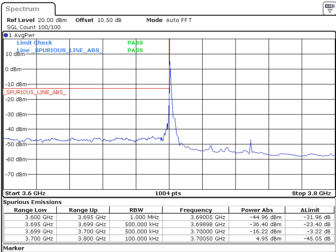
50MHz_15kHz_3725MHz_DFT-s-OFDM QPSK_RB1@0 -16.22 dBm
