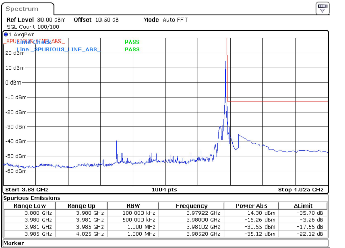
50MHz_15kHz_3955MHz_DFT-s-OFDM QPSK_RB1@269 -16.26 dBm
