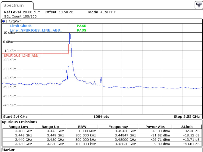
25MHz_30kHz_3462.5MHz_DFT-s-OFDM QPSK_RB1@0 -26.71 dBm
