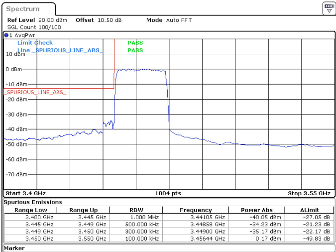
25MHz_30kHz_3462.5MHz_DFT-s-OFDM QPSK_RB64@0 -34.23 dBm
