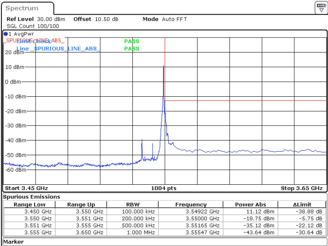
15MHz_30kHz_3542.5MHz_DFT-s-OFDM QPSK_RB1@37 -18.75 dBm
