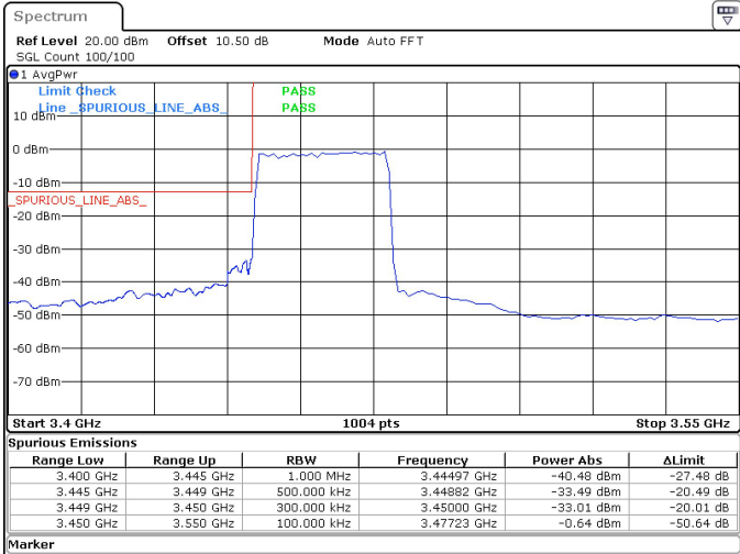
30MHz_30kHz_3465MHz_DFT-s-OFDM QPSK_RB75@0 -33.01 dBm
