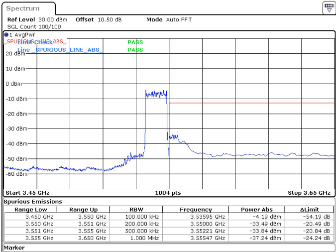
15MHz_30kHz_3542.5MHz_DFT-s-OFDM QPSK_RB36@0 -33.49 dBm
